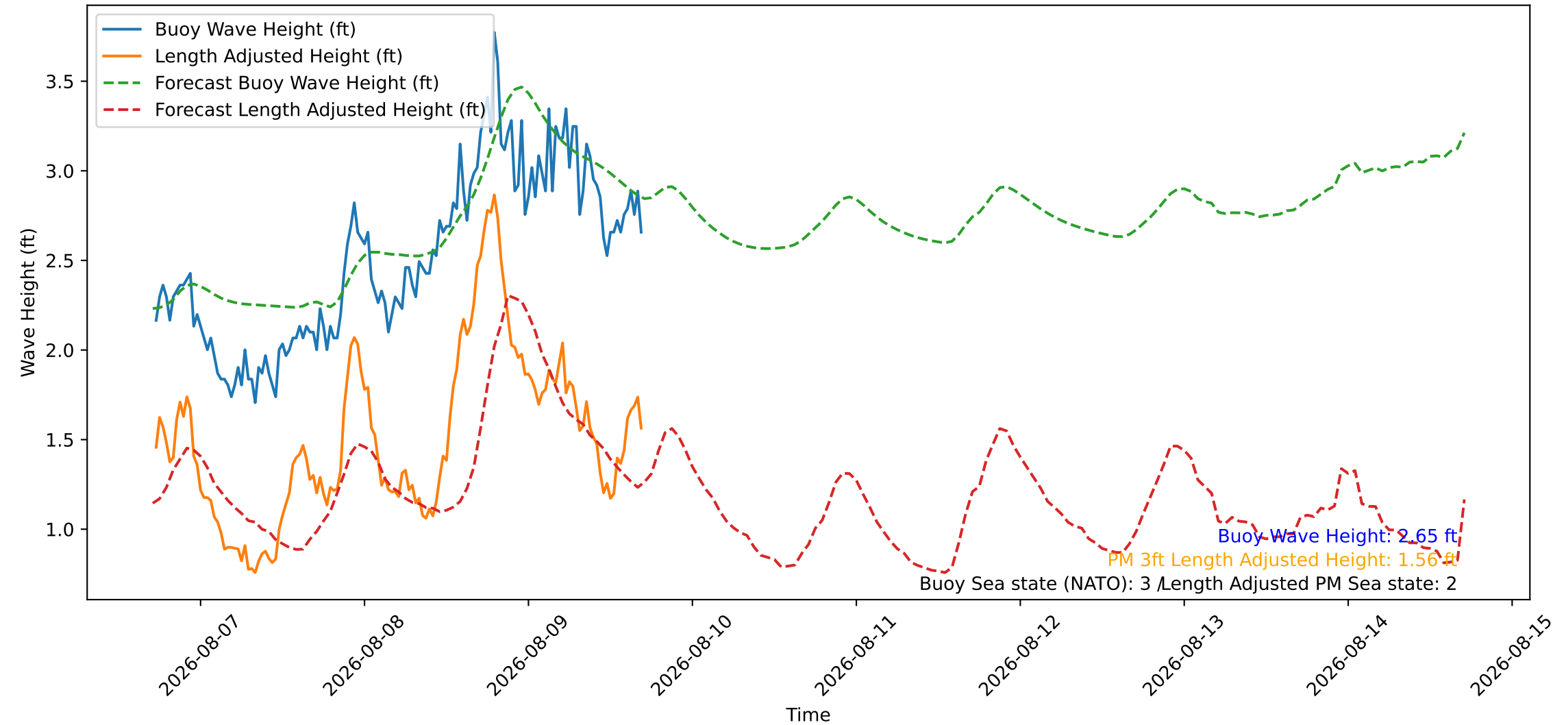
Wave Heights over Time for Green Beach at 2026-08-09 17:21:11
