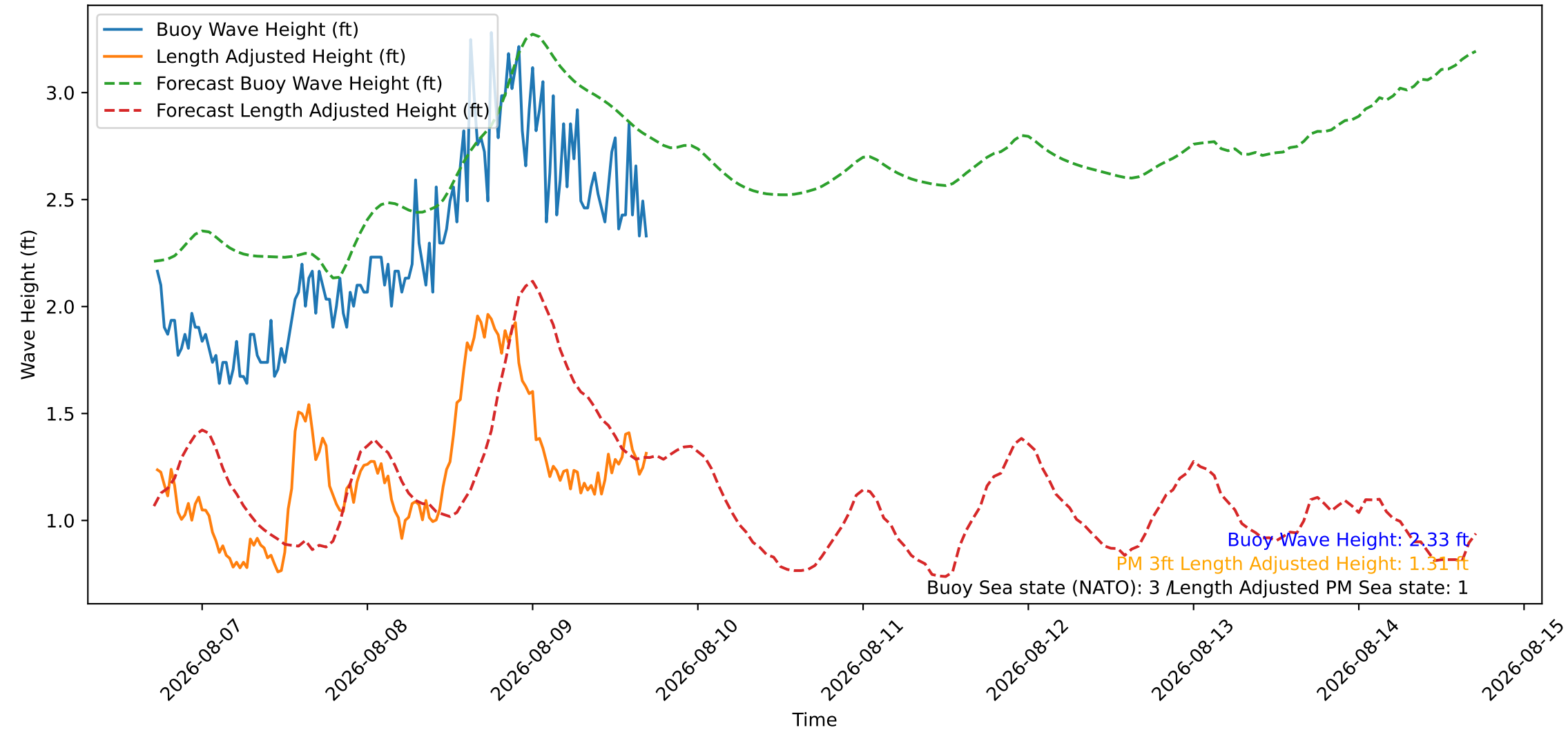
Wave Heights over Time for Oceanside Harbor at 2026-08-09 17:20:27
