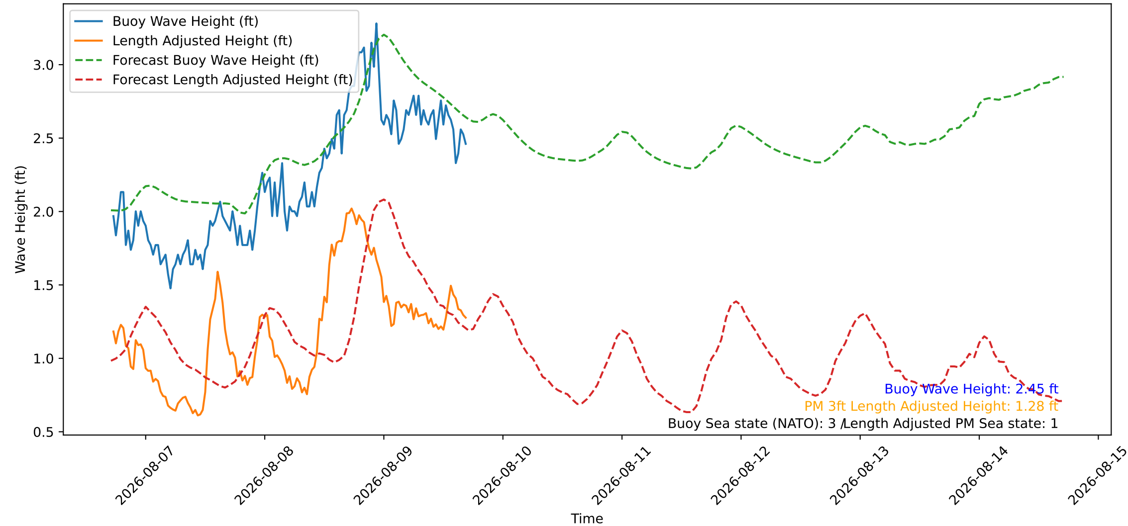
Wave Heights over Time for Red Beach at 2026-08-09 17:20:48
