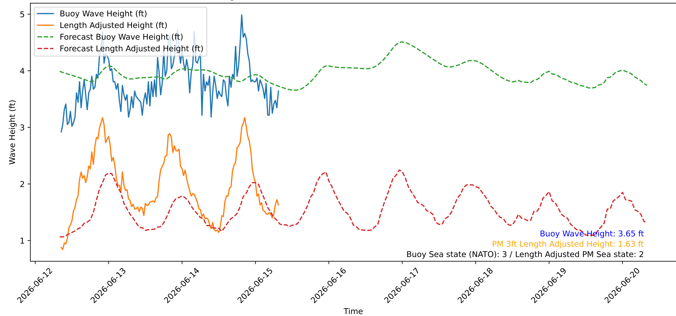
Wave Heights over Time for Oceanside Harbor at 2026-06-15 08:20:26
