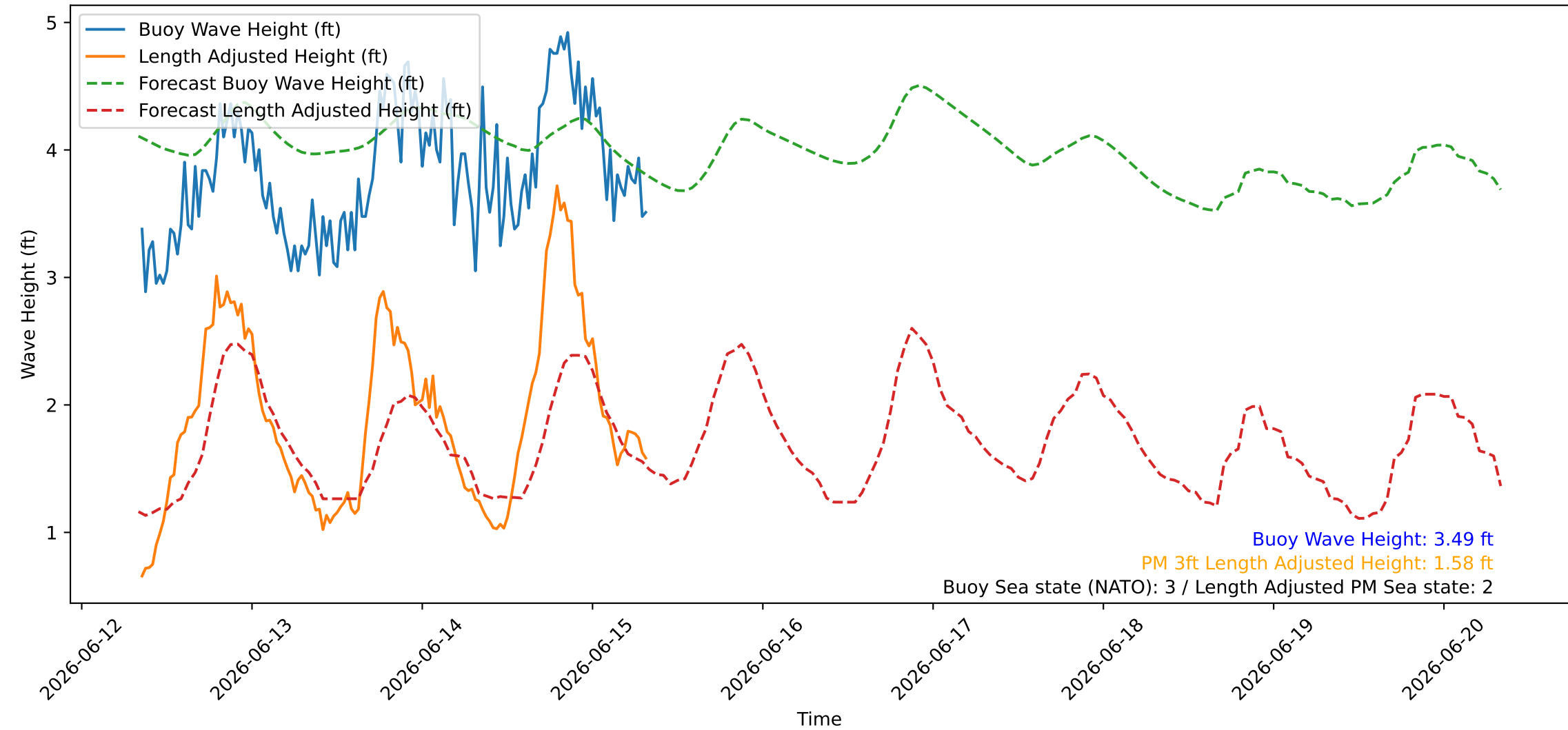
Wave Heights over Time for Green Beach at 2026-06-15 08:21:10
