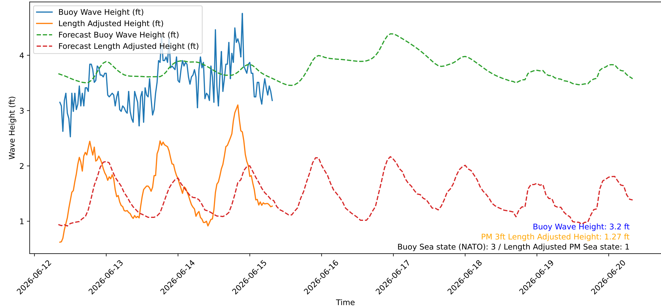
Wave Heights over Time for Red Beach at 2026-06-15 08:20:47
