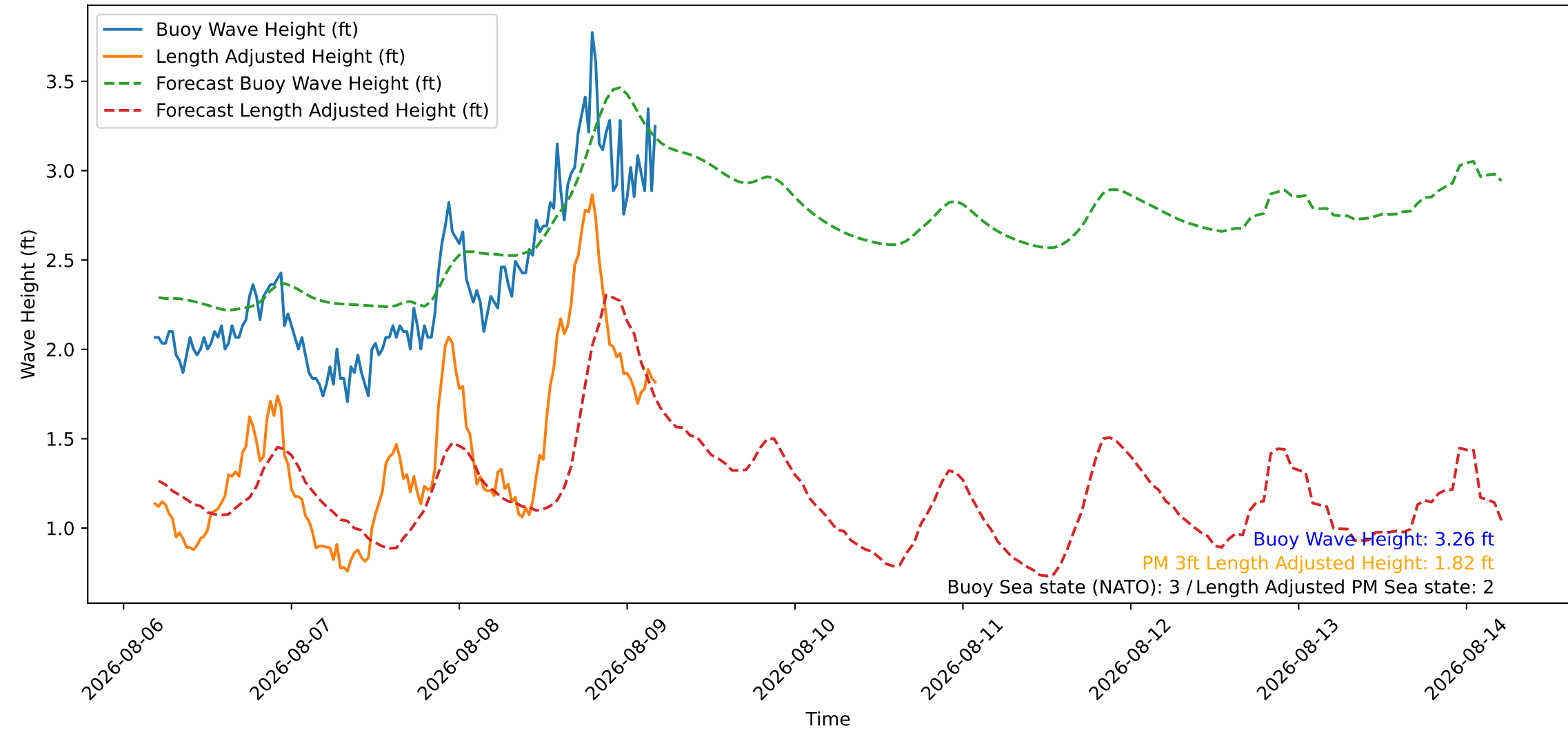
Wave Heights over Time for Green Beach at 2026-08-09 04:41:08
