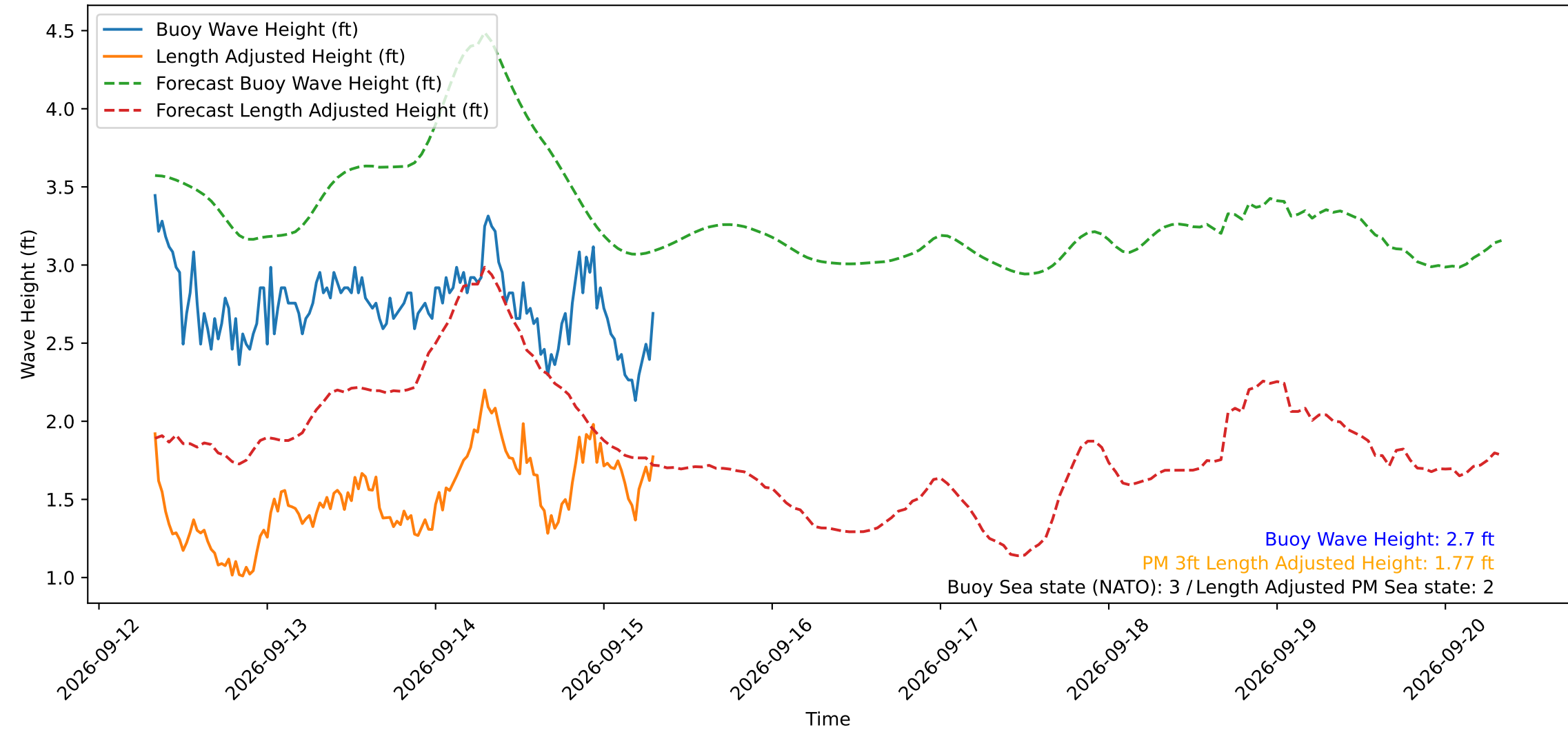
Wave Heights over Time for Green Beach at 2026-09-15 07:51:14
