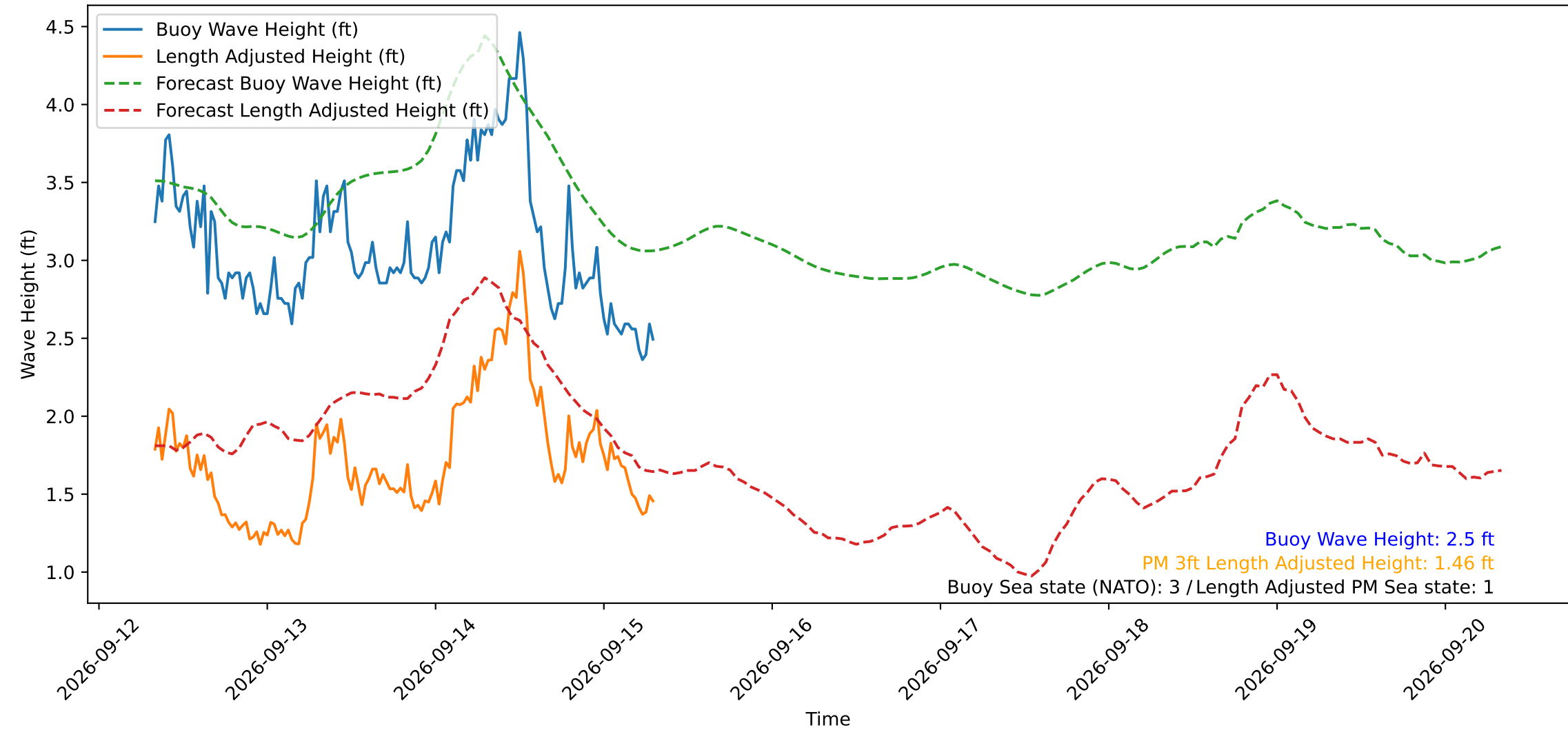
Wave Heights over Time for Oceanside Harbor at 2026-09-15 07:50:29
