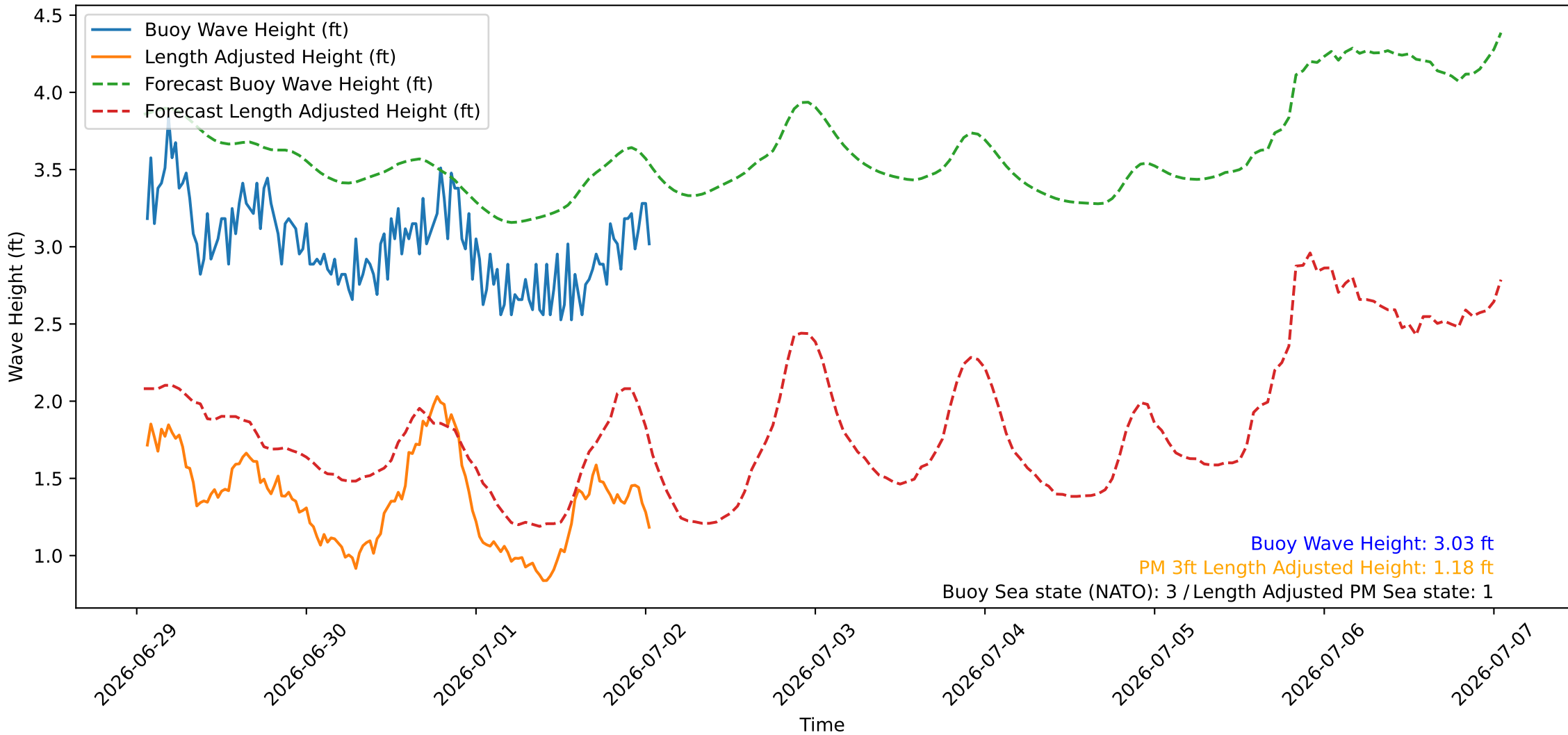
Wave Heights over Time for Green Beach at 2026-07-02 01:21:09
