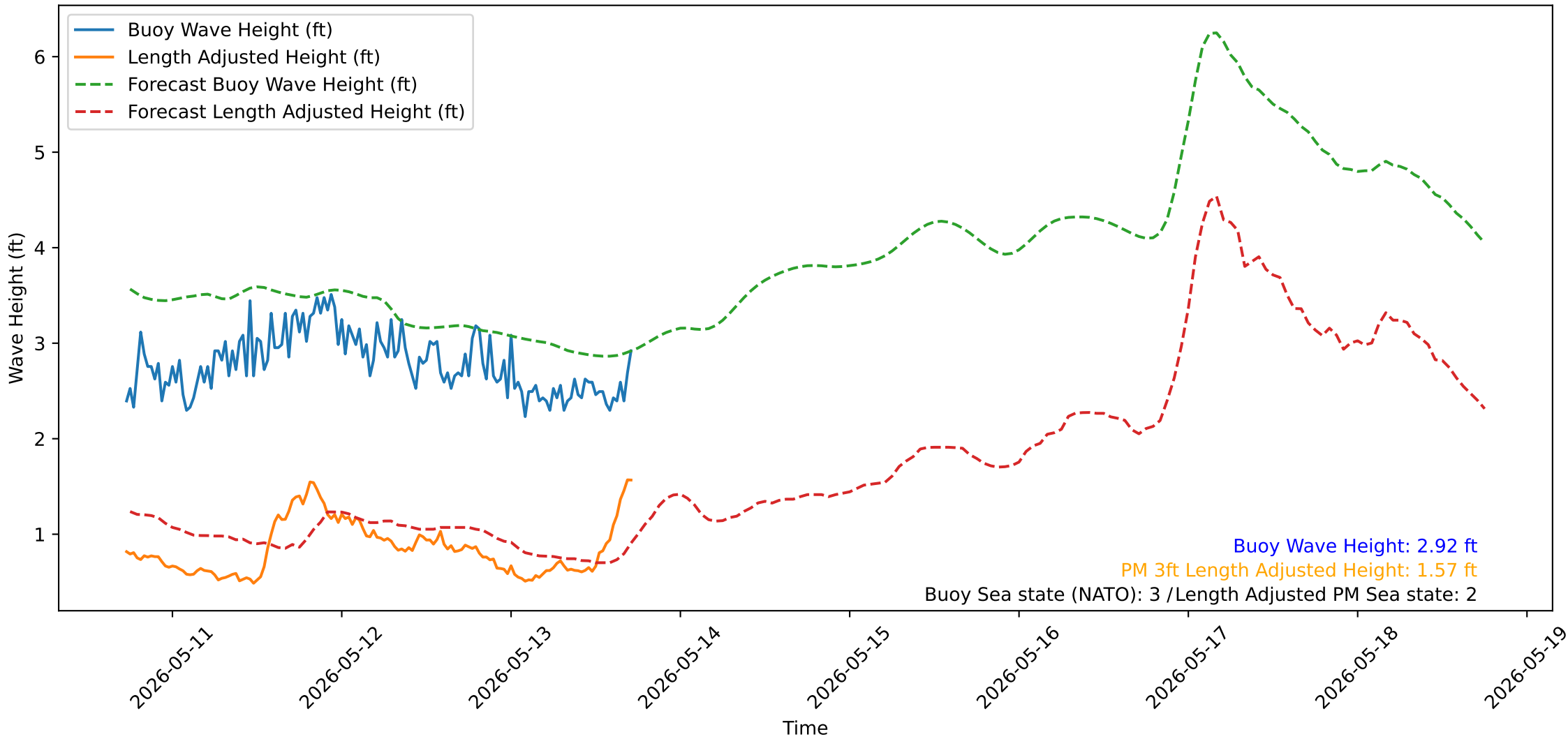
Wave Heights over Time for Green Beach at 2026-05-13 17:41:15
