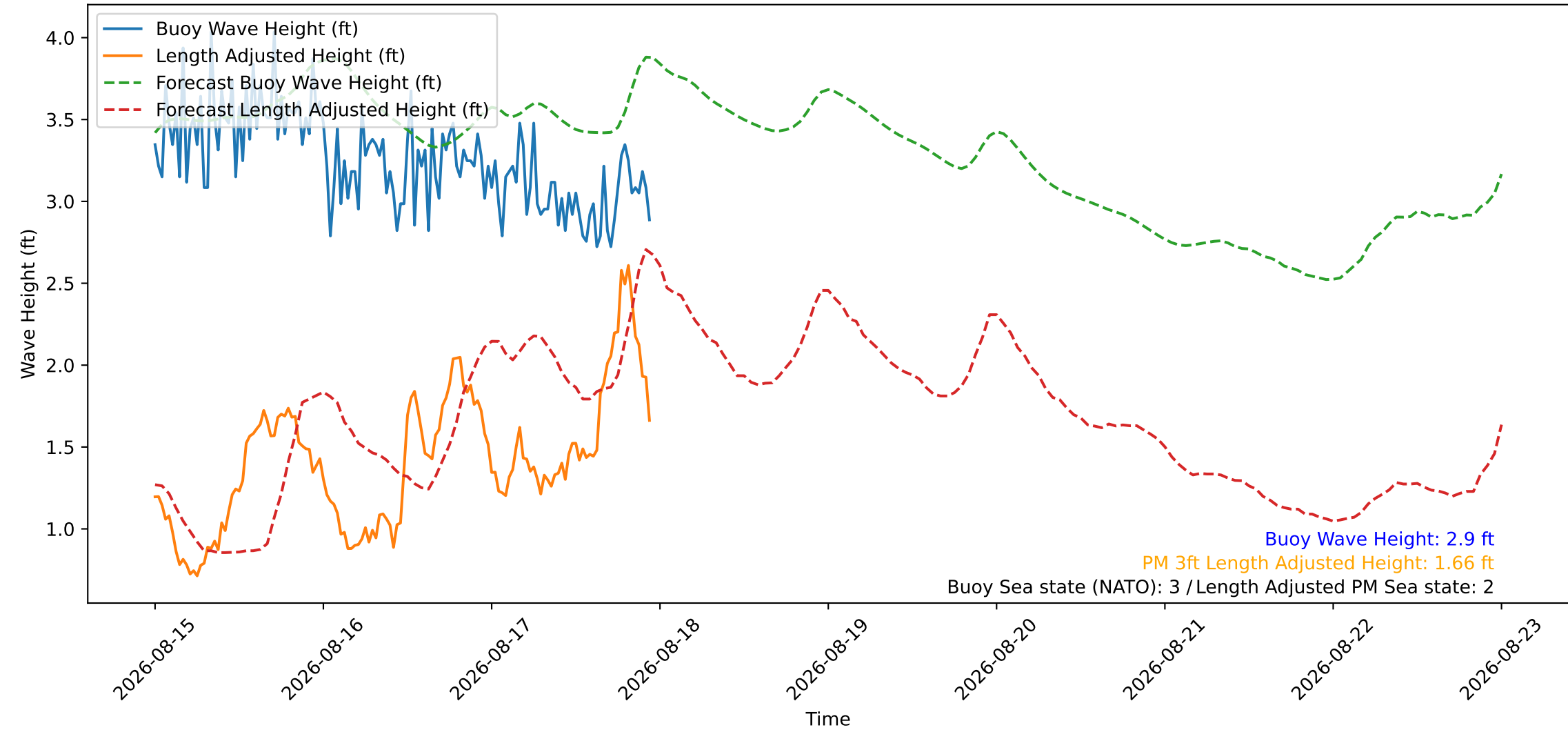
Wave Heights over Time for Red Beach at 2026-08-17 23:40:45
