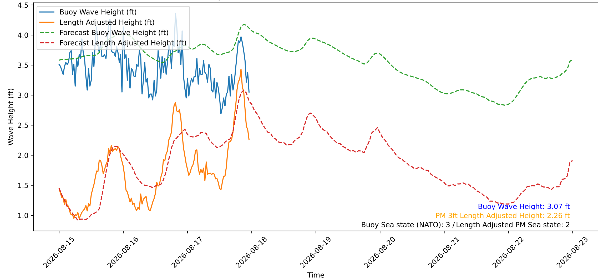
Wave Heights over Time for Green Beach at 2026-08-17 23:41:08
