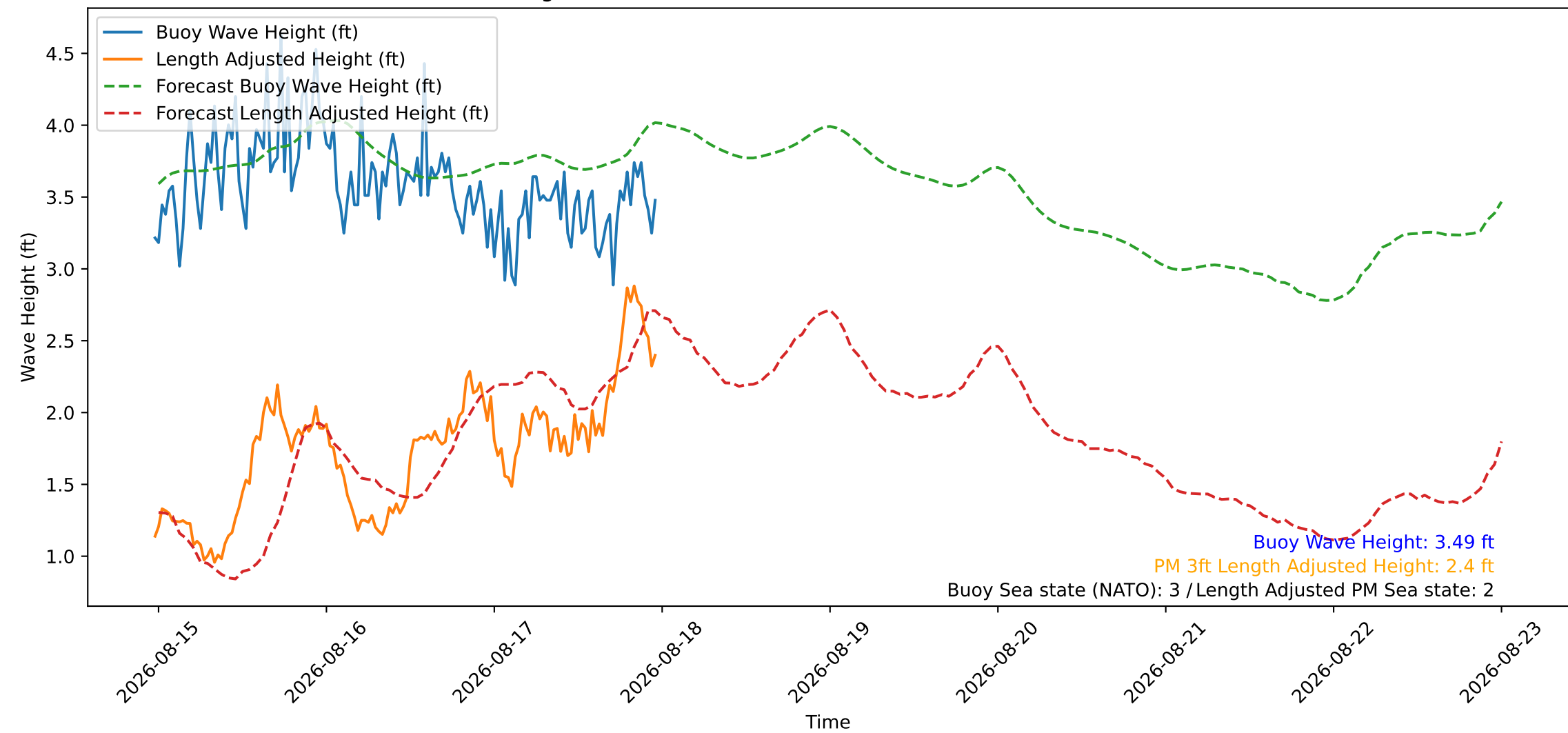
Wave Heights over Time for Oceanside Harbor at 2026-08-17 23:40:26
