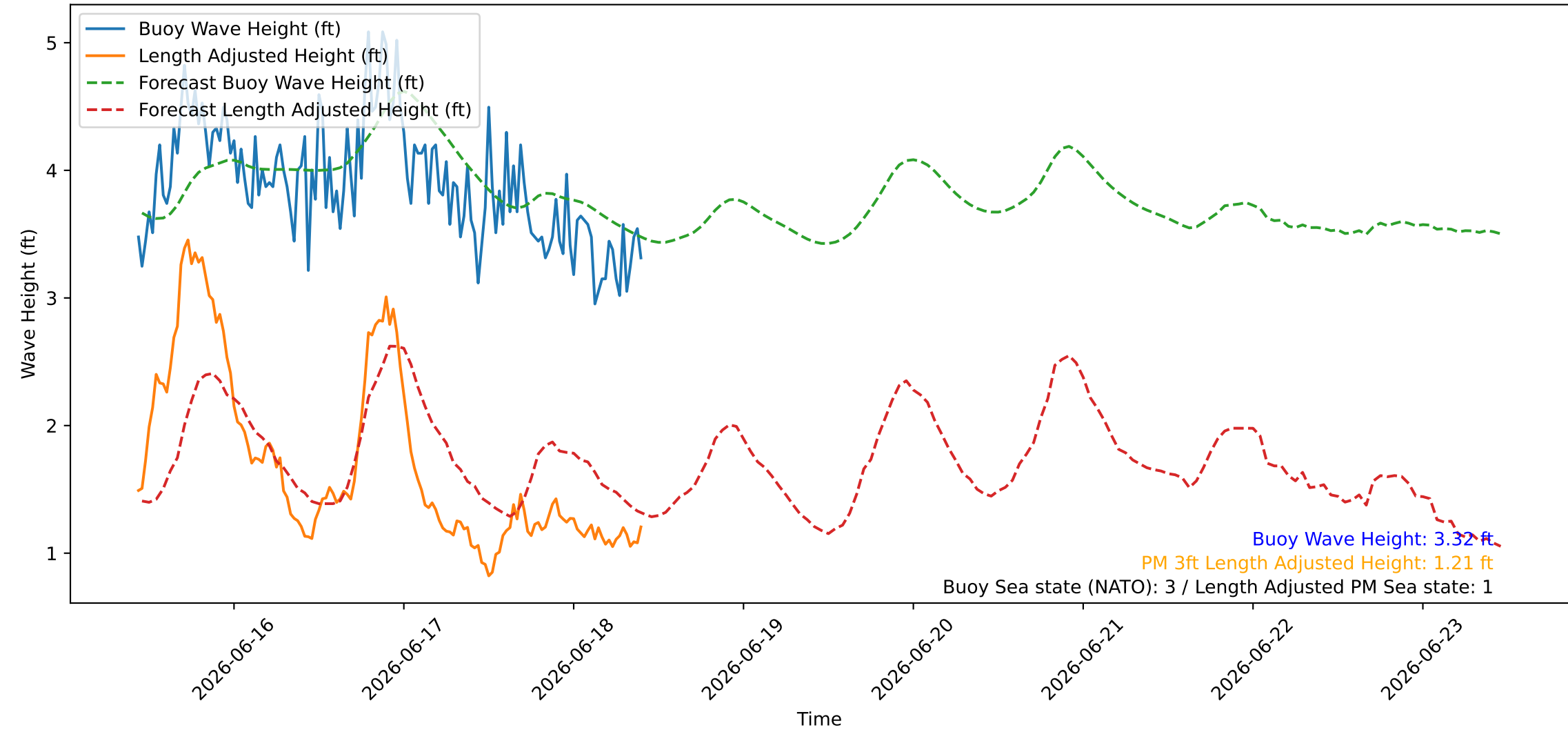
Wave Heights over Time for Green Beach at 2026-06-18 10:31:08
