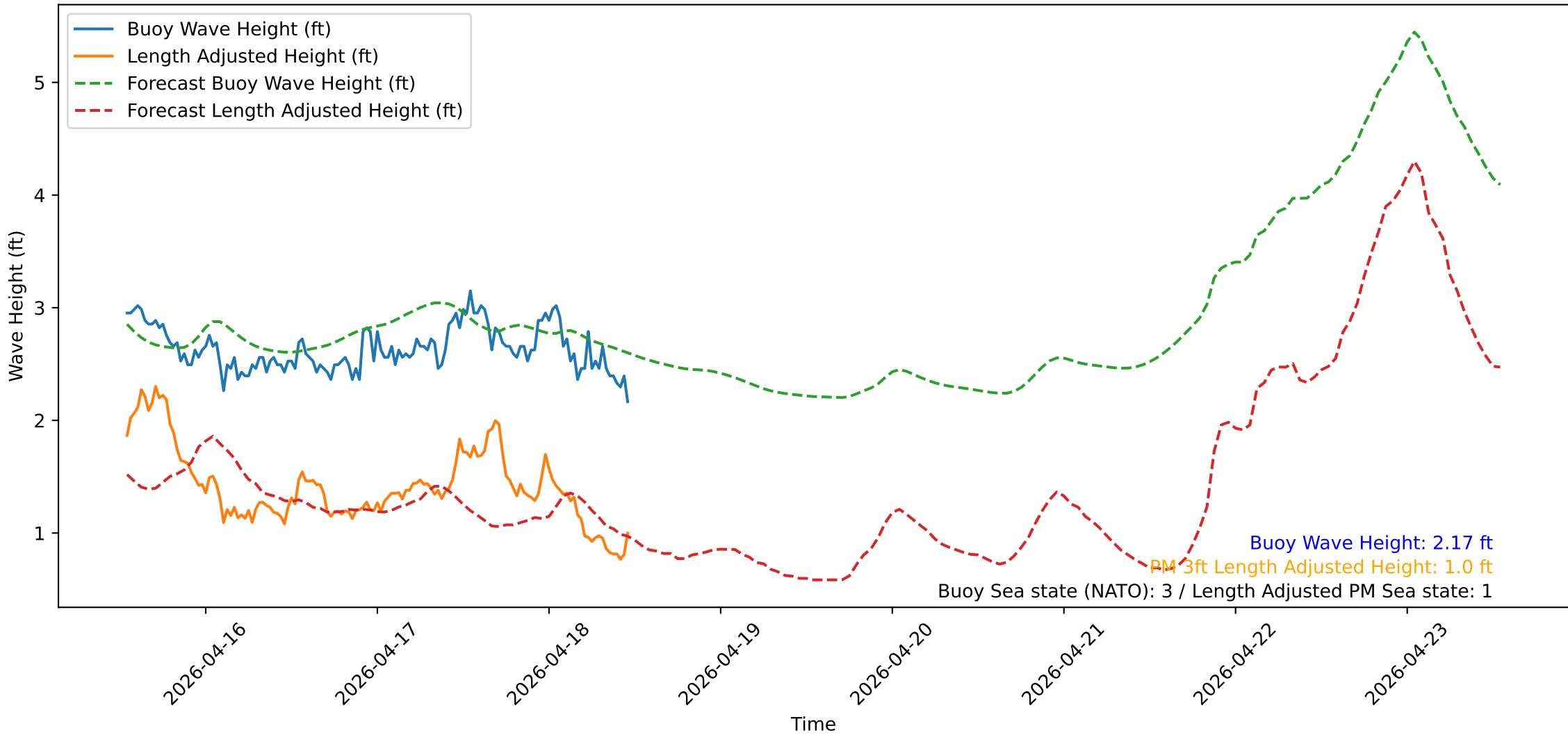
Wave Heights over Time for Red Beach at 2026-04-18 12:30:50
