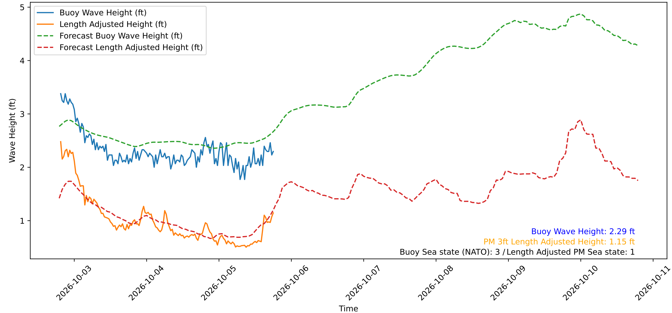
Wave Heights over Time for Green Beach at 2026-10-05 19:01:11
