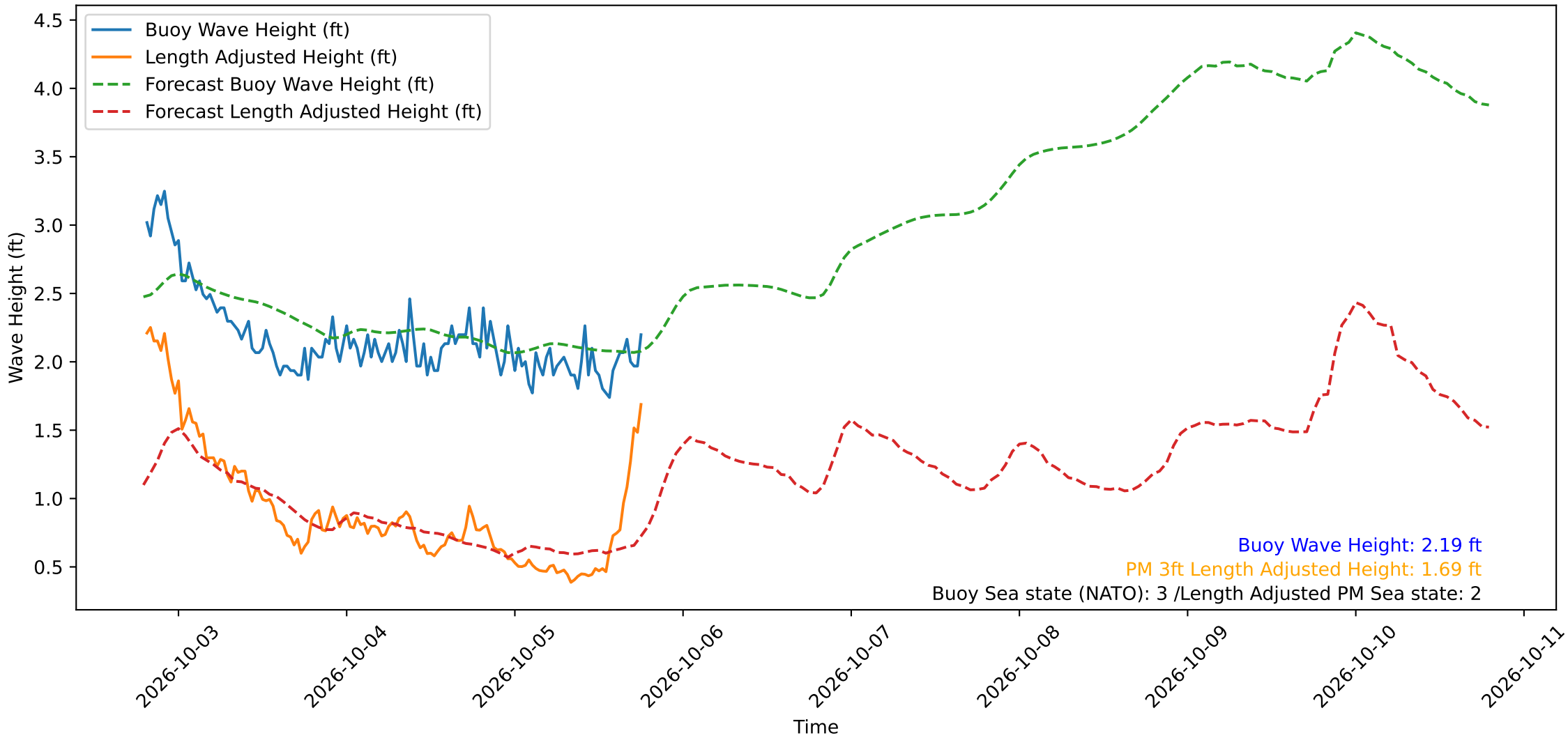
Wave Heights over Time for Red Beach at 2026-10-05 19:00:49
