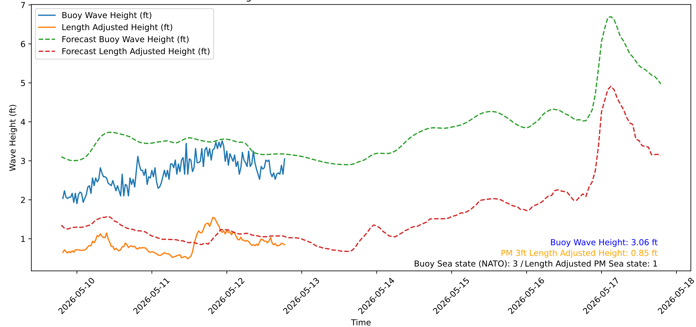
Wave Heights over Time for Green Beach at 2026-05-12 19:21:15
