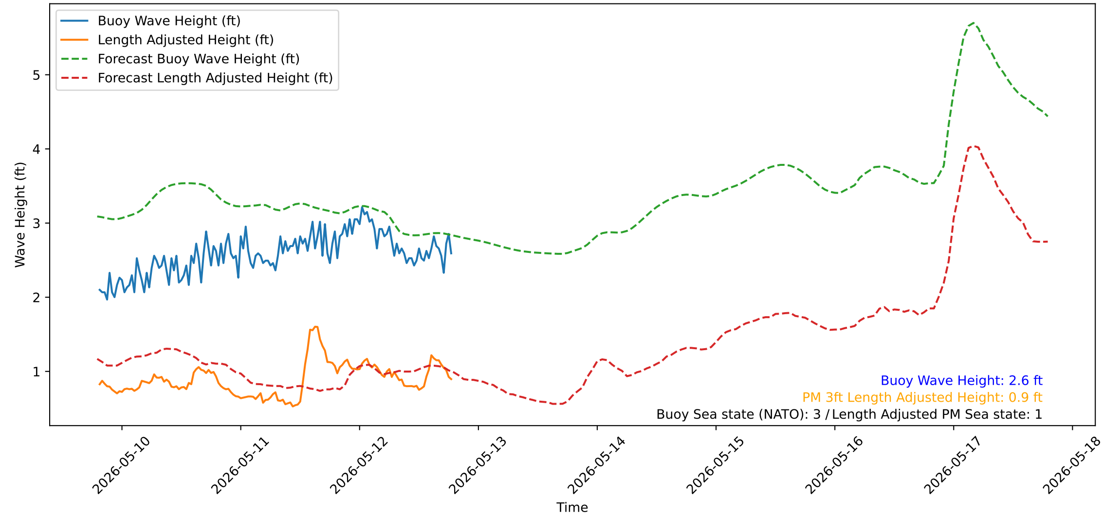
Wave Heights over Time for Red Beach at 2026-05-12 19:20:52
