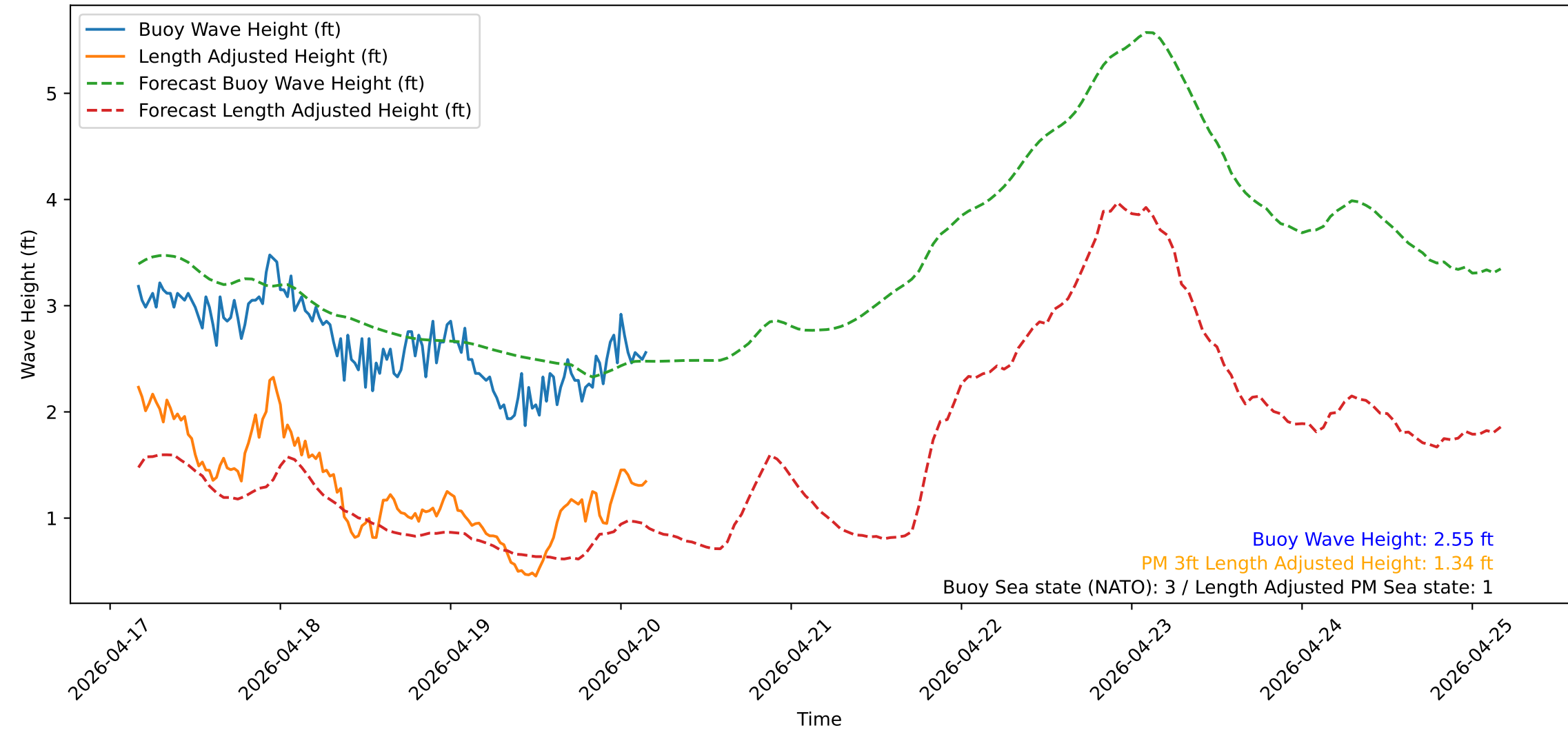
Wave Heights over Time for Green Beach at 2026-04-20 04:11:12
