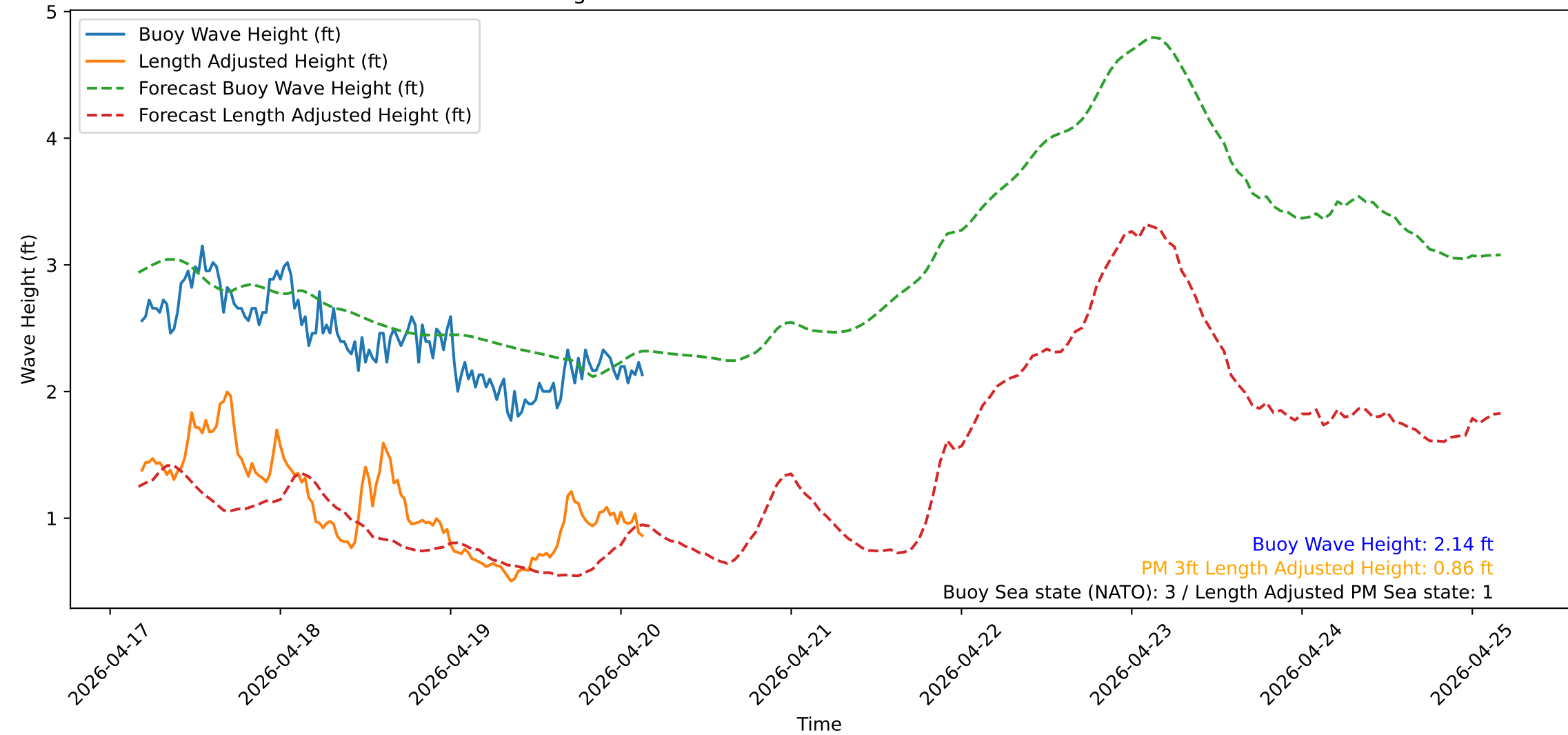
Wave Heights over Time for Red Beach at 2026-04-20 04:10:50
