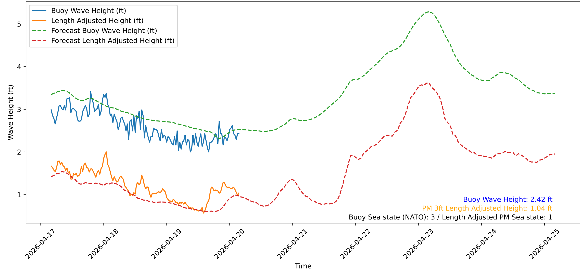
Wave Heights over Time for Oceanside Harbor at 2026-04-20 04:10:32
