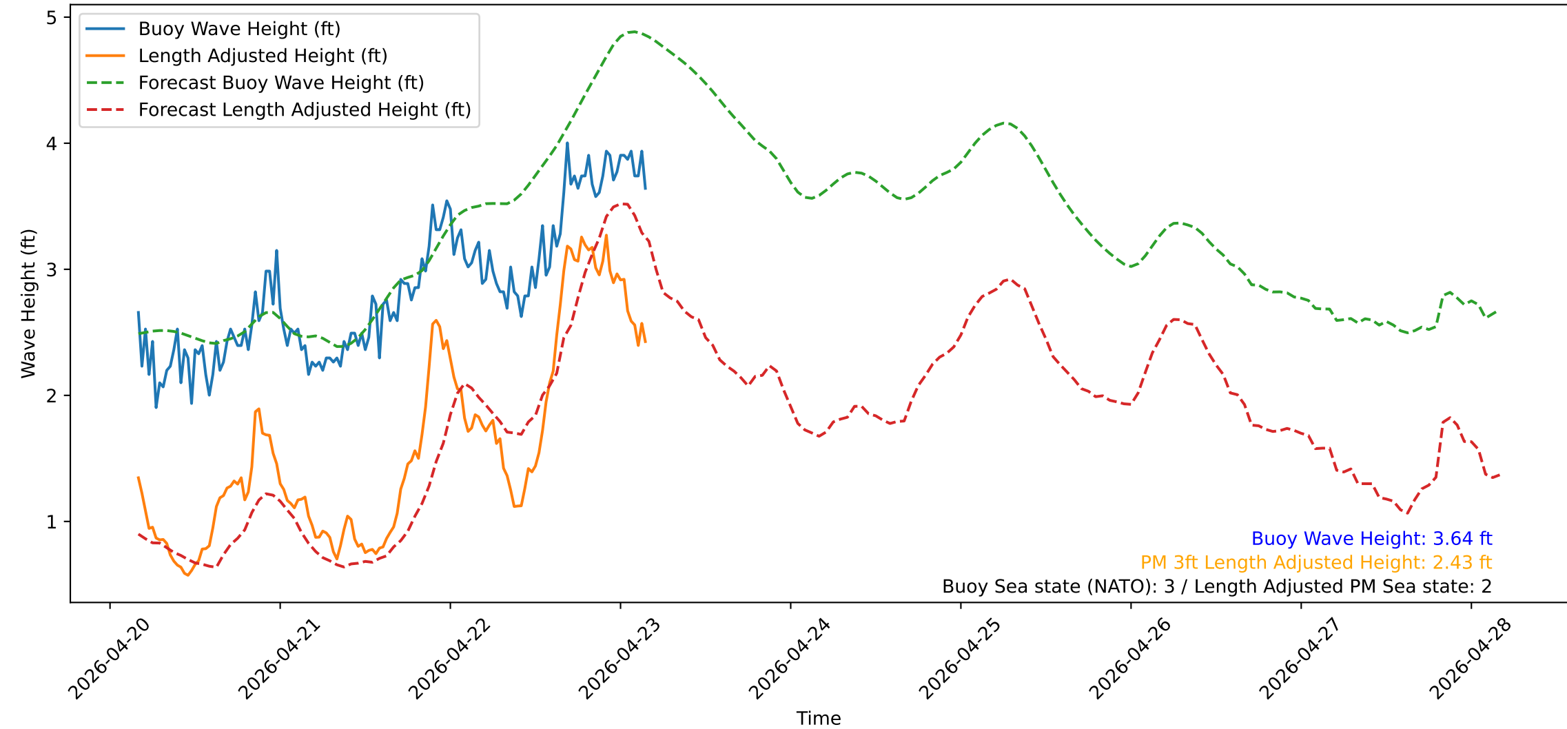
Wave Heights over Time for Green Beach at 2026-04-23 04:11:12
