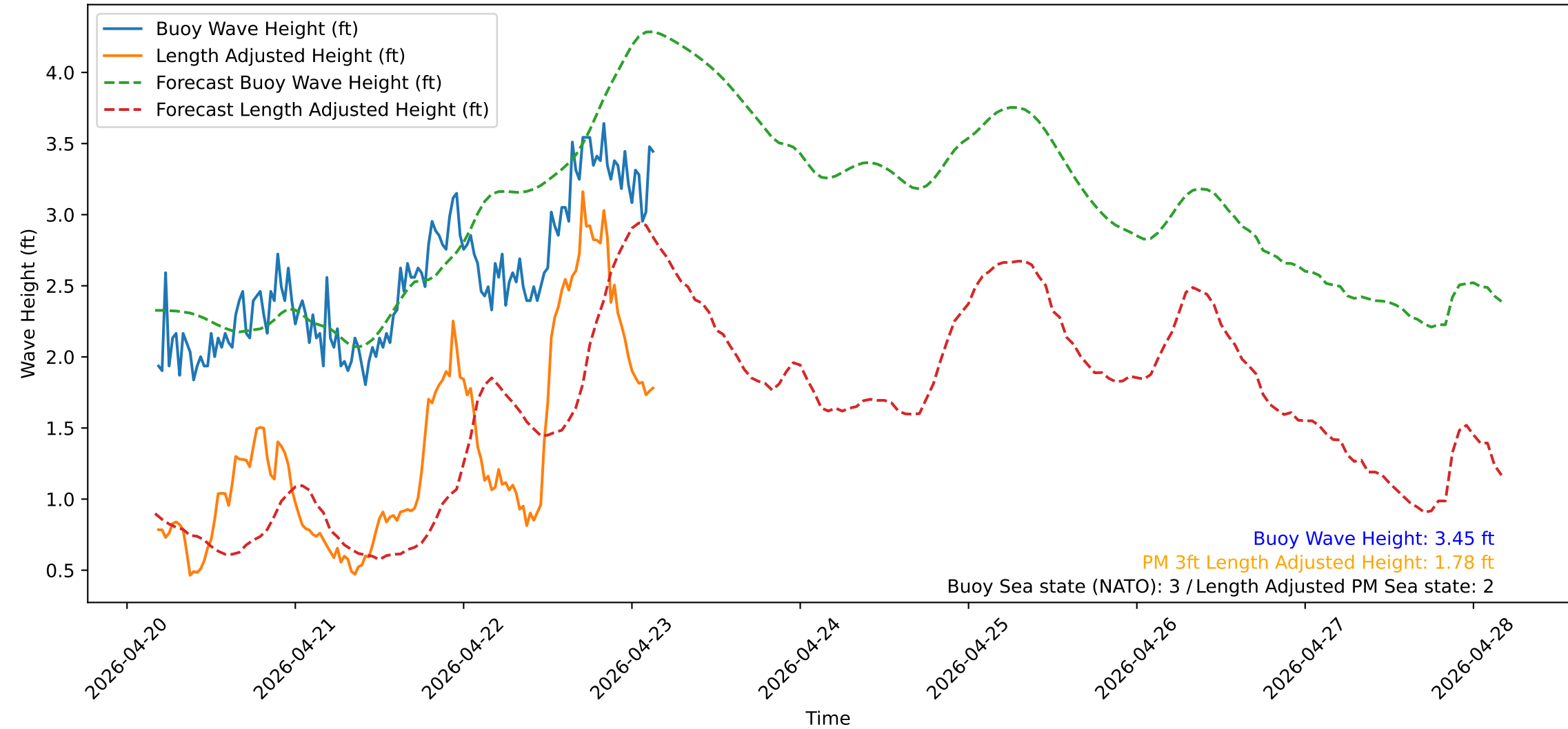
Wave Heights over Time for Red Beach at 2026-04-23 04:10:50
