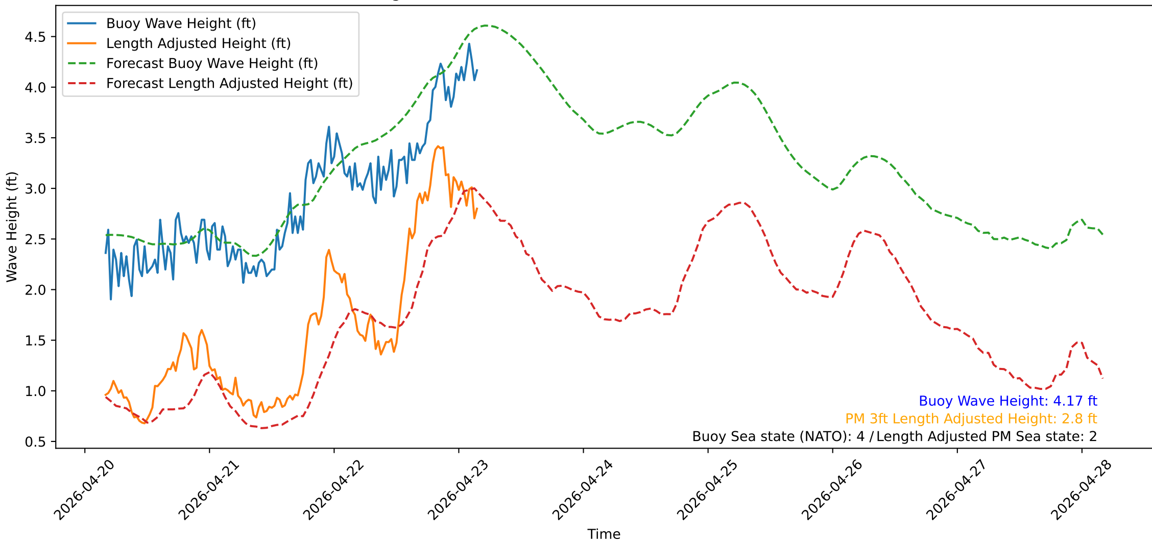
Wave Heights over Time for Oceanside Harbor at 2026-04-23 04:10:31
