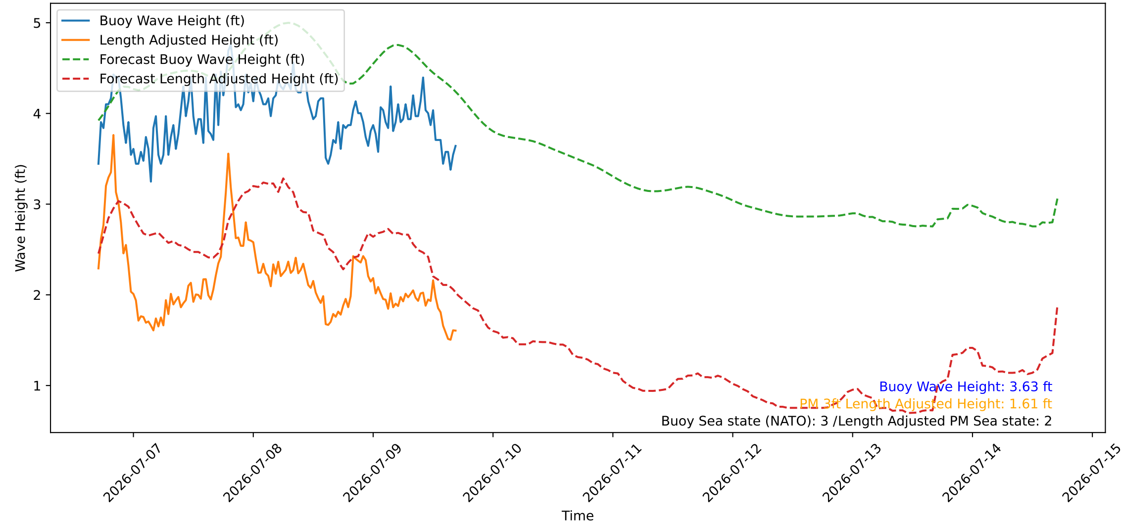
Wave Heights over Time for Green Beach at 2026-07-09 17:11:07
