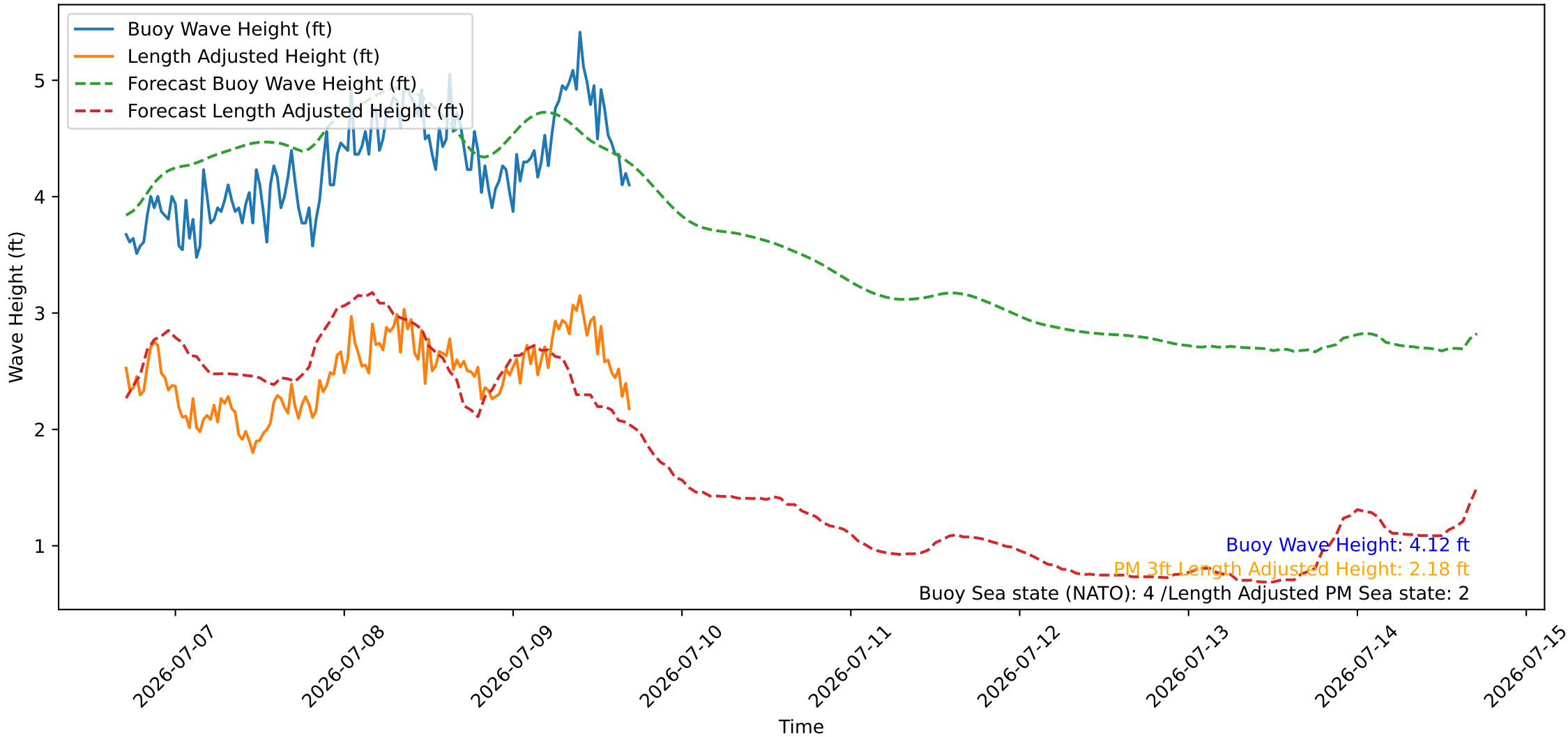
Wave Heights over Time for Oceanside Harbor at 2026-07-09 17:10:26
