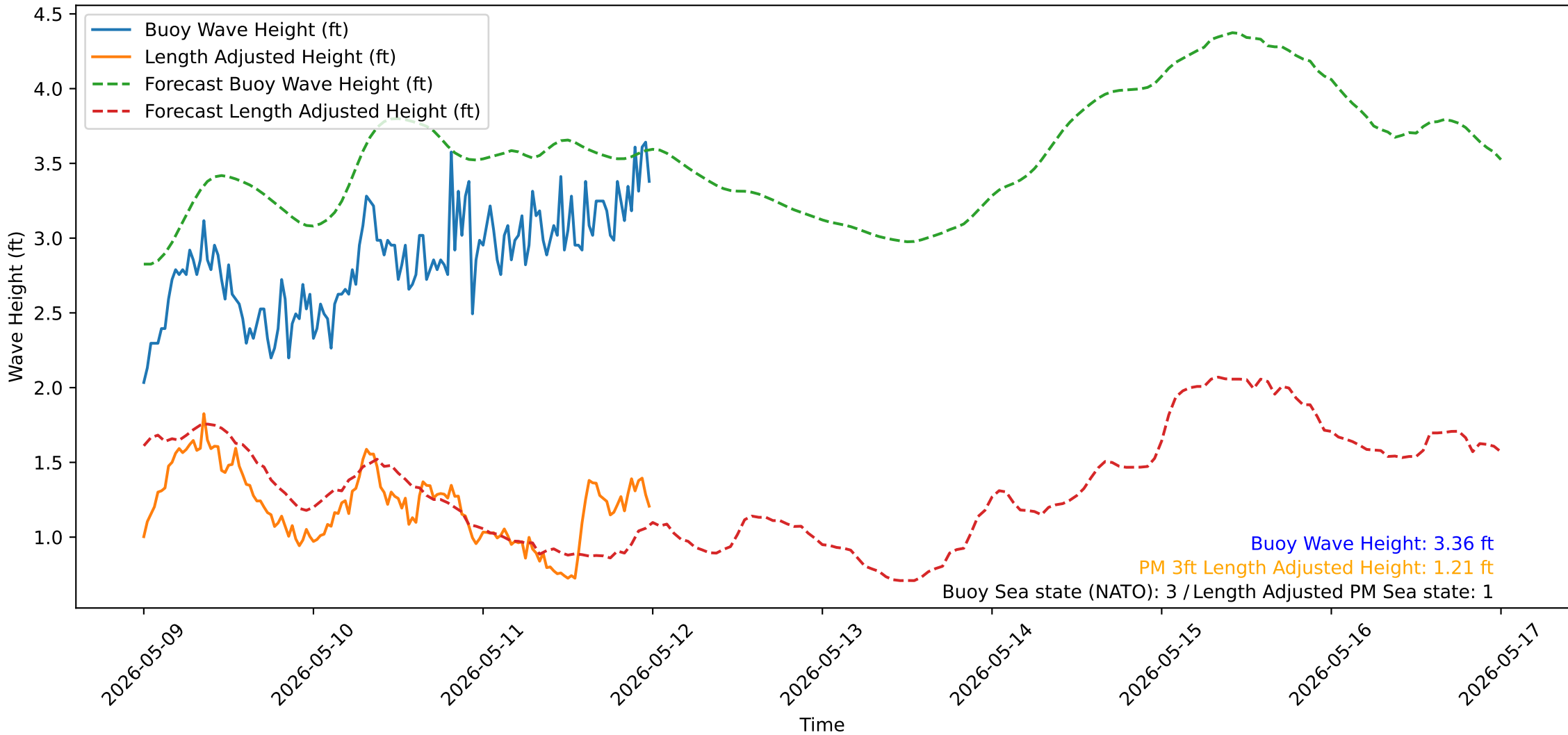
Wave Heights over Time for Oceanside Harbor at 2026-05-12 00:10:31
