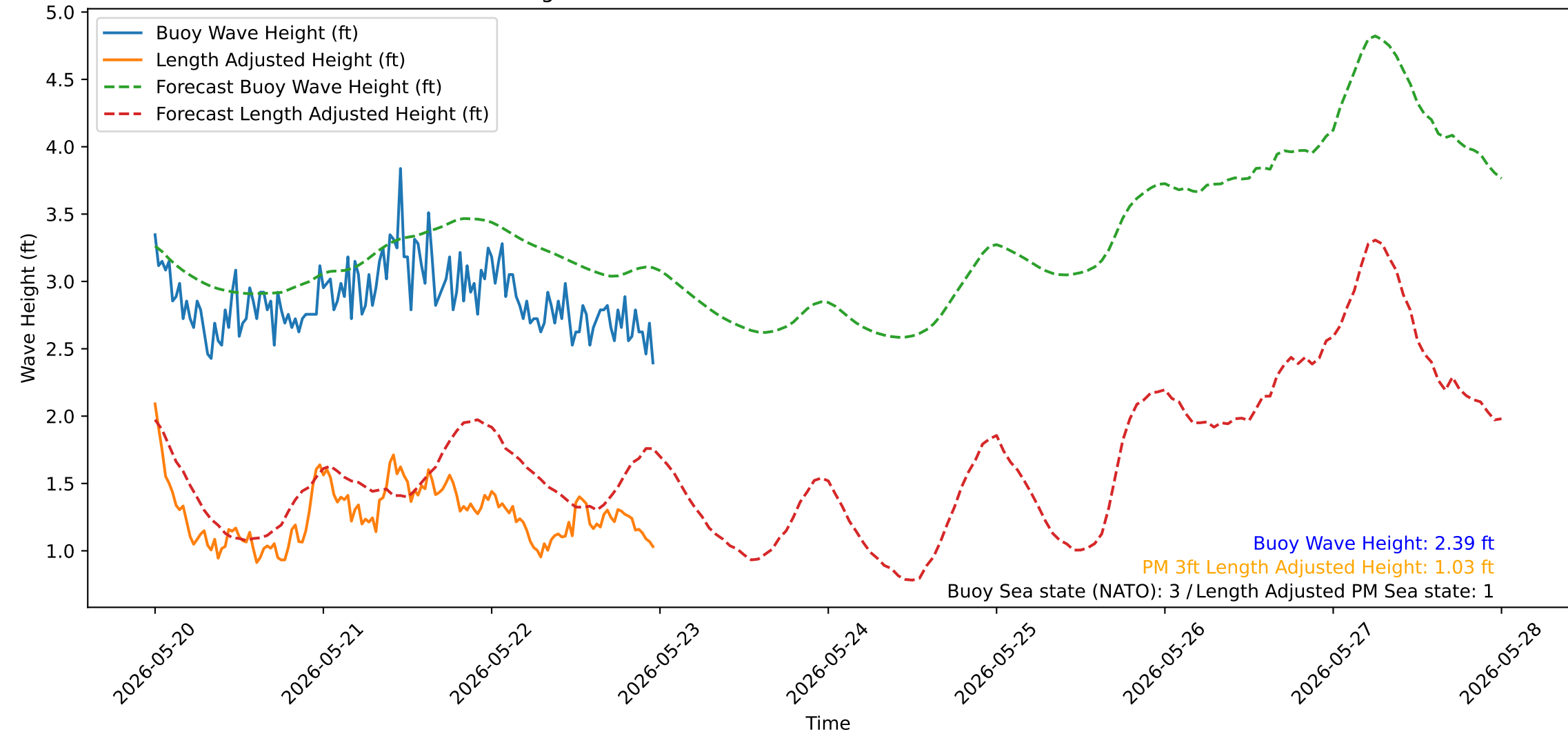
Wave Heights over Time for Oceanside Harbor at 2026-05-22 23:50:31
