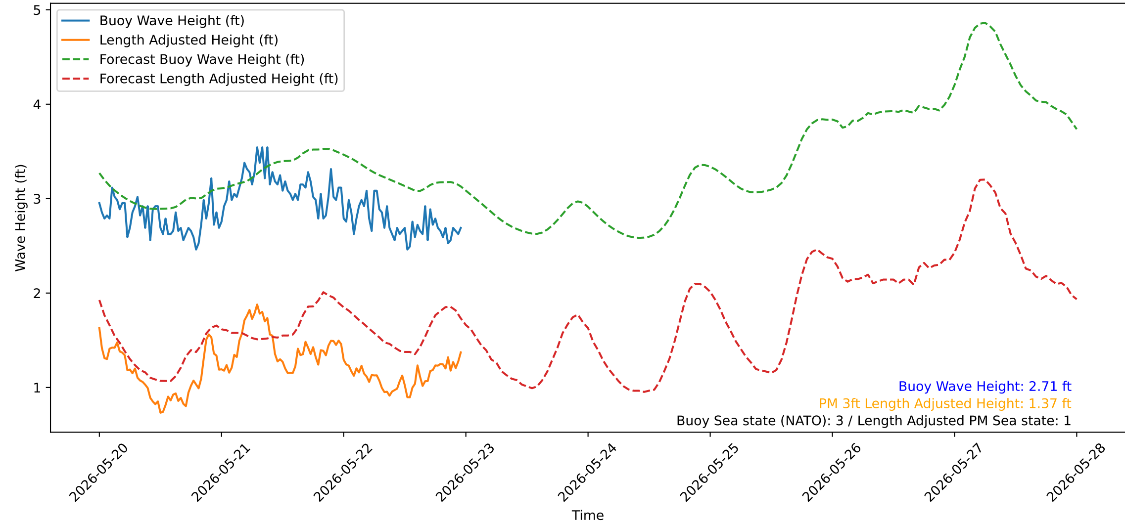
Wave Heights over Time for Green Beach at 2026-05-22 23:51:14
