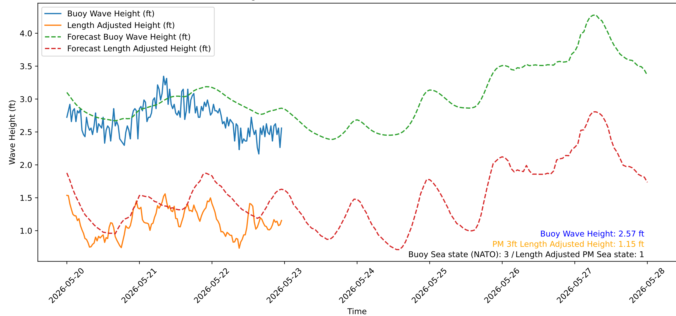
Wave Heights over Time for Red Beach at 2026-05-22 23:50:52
