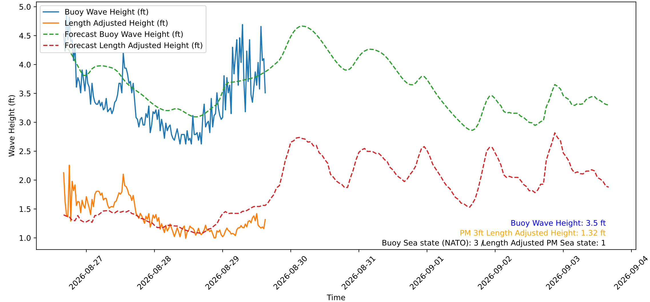
Wave Heights over Time for Red Beach at 2026-08-29 15:50:51
