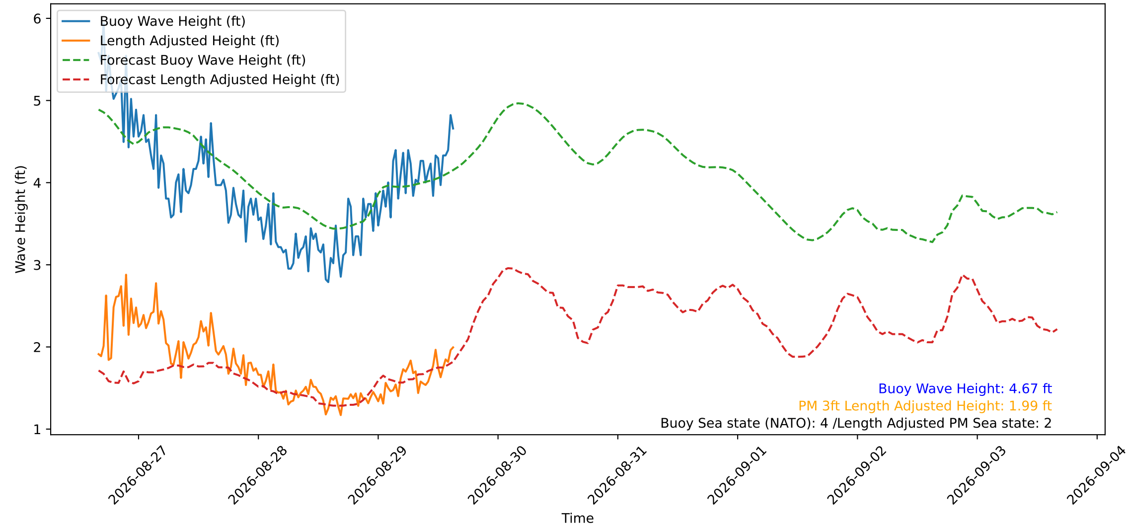
Wave Heights over Time for Oceanside Harbor at 2026-08-29 15:50:30
