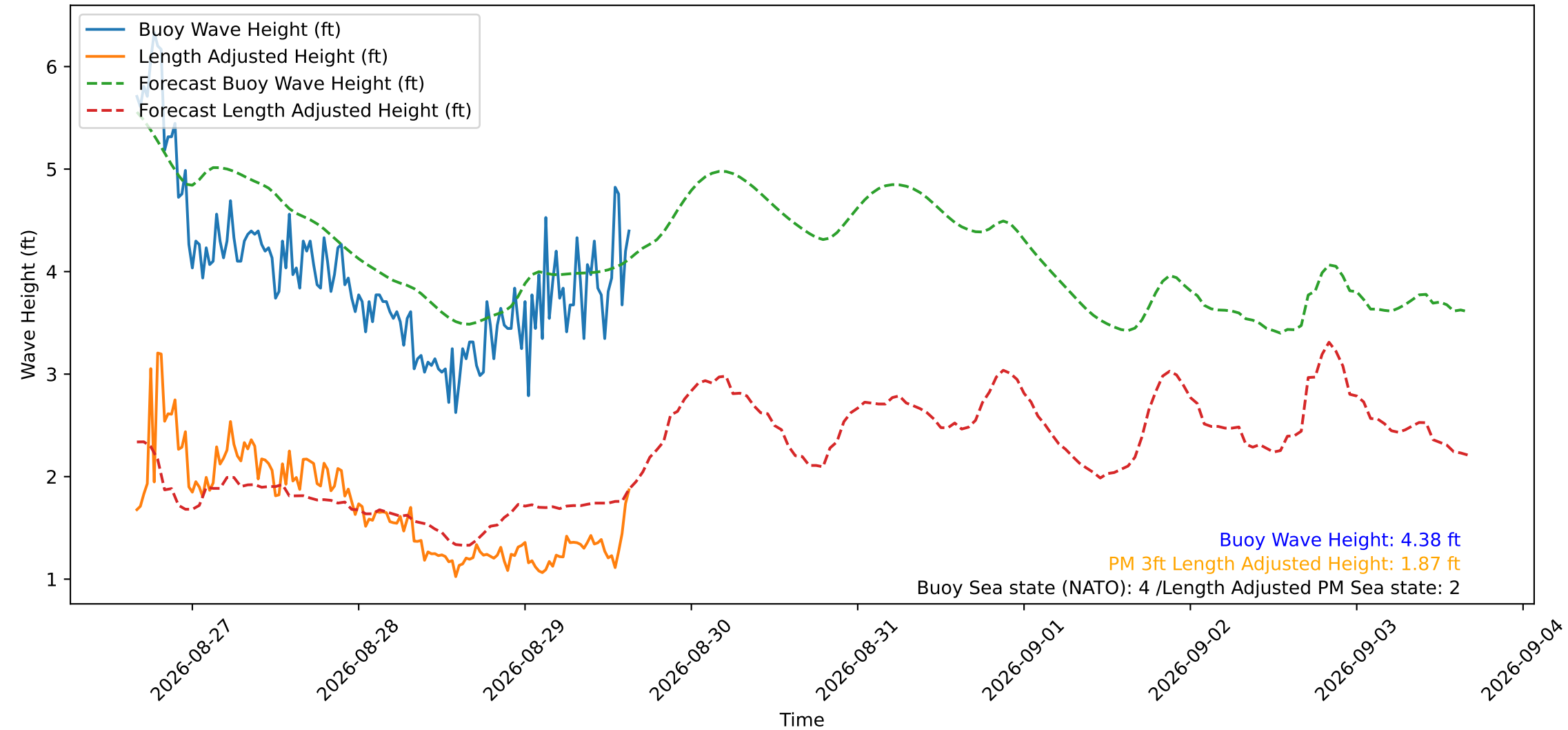
Wave Heights over Time for Green Beach at 2026-08-29 15:51:15
