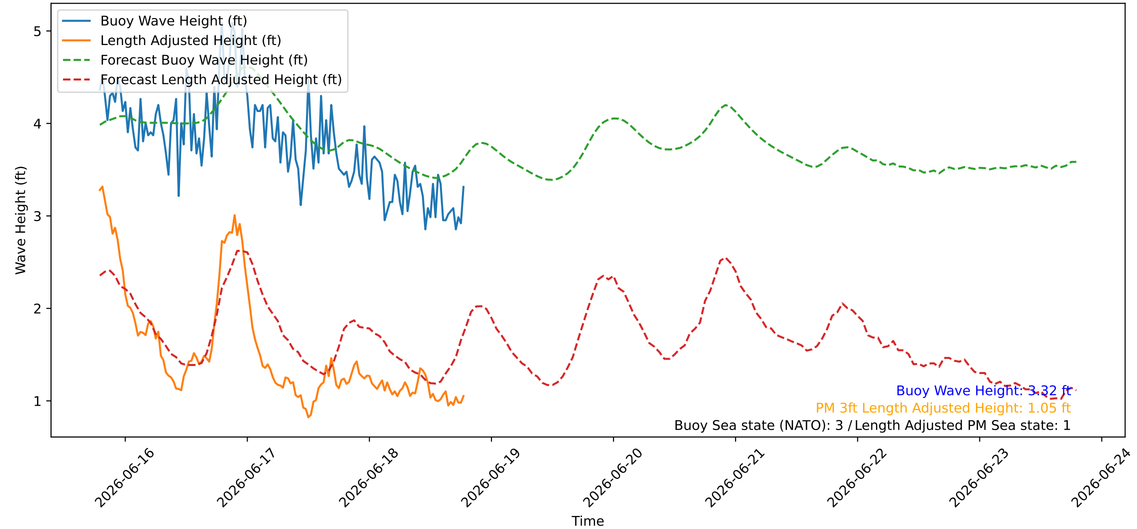
Wave Heights over Time for Green Beach at 2026-06-18 19:11:07
