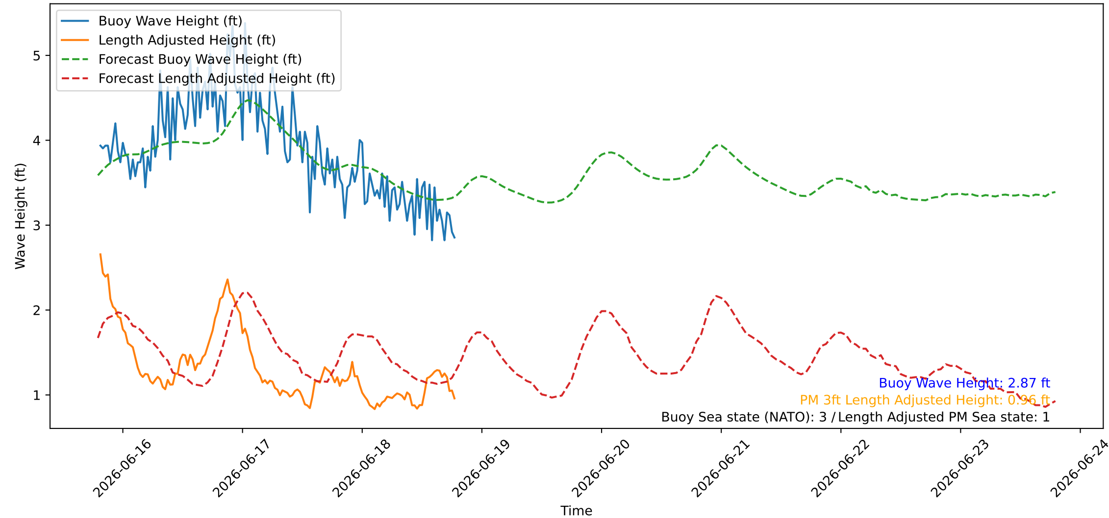
Wave Heights over Time for Red Beach at 2026-06-18 19:10:45
