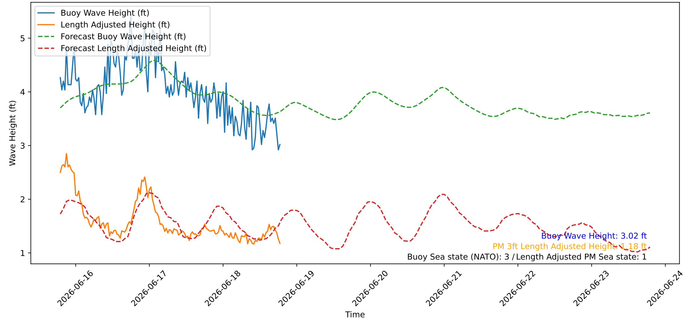
Wave Heights over Time for Oceanside Harbor at 2026-06-18 19:10:26
