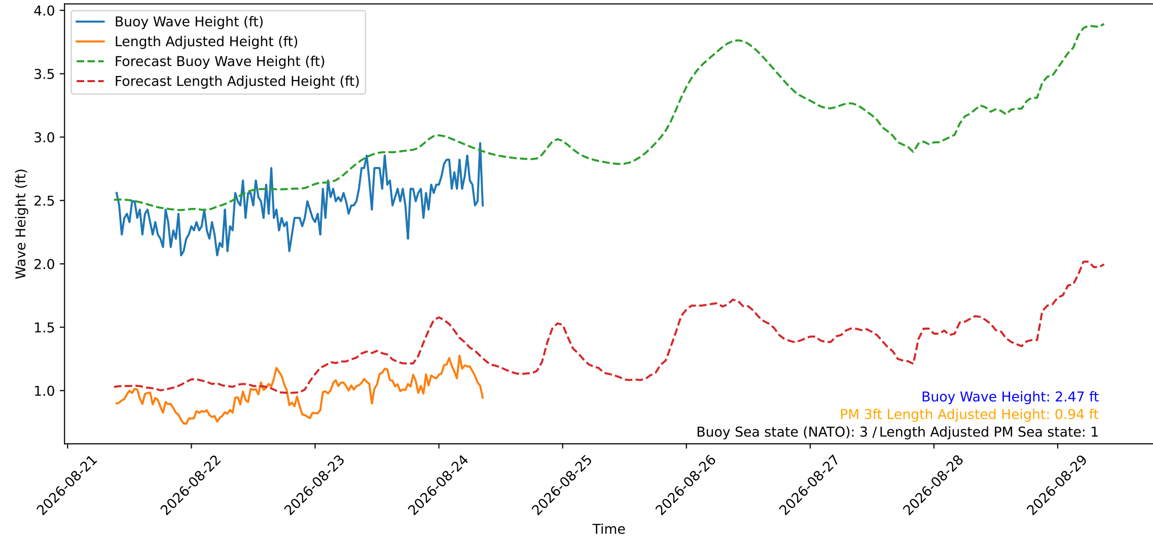
Wave Heights over Time for Red Beach at 2026-08-24 09:10:48
