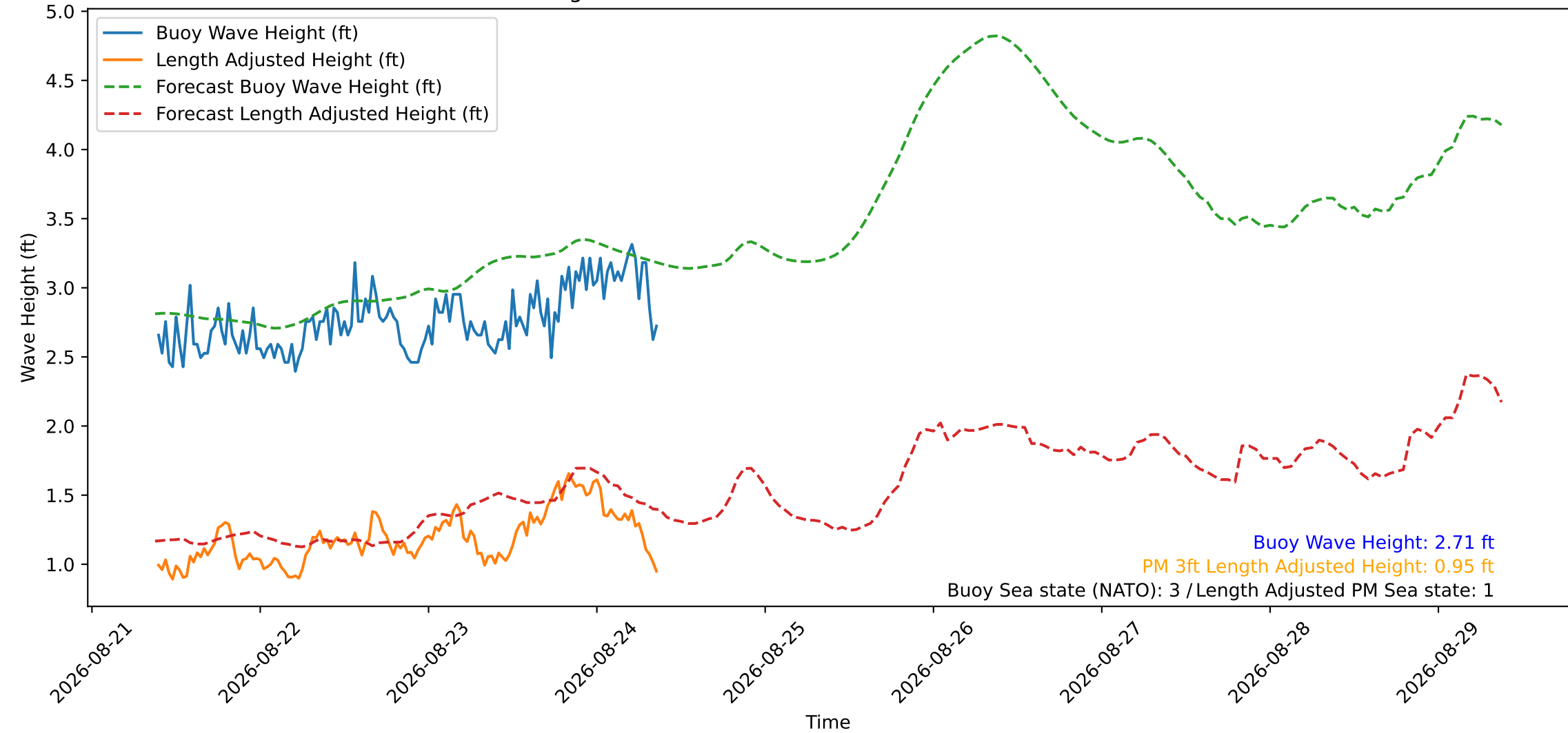
Wave Heights over Time for Green Beach at 2026-08-24 09:11:11
