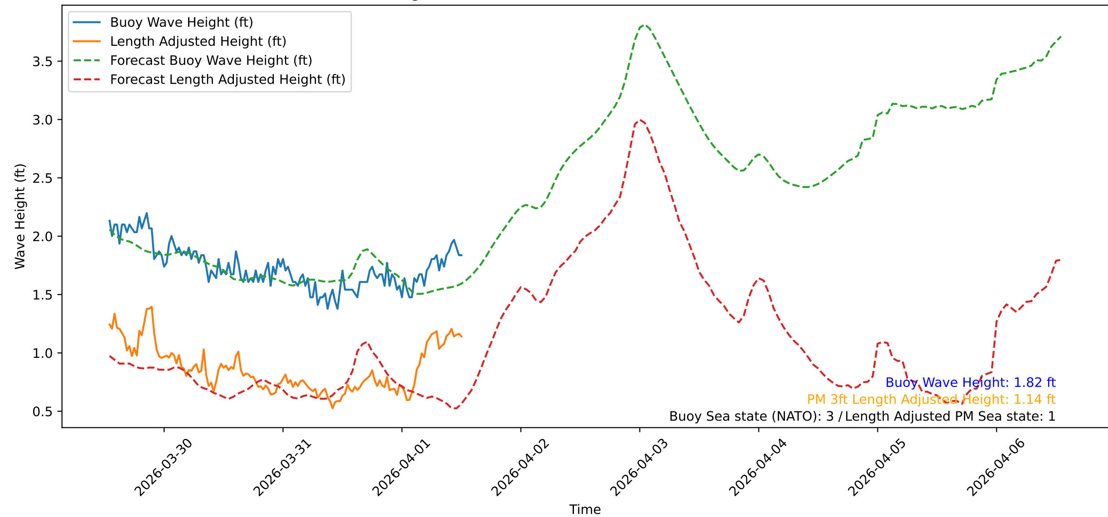
Wave Heights over Time for Red Beach at 2026-04-01 12:50:48
