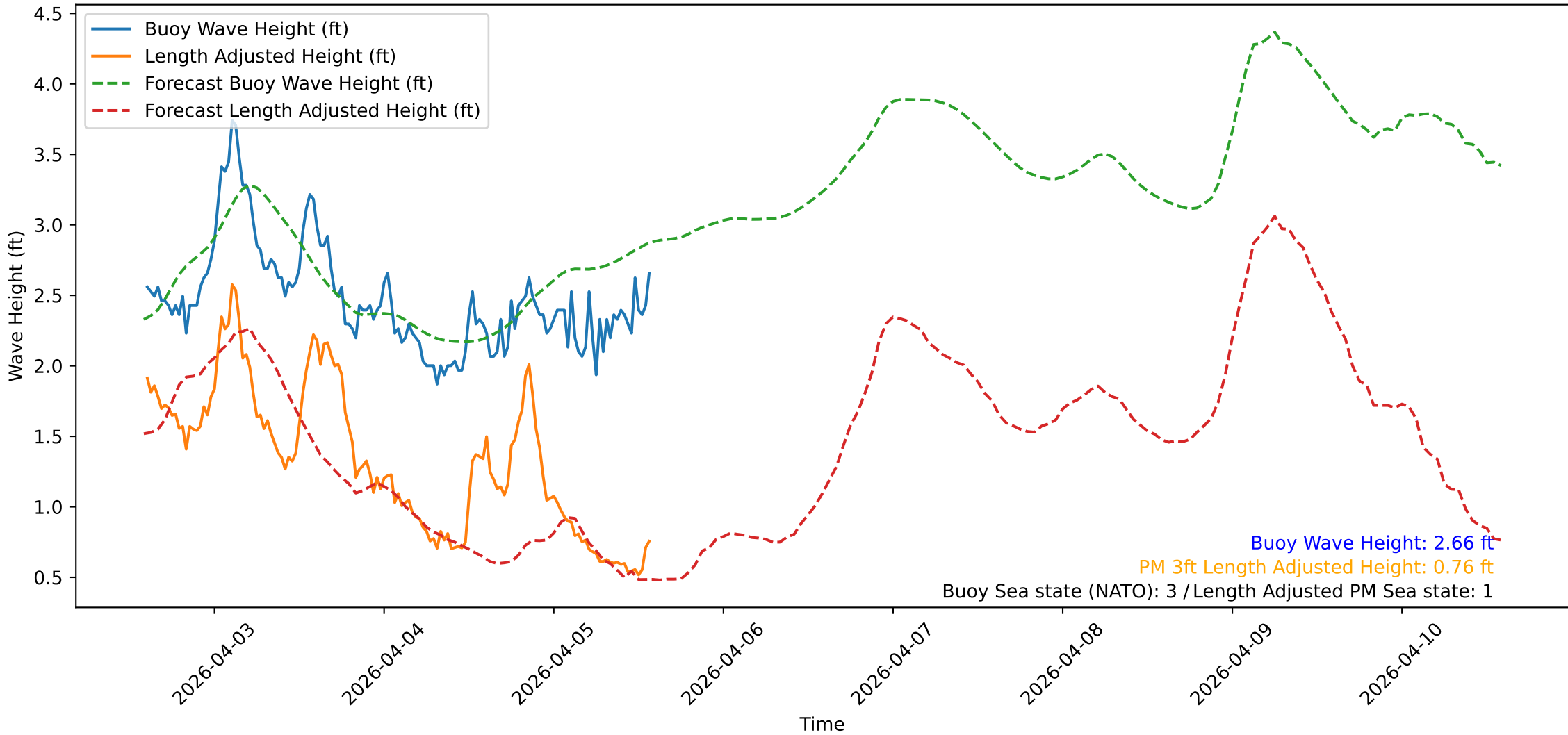
Wave Heights over Time for Red Beach at 2026-04-05 14:20:47
