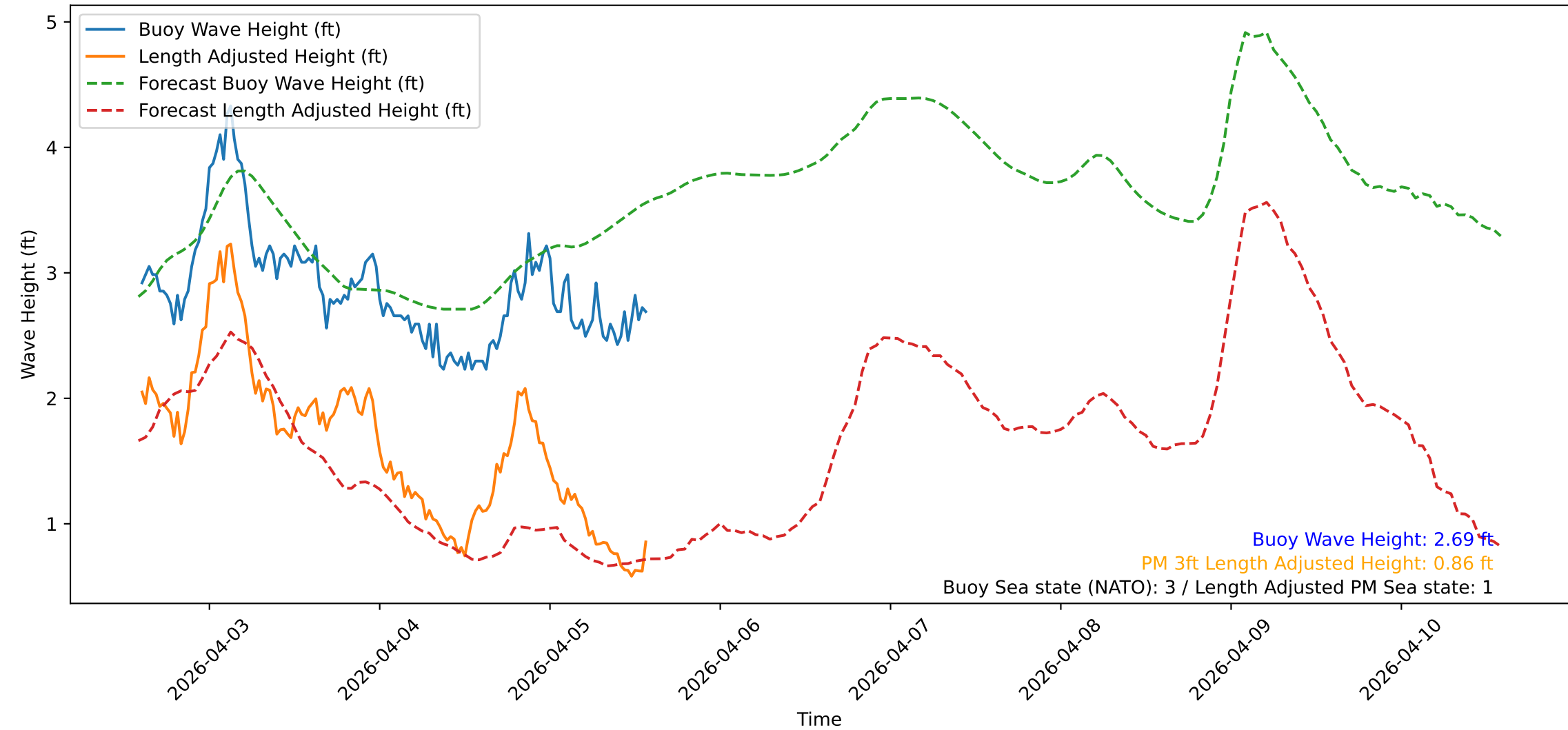
Wave Heights over Time for Green Beach at 2026-04-05 14:21:10
