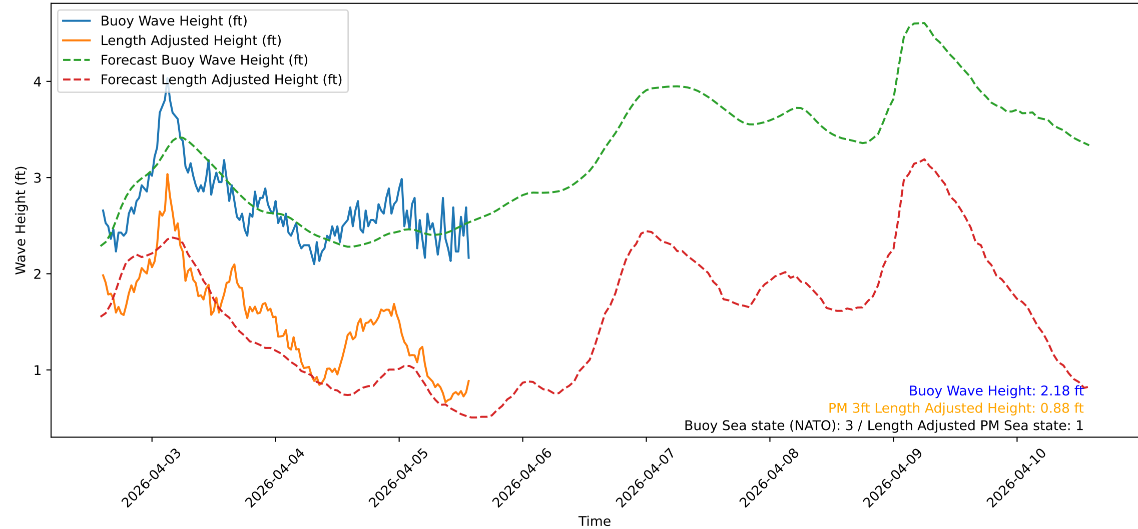
Wave Heights over Time for Oceanside Harbor at 2026-04-05 14:20:31
