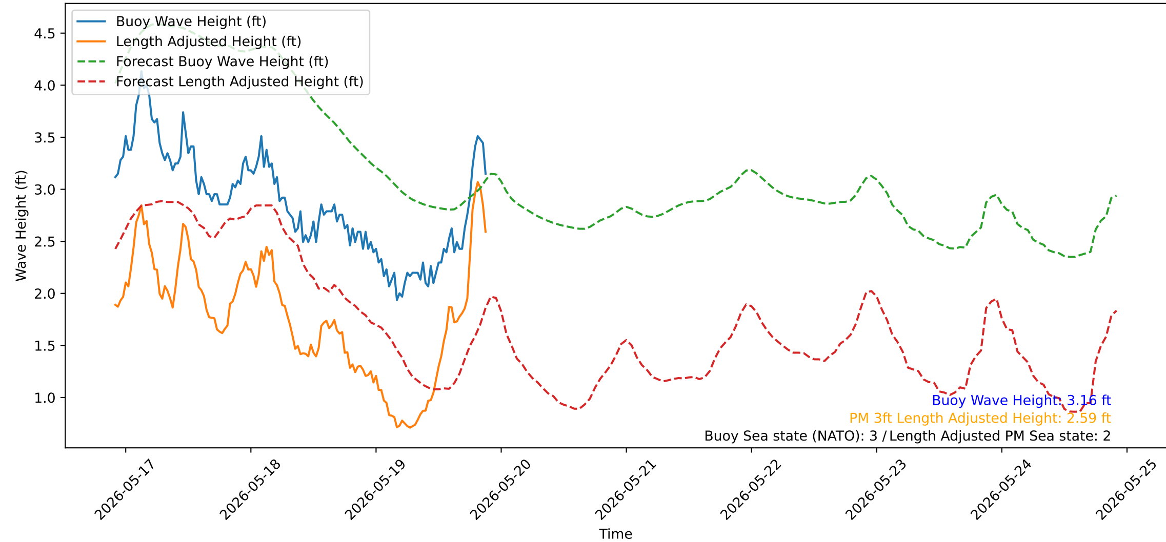
Wave Heights over Time for Red Beach at 2026-05-19 21:50:51
