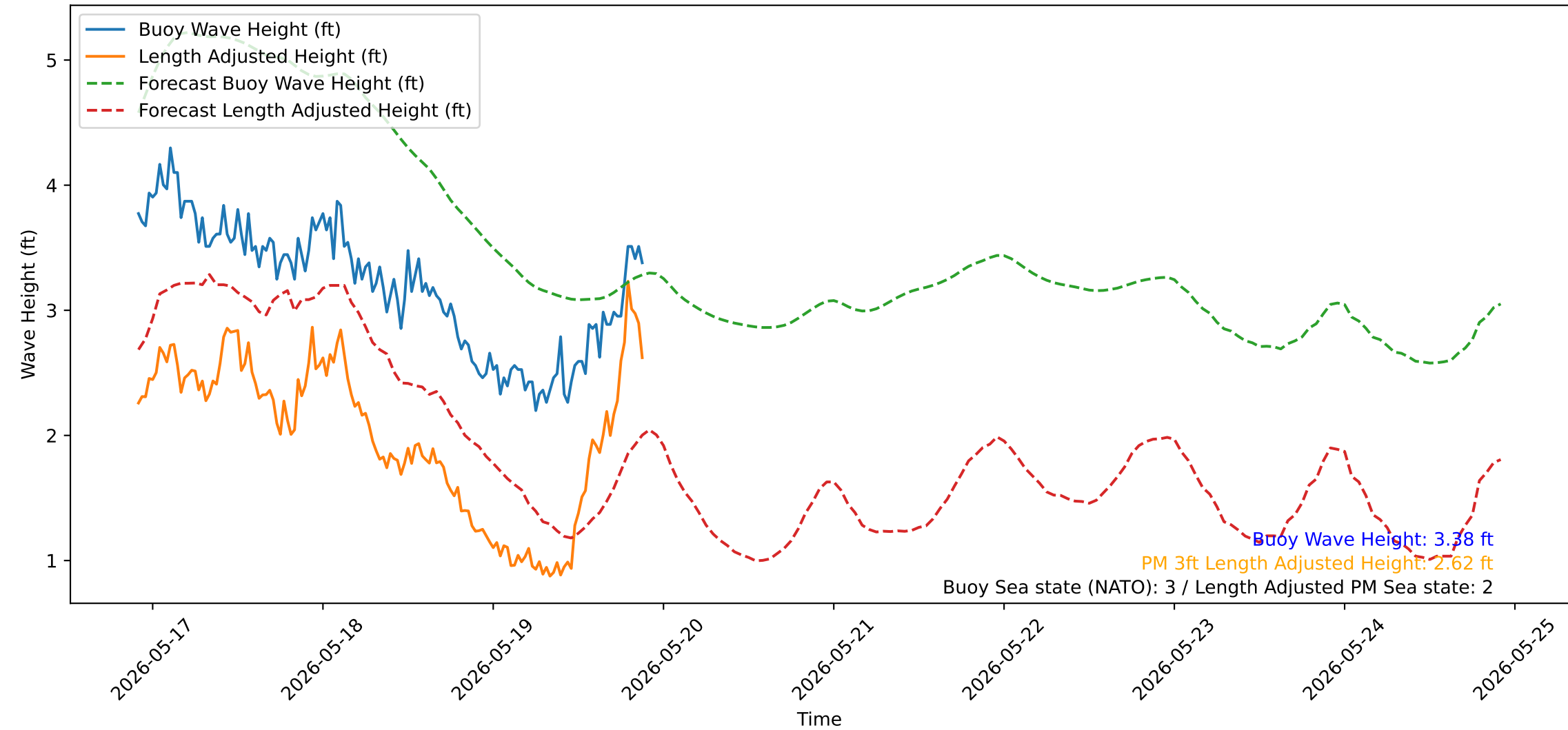
Wave Heights over Time for Oceanside Harbor at 2026-05-19 21:50:31
