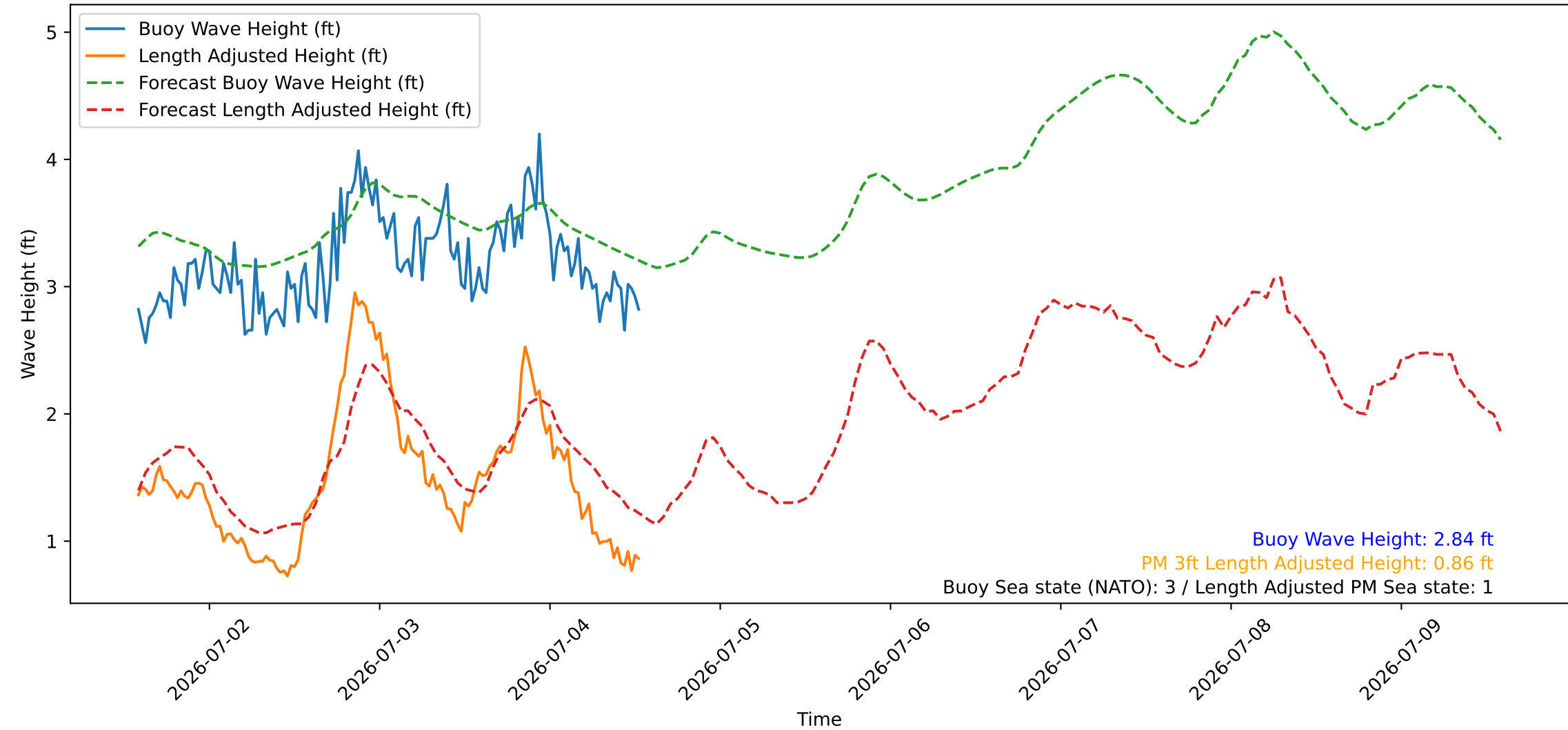
Wave Heights over Time for Green Beach at 2026-07-04 13:51:09
