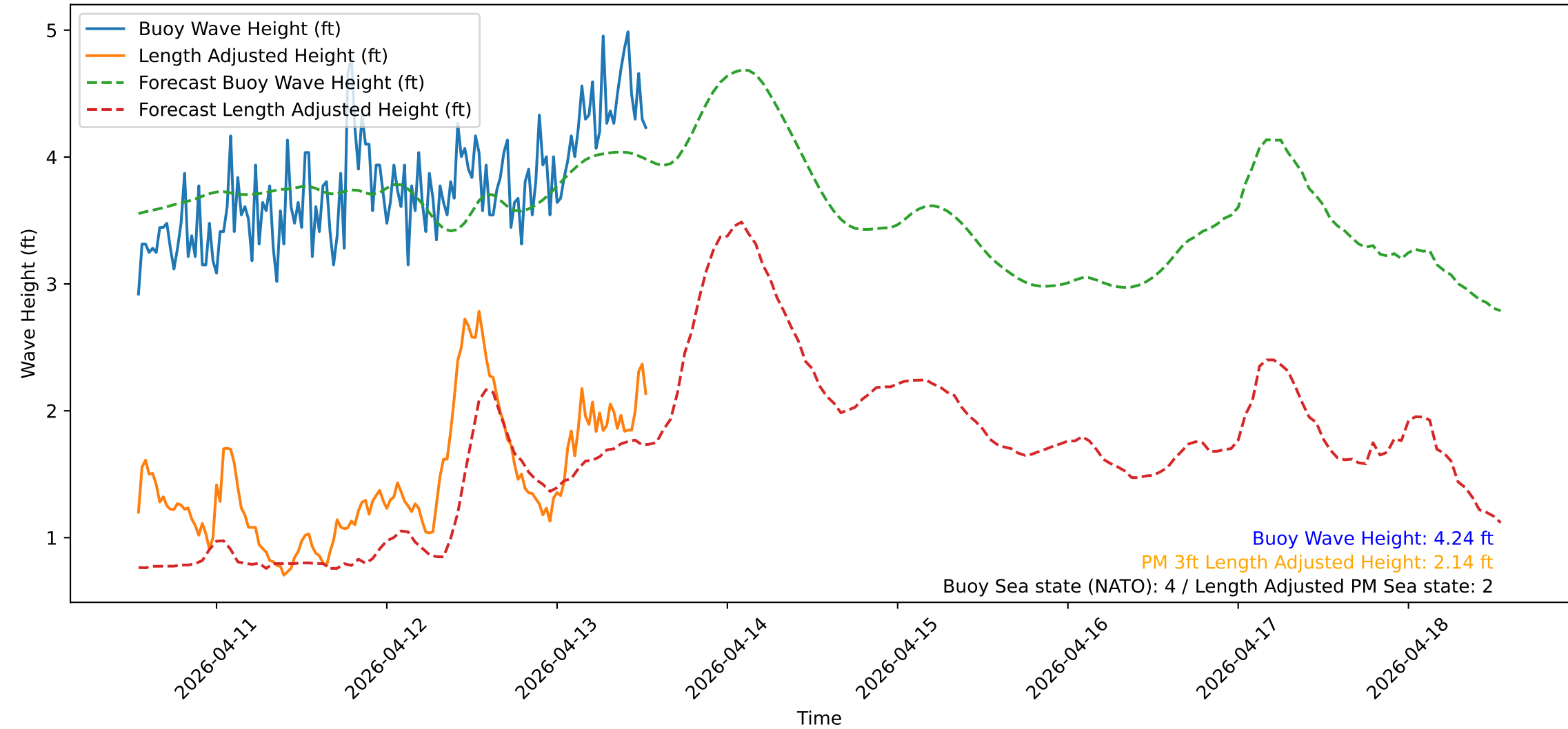
Wave Heights over Time for Oceanside Harbor at 2026-04-13 13:00:31
