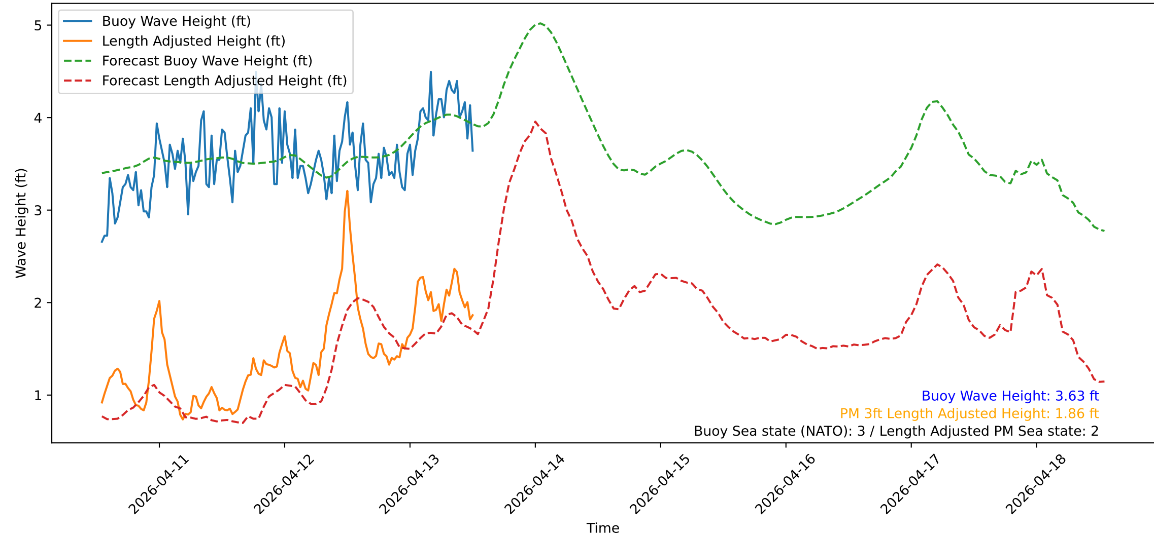
Wave Heights over Time for Green Beach at 2026-04-13 13:01:13
