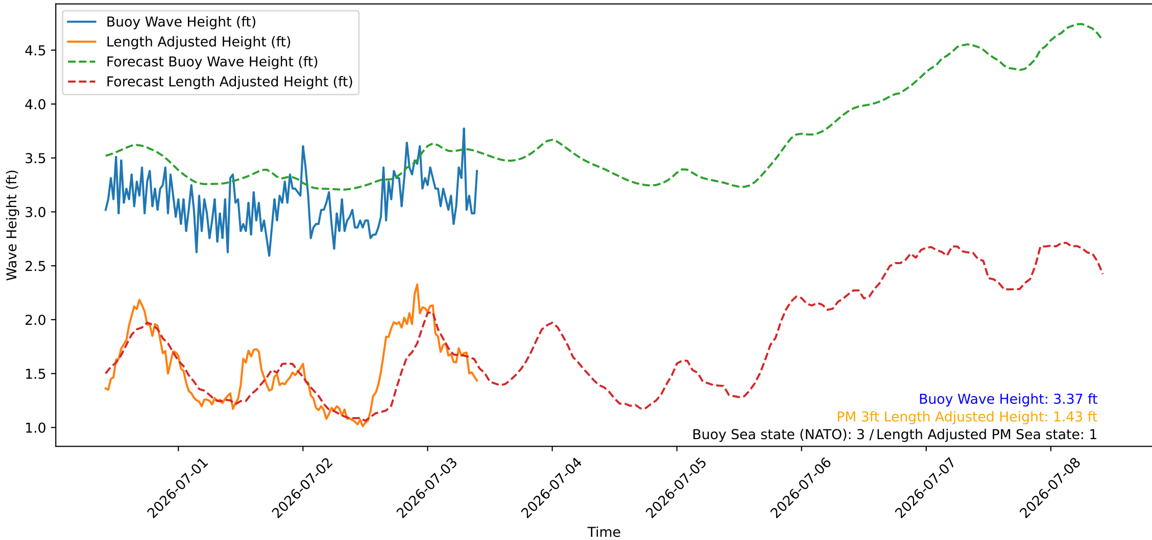
Wave Heights over Time for Oceanside Harbor at 2026-07-03 10:00:26
