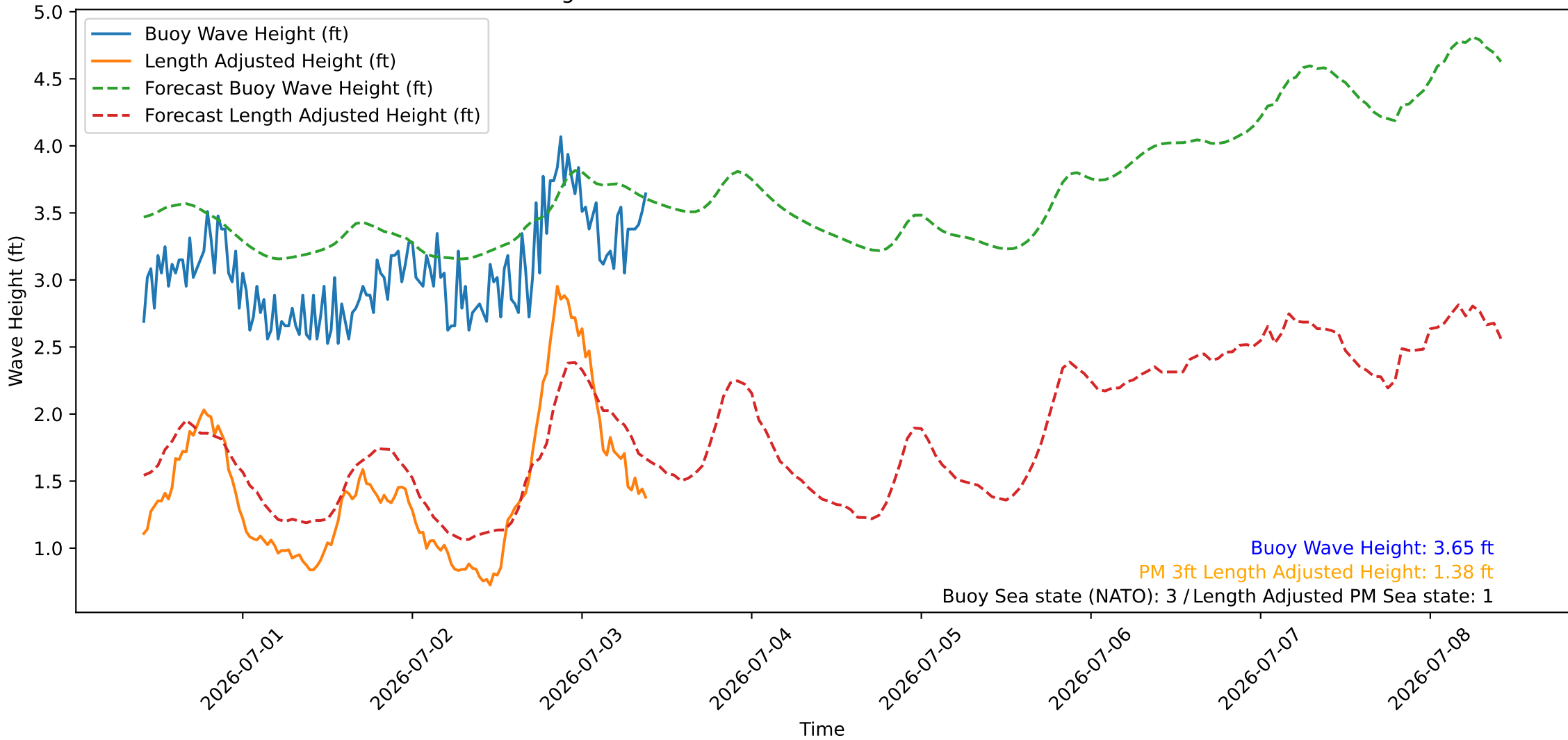
Wave Heights over Time for Green Beach at 2026-07-03 10:01:08
