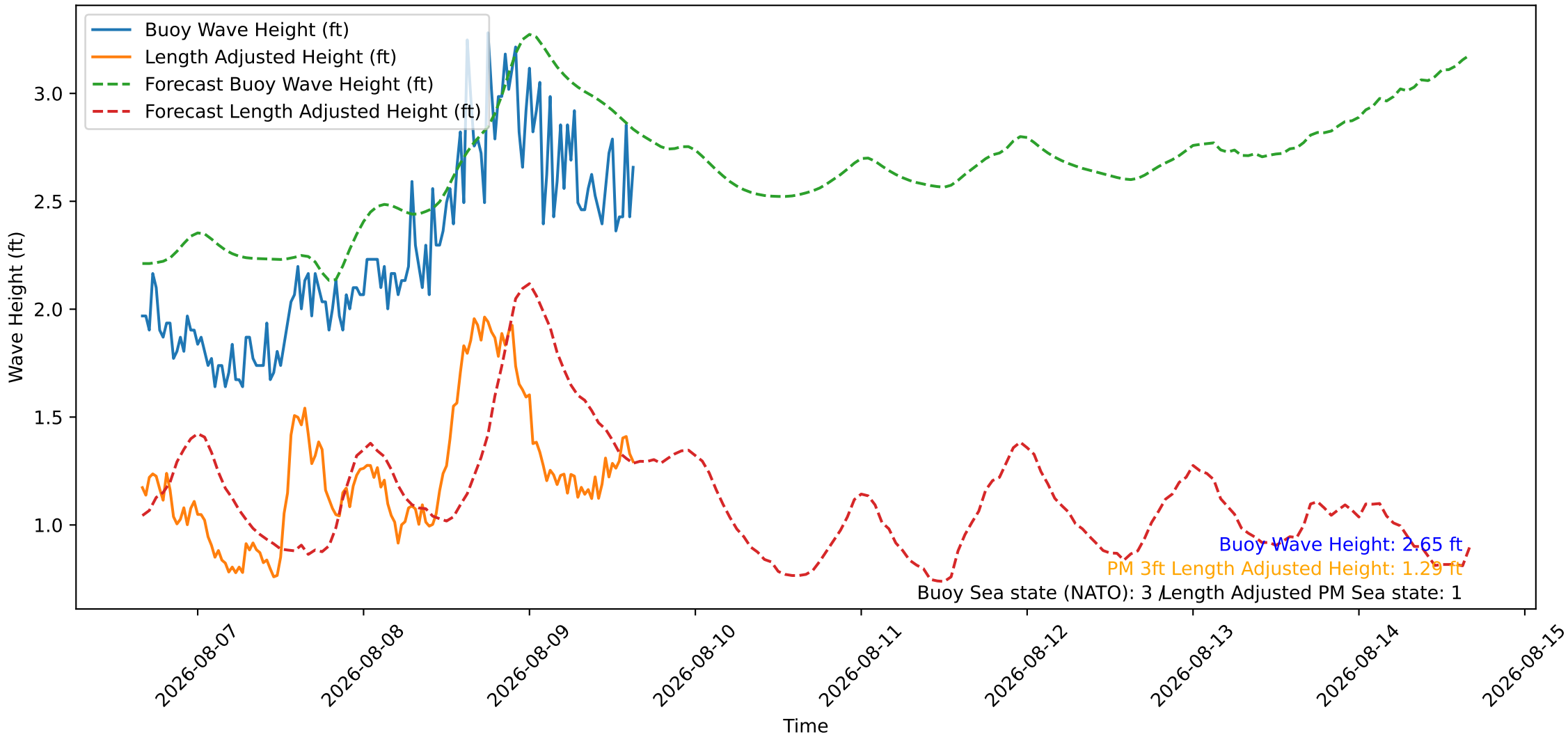
Wave Heights over Time for Oceanside Harbor at 2026-08-09 15:50:27
