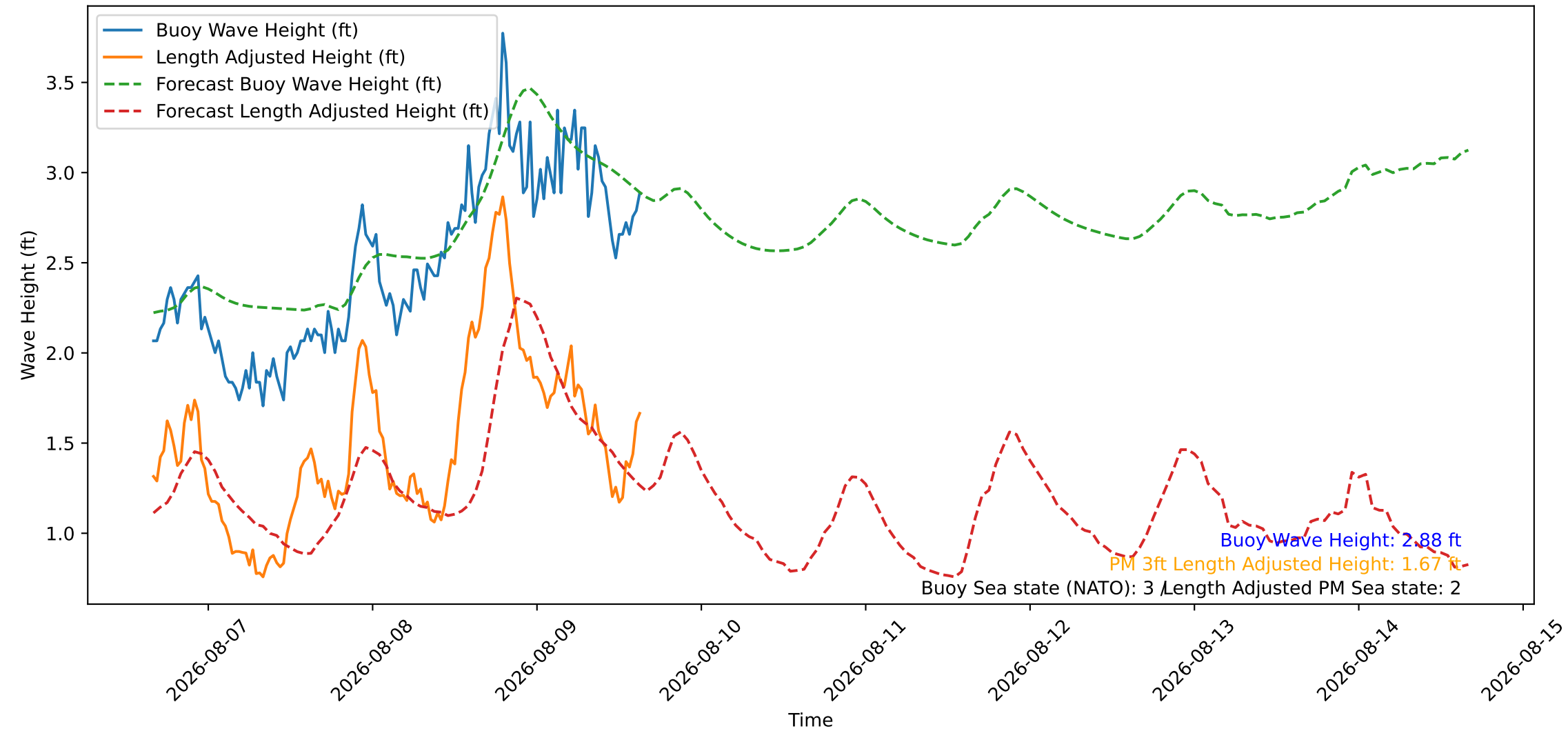
Wave Heights over Time for Green Beach at 2026-08-09 15:51:10
