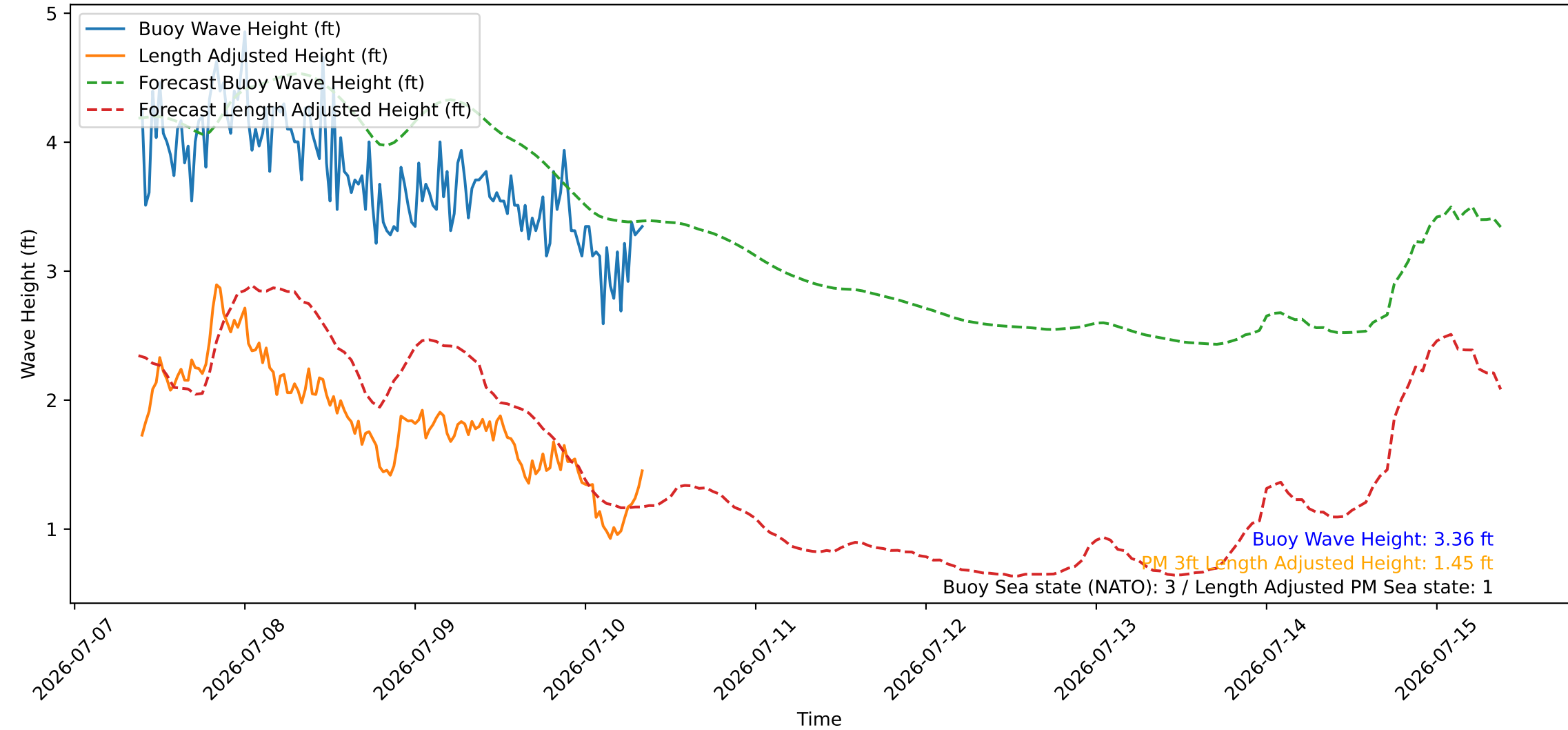
Wave Heights over Time for Red Beach at 2026-07-10 09:00:46
