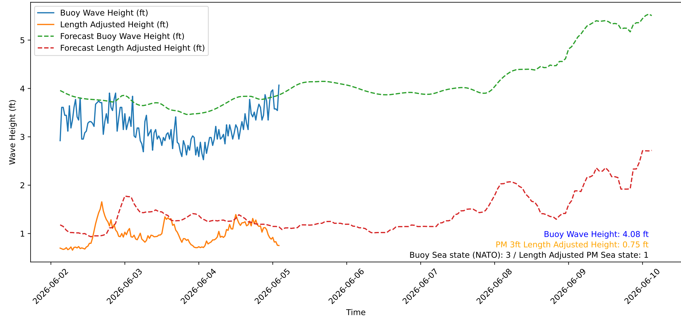
Wave Heights over Time for Red Beach at 2026-06-05 02:50:46
