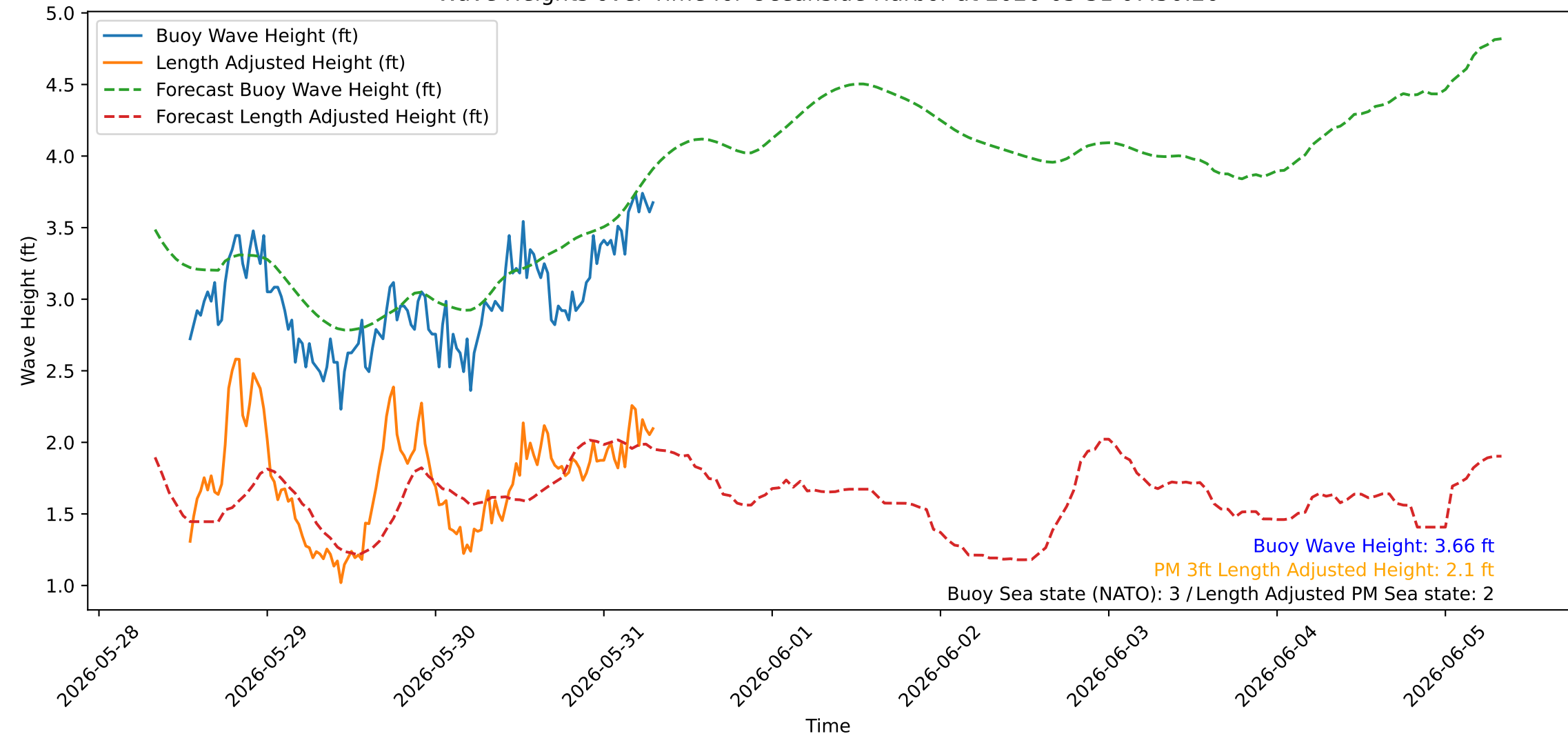
Wave Heights over Time for Oceanside Harbor at 2026-05-31 07:50:26
