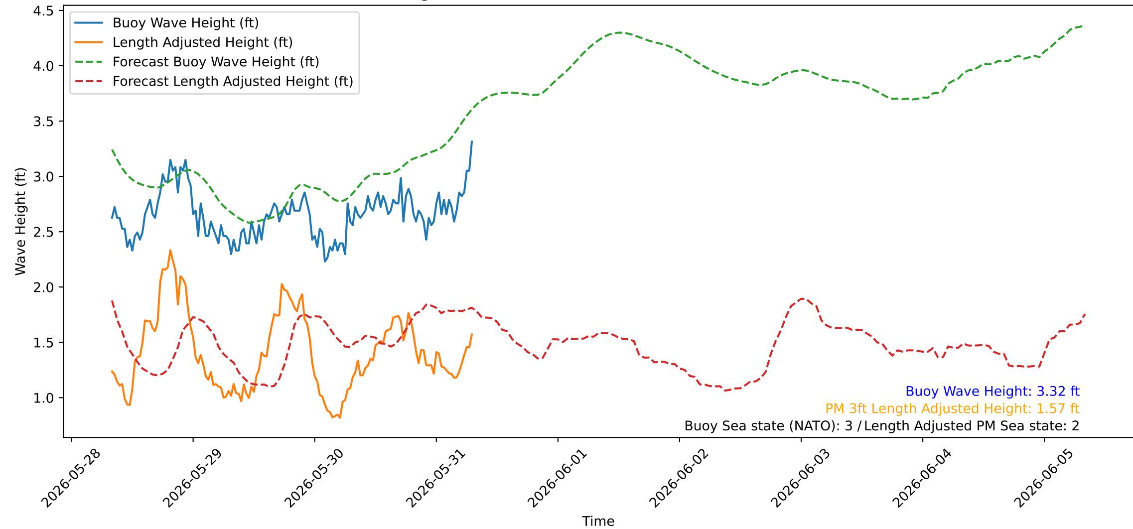
Wave Heights over Time for Red Beach at 2026-05-31 07:50:46
