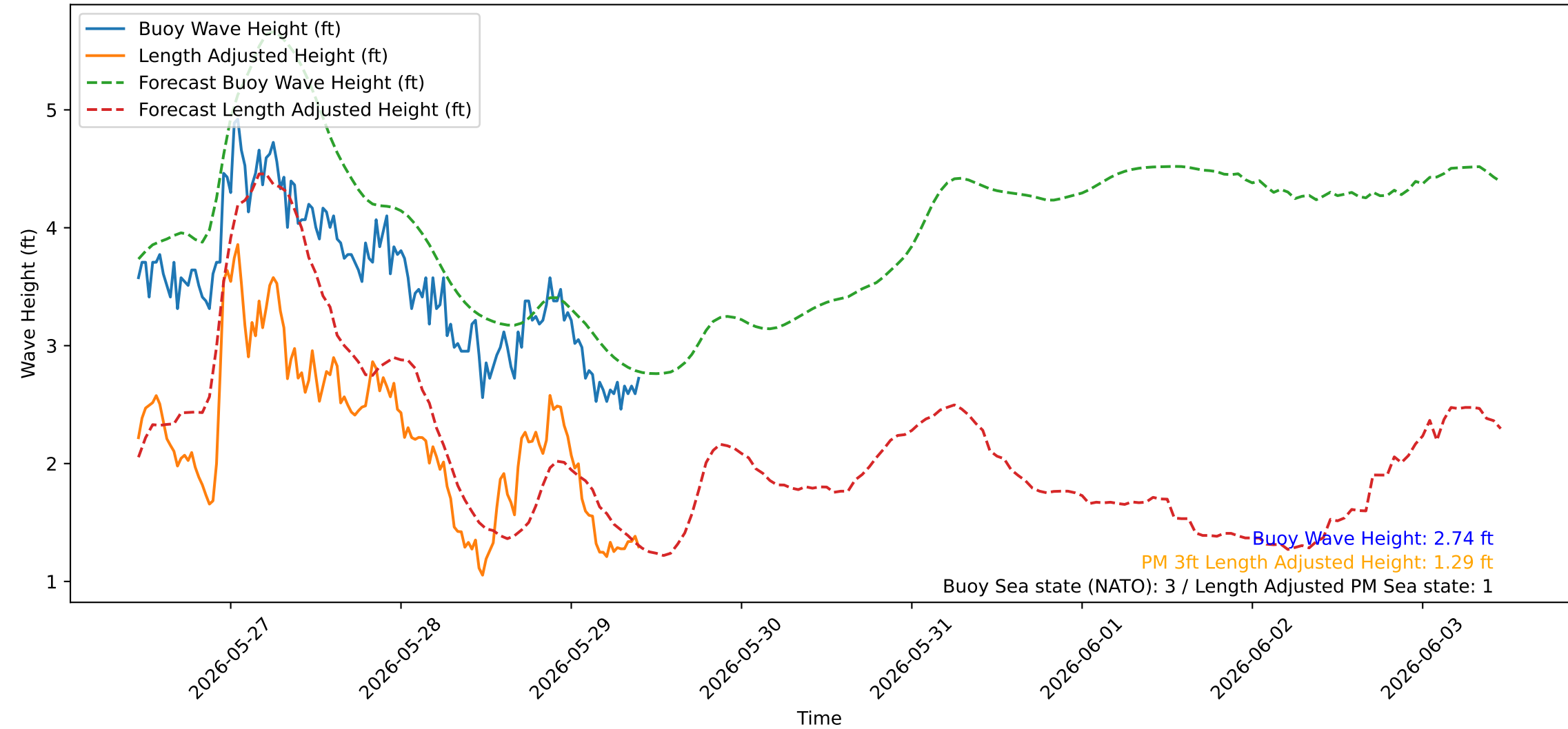
Wave Heights over Time for Green Beach at 2026-05-29 11:01:05
