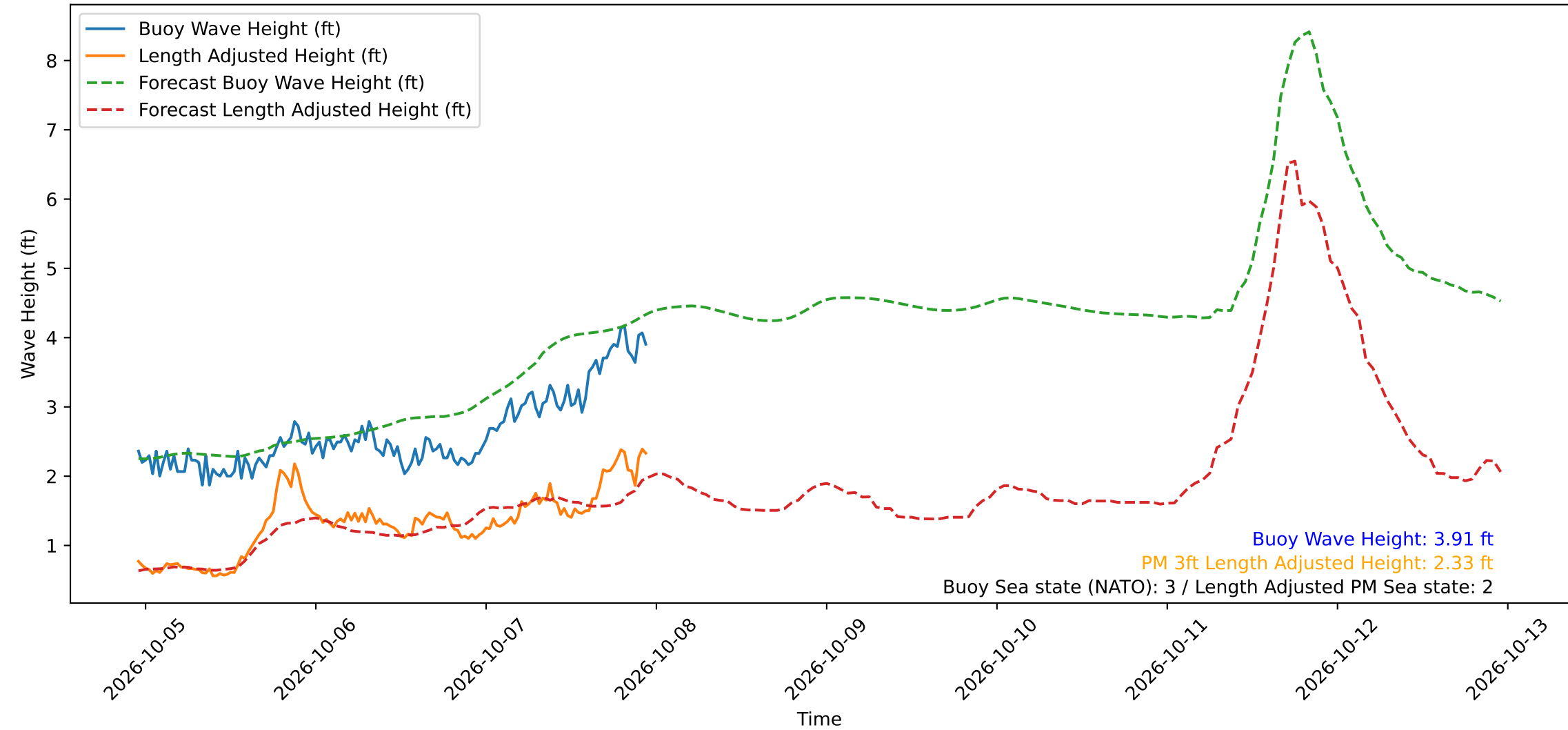
Wave Heights over Time for Oceanside Harbor at 2026-10-07 23:10:30
