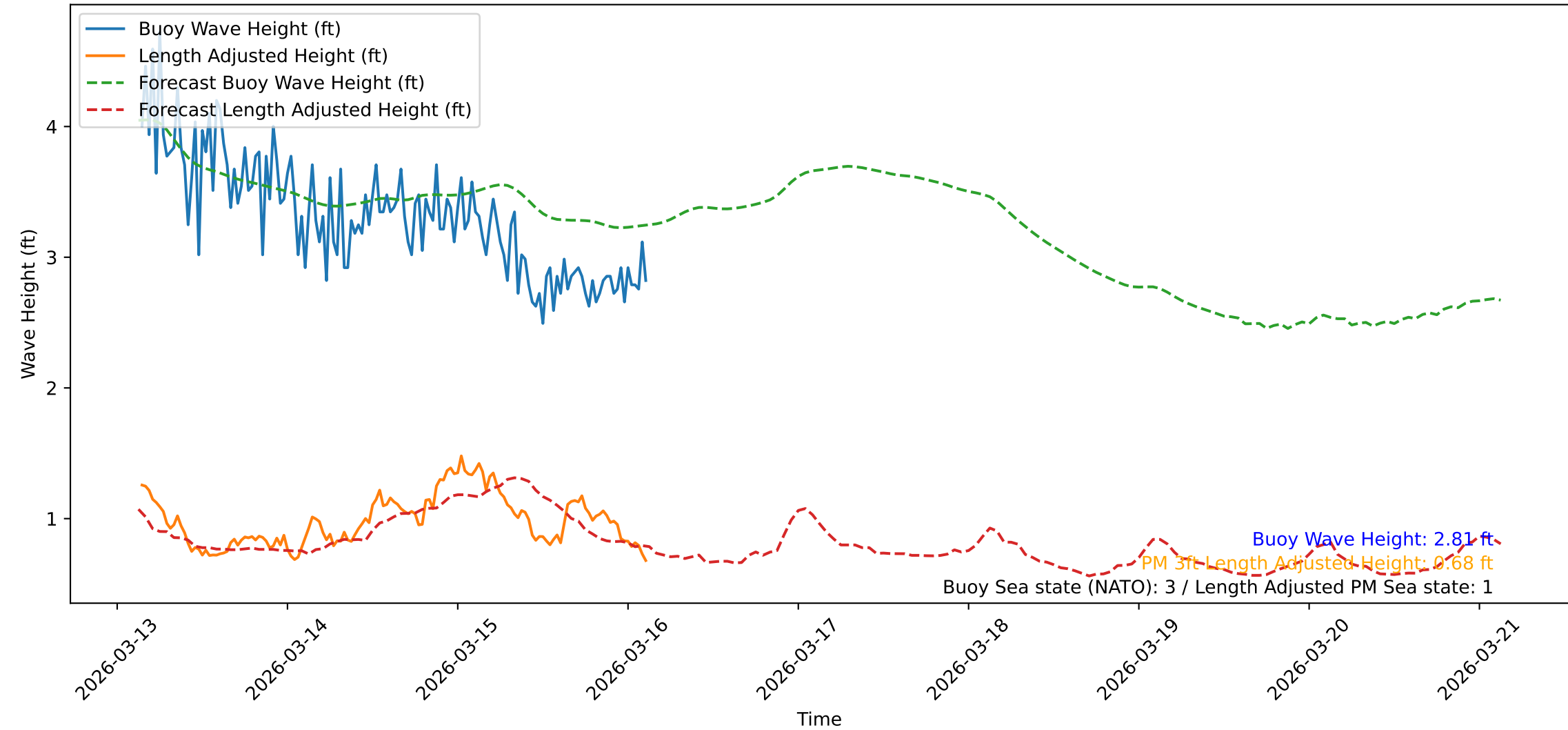
Wave Heights over Time for Oceanside Harbor at 2026-03-16 03:20:48
