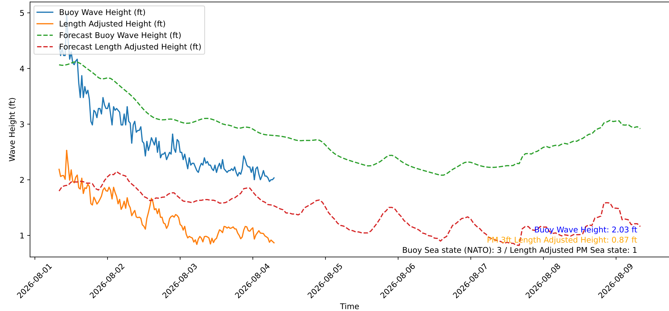
Wave Heights over Time for Green Beach at 2026-08-04 08:01:07
