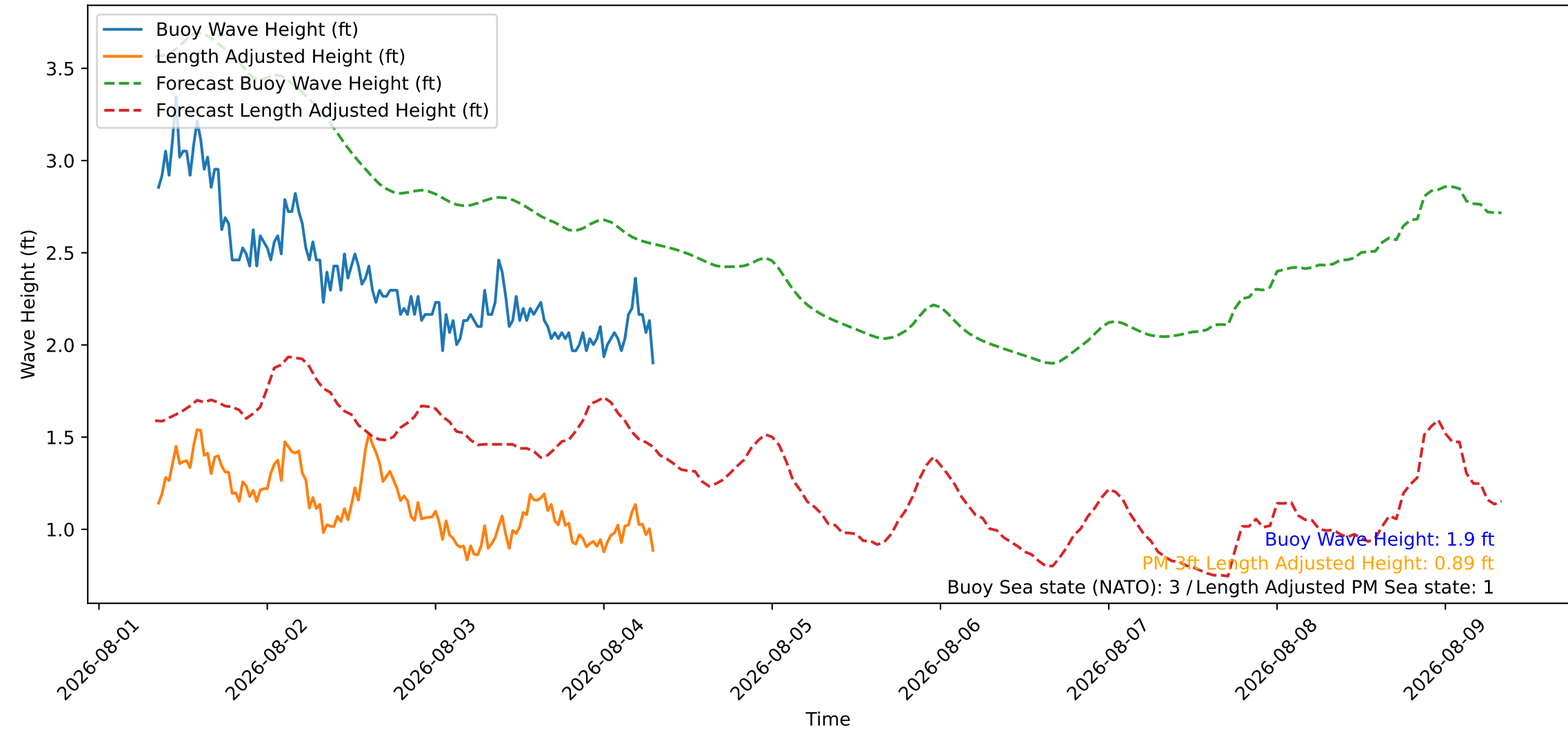
Wave Heights over Time for Red Beach at 2026-08-04 08:00:45
