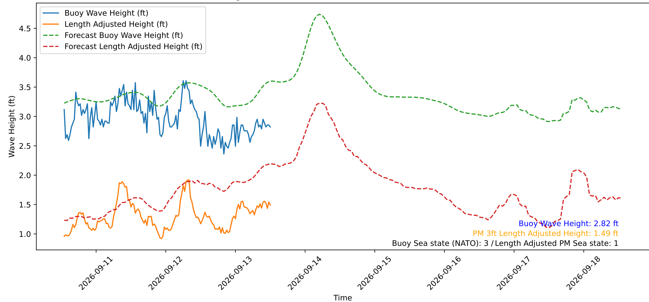
Wave Heights over Time for Green Beach at 2026-09-13 12:51:14
