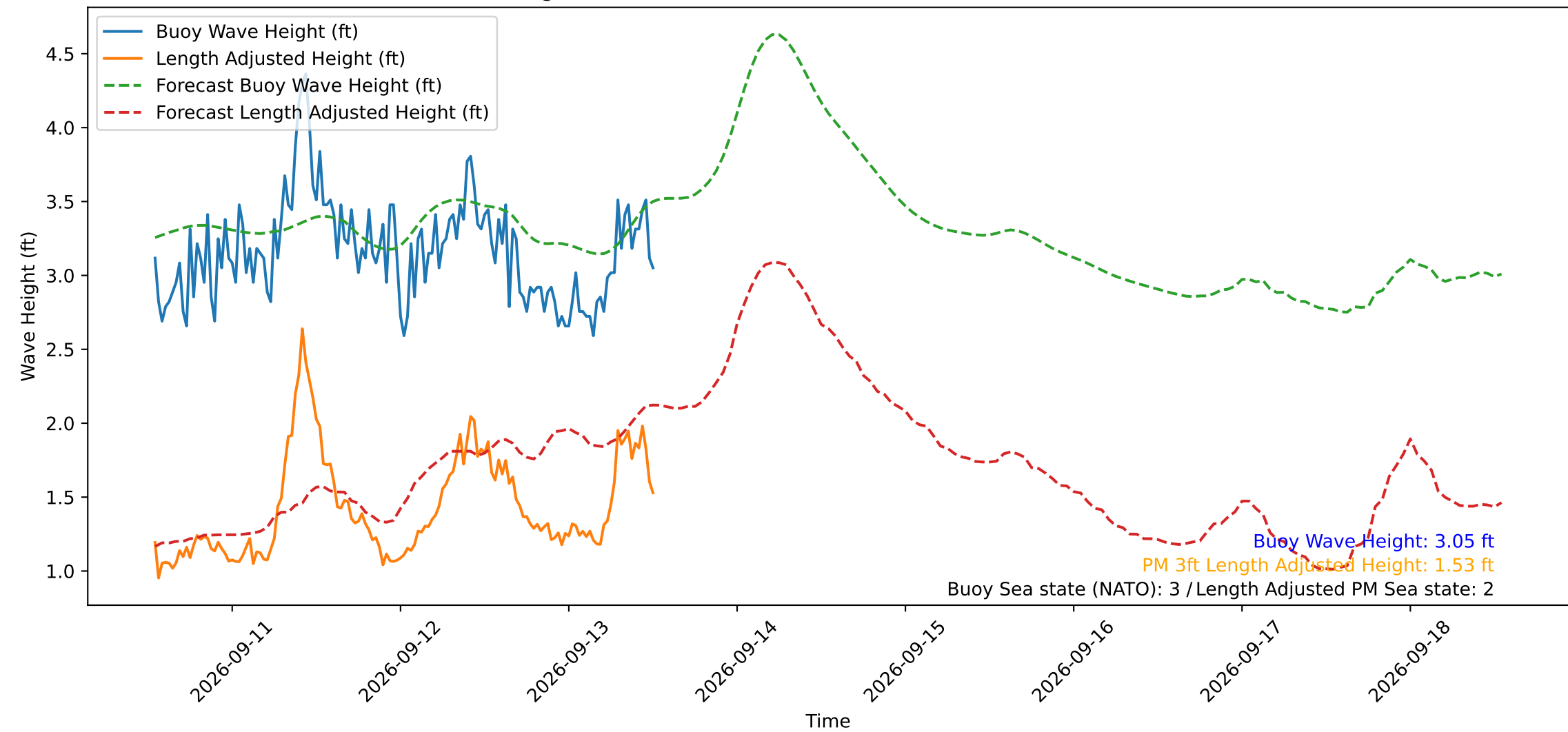
Wave Heights over Time for Oceanside Harbor at 2026-09-13 12:50:30
