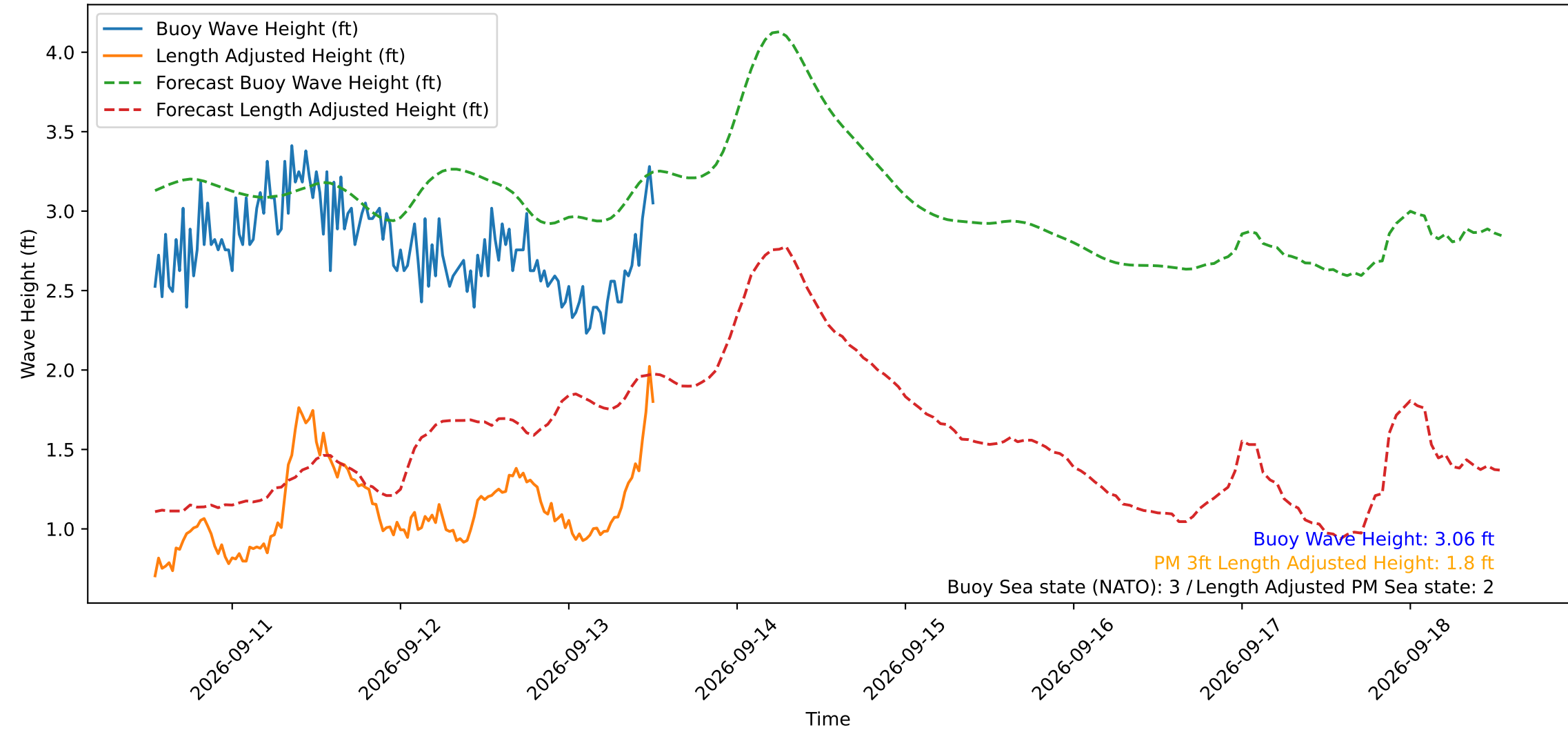
Wave Heights over Time for Red Beach at 2026-09-13 12:50:50
