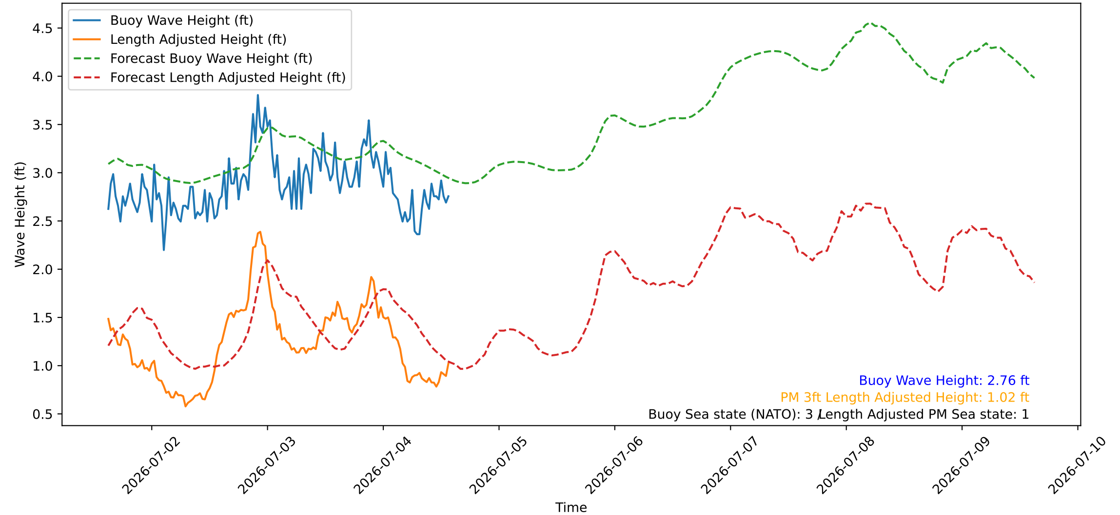
Wave Heights over Time for Red Beach at 2026-07-04 14:40:45
