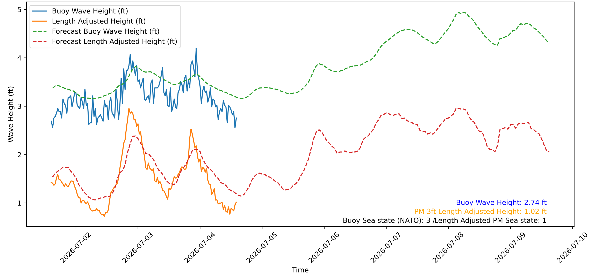
Wave Heights over Time for Green Beach at 2026-07-04 14:41:08
