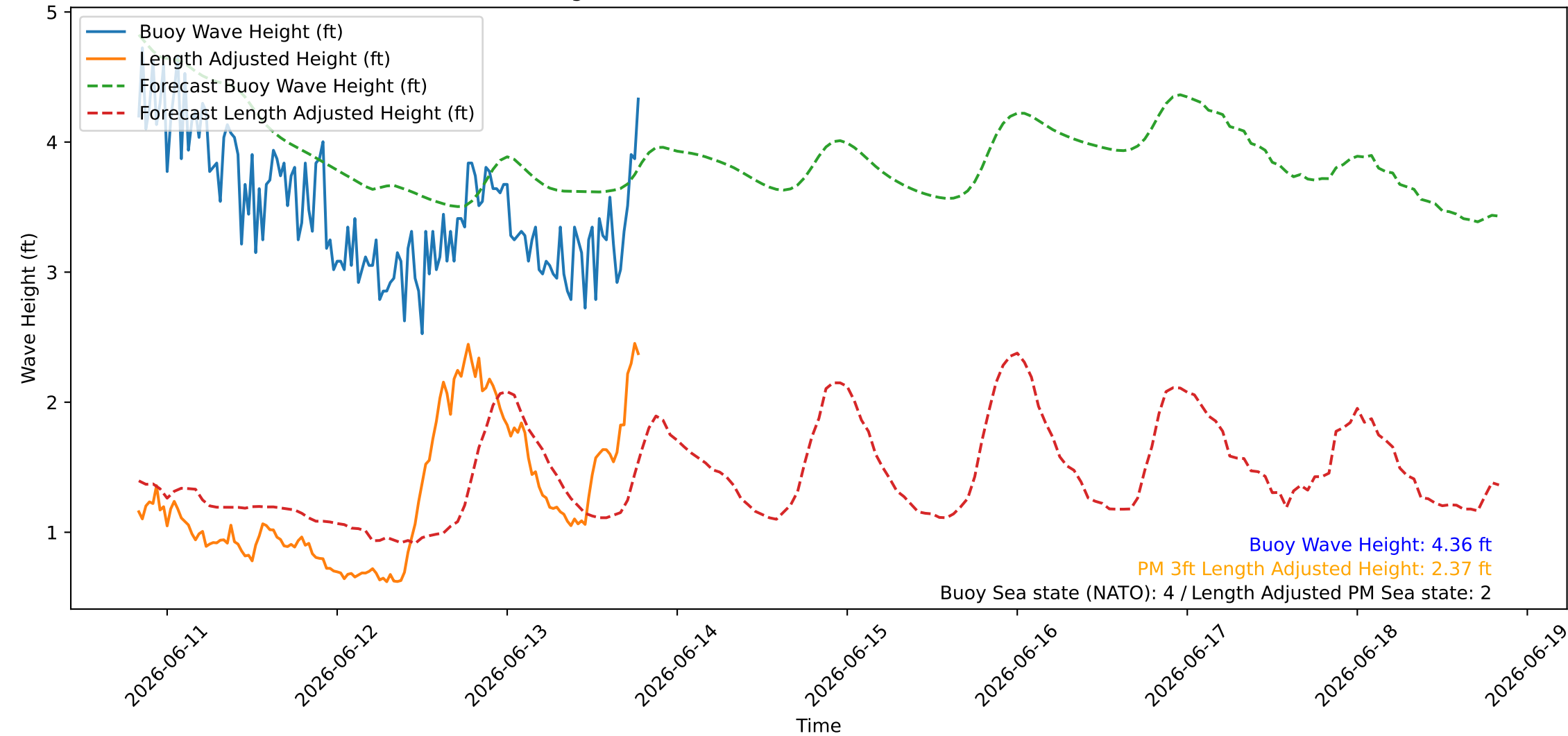
Wave Heights over Time for Red Beach at 2026-06-13 19:30:45
