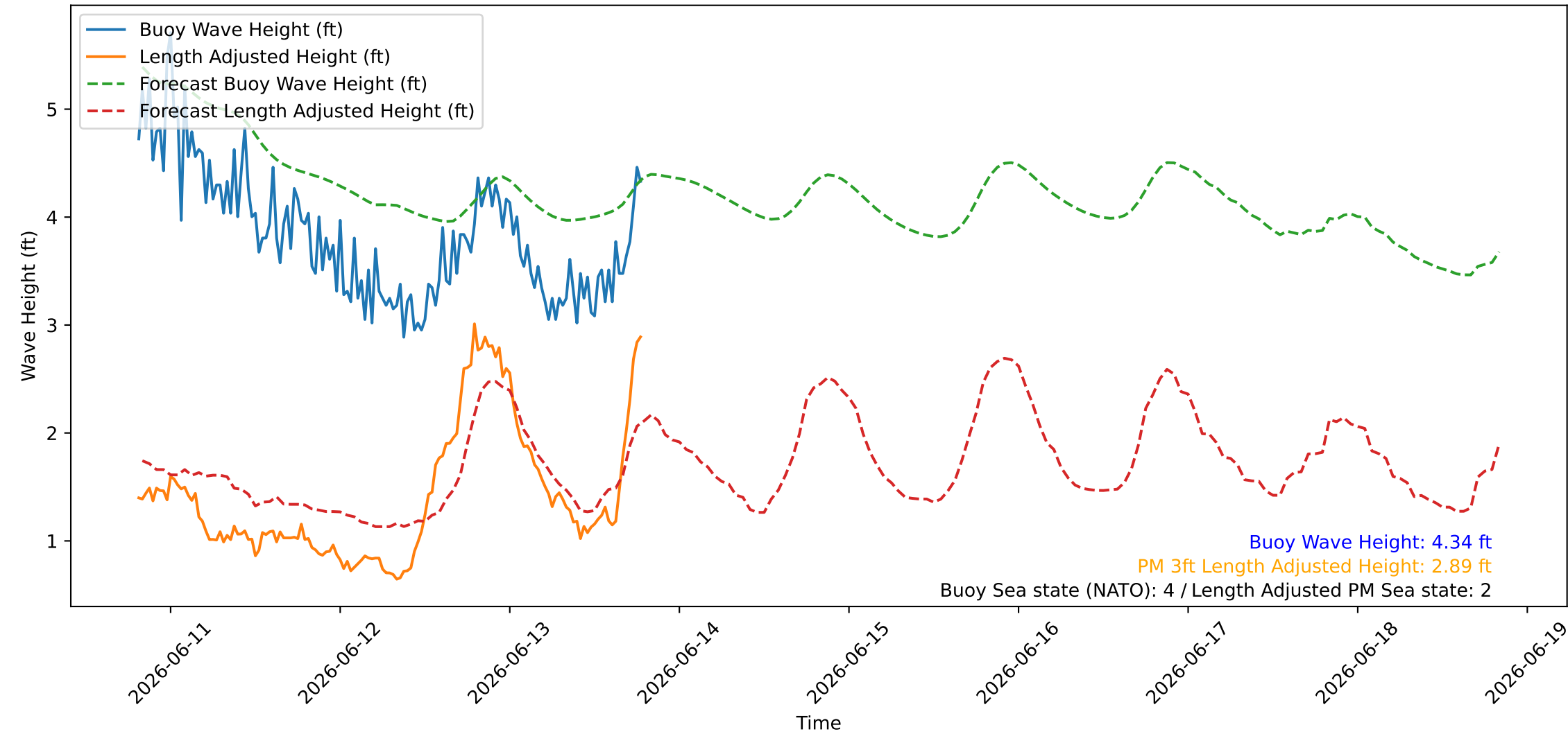
Wave Heights over Time for Green Beach at 2026-06-13 19:31:08
