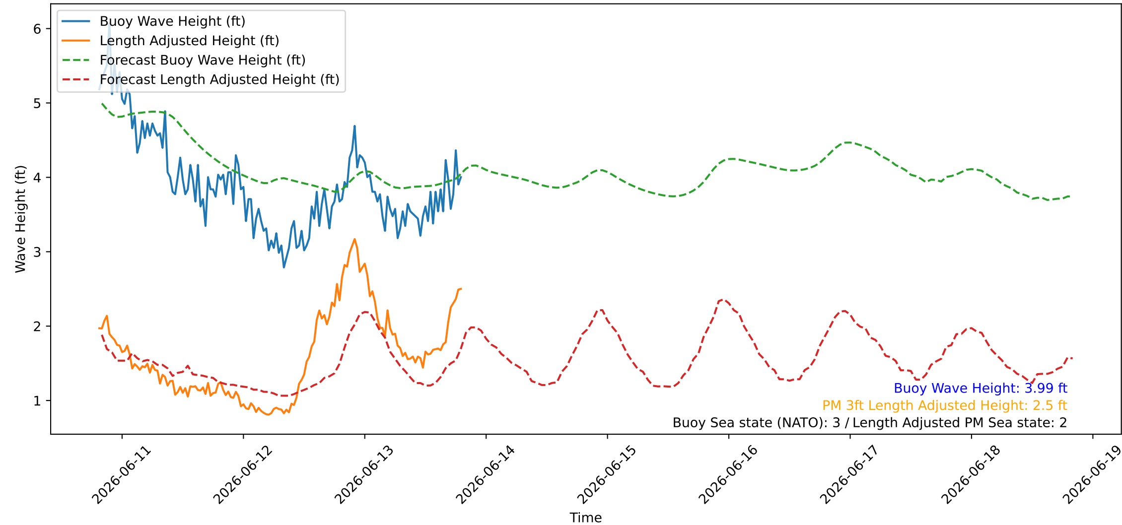
Wave Heights over Time for Oceanside Harbor at 2026-06-13 19:30:26
