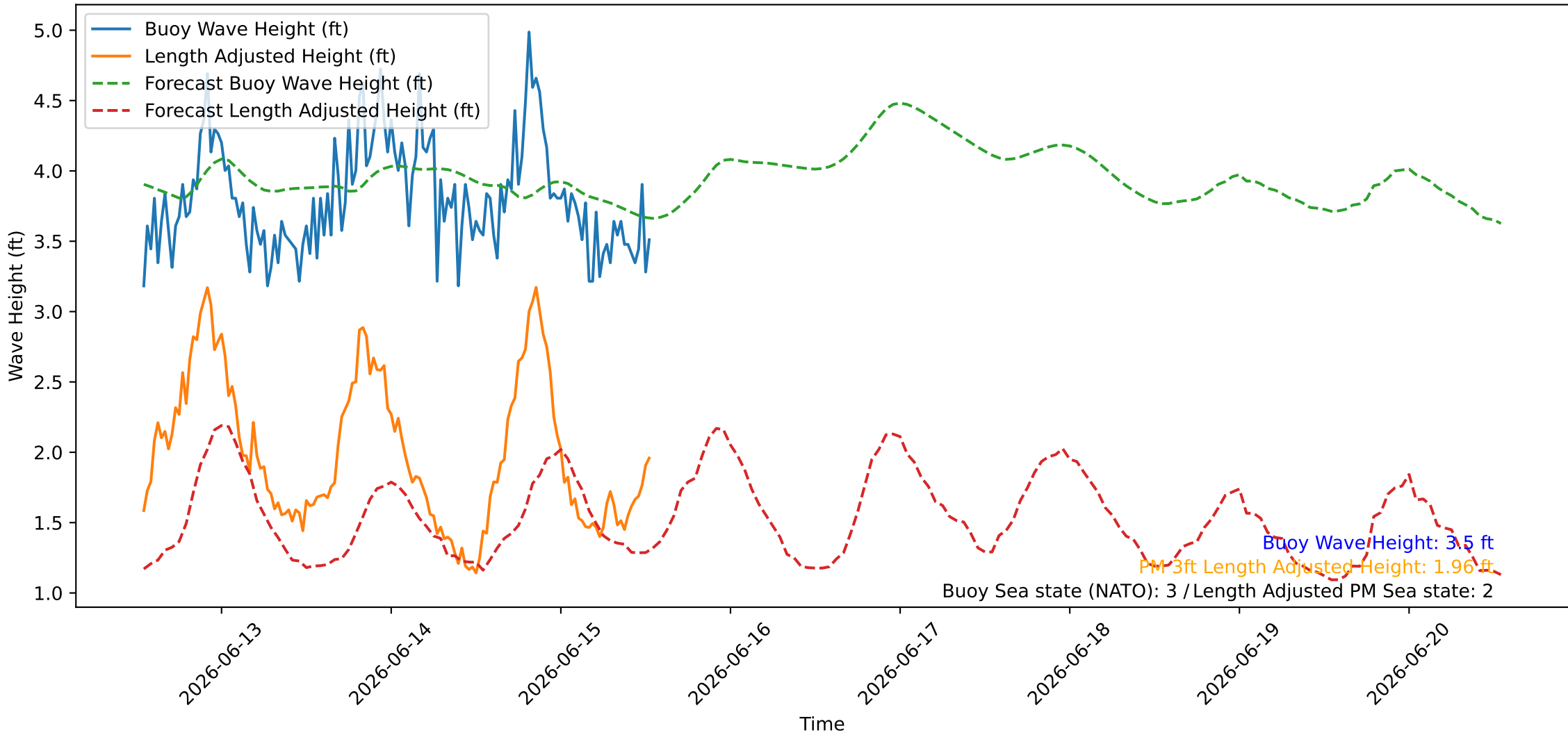
Wave Heights over Time for Oceanside Harbor at 2026-06-15 13:10:25
