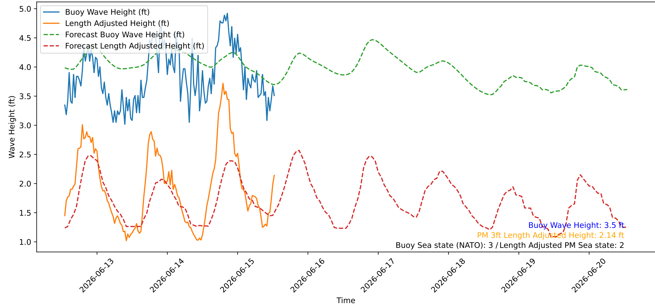
Wave Heights over Time for Green Beach at 2026-06-15 13:11:07
