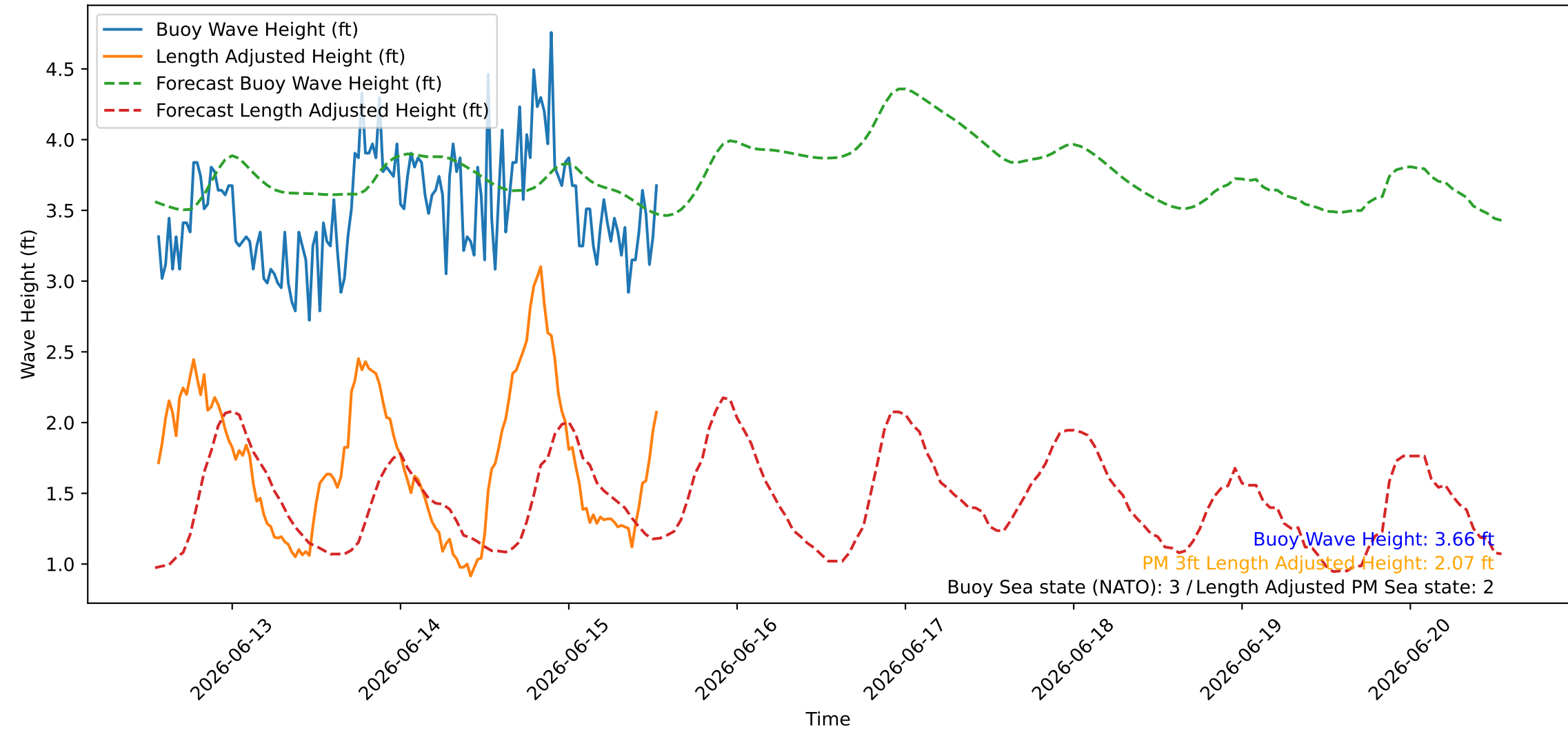
Wave Heights over Time for Red Beach at 2026-06-15 13:10:44
