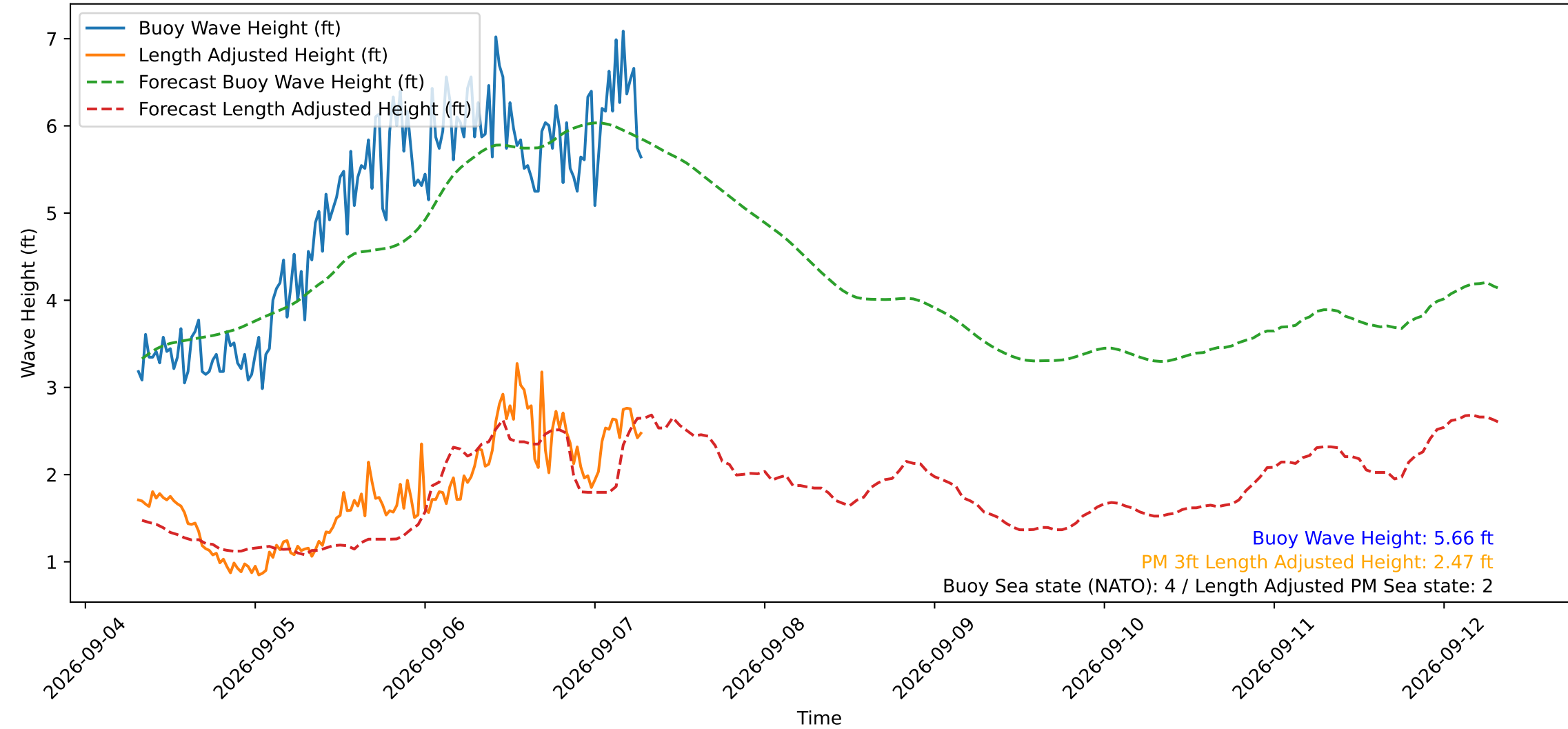
Wave Heights over Time for Oceanside Harbor at 2026-09-07 07:30:30
