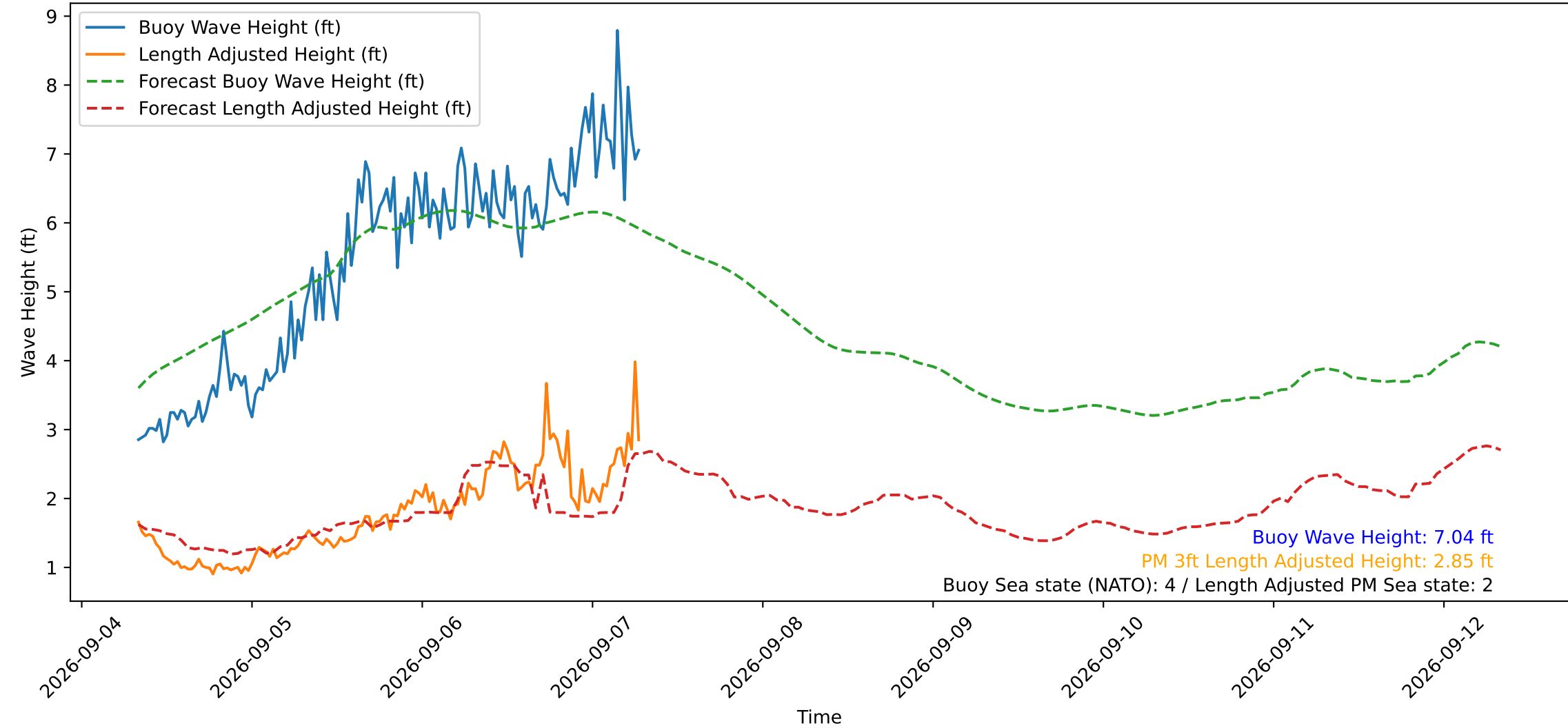
Wave Heights over Time for Green Beach at 2026-09-07 07:31:12
