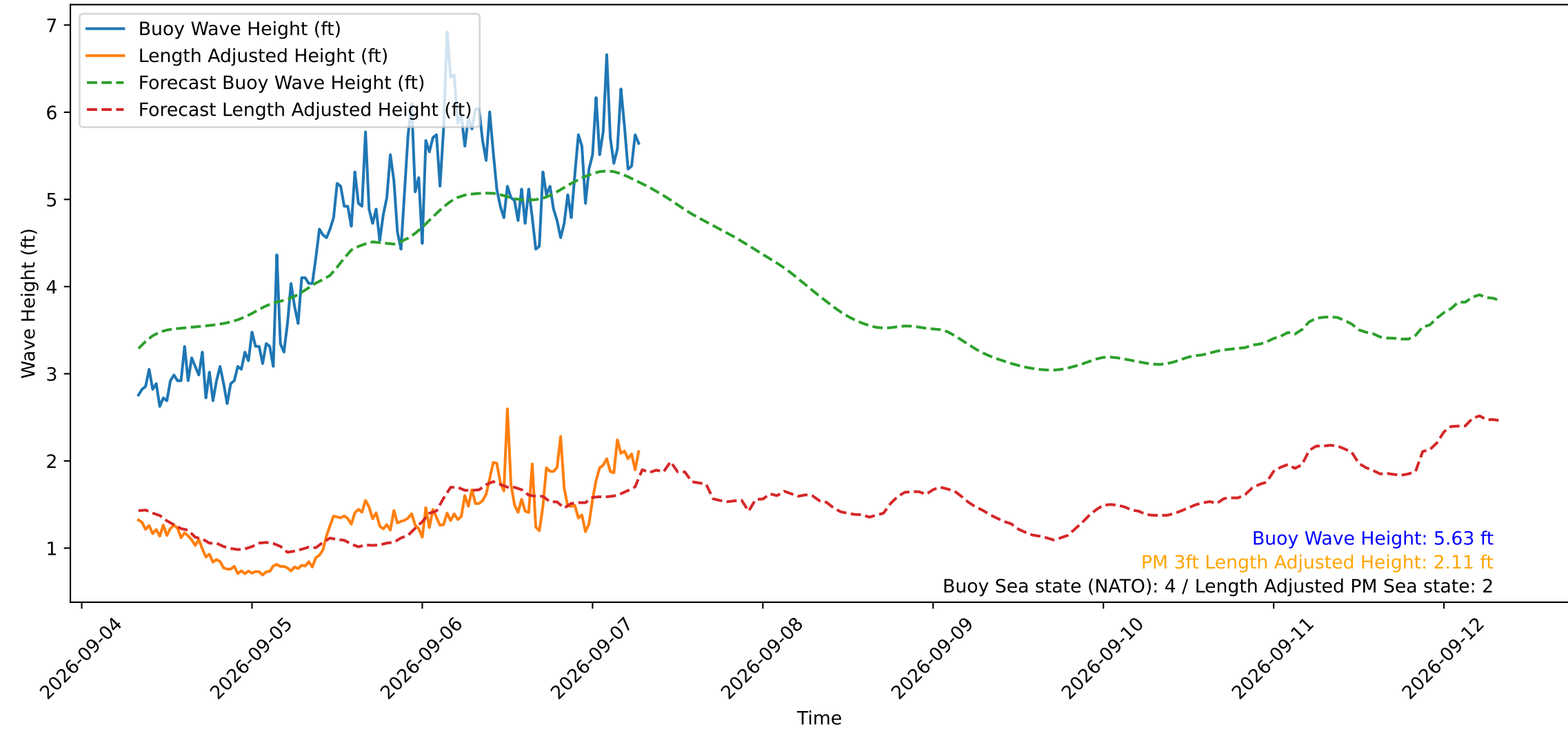
Wave Heights over Time for Red Beach at 2026-09-07 07:30:49
