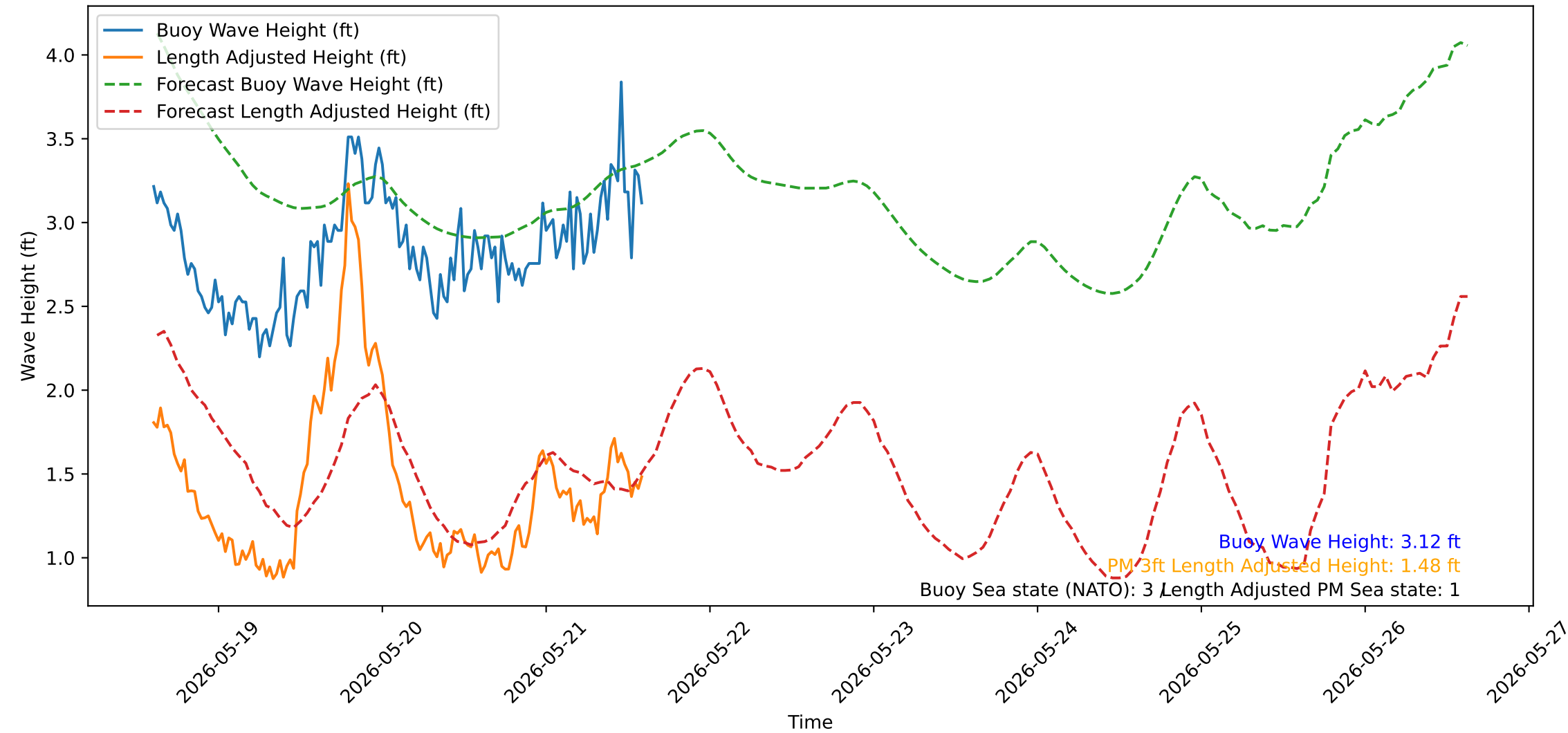
Wave Heights over Time for Oceanside Harbor at 2026-05-21 14:40:31
