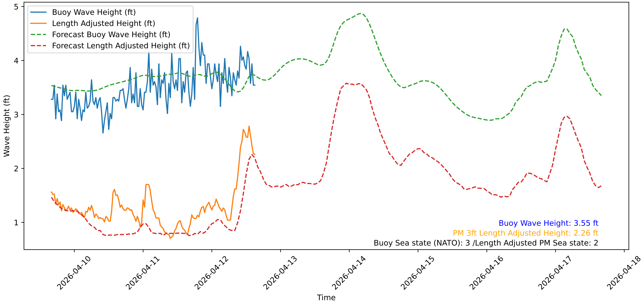
Wave Heights over Time for Oceanside Harbor at 2026-04-12 16:10:31
