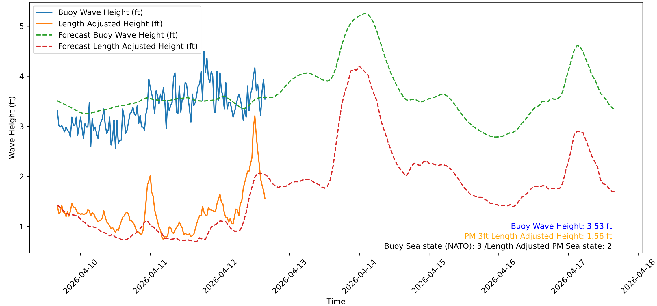
Wave Heights over Time for Green Beach at 2026-04-12 16:11:13
