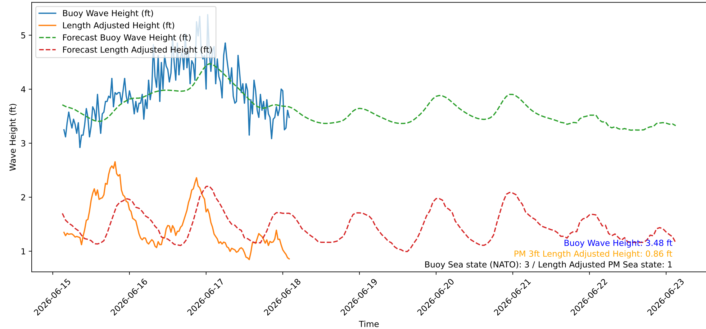
Wave Heights over Time for Red Beach at 2026-06-18 03:00:45
