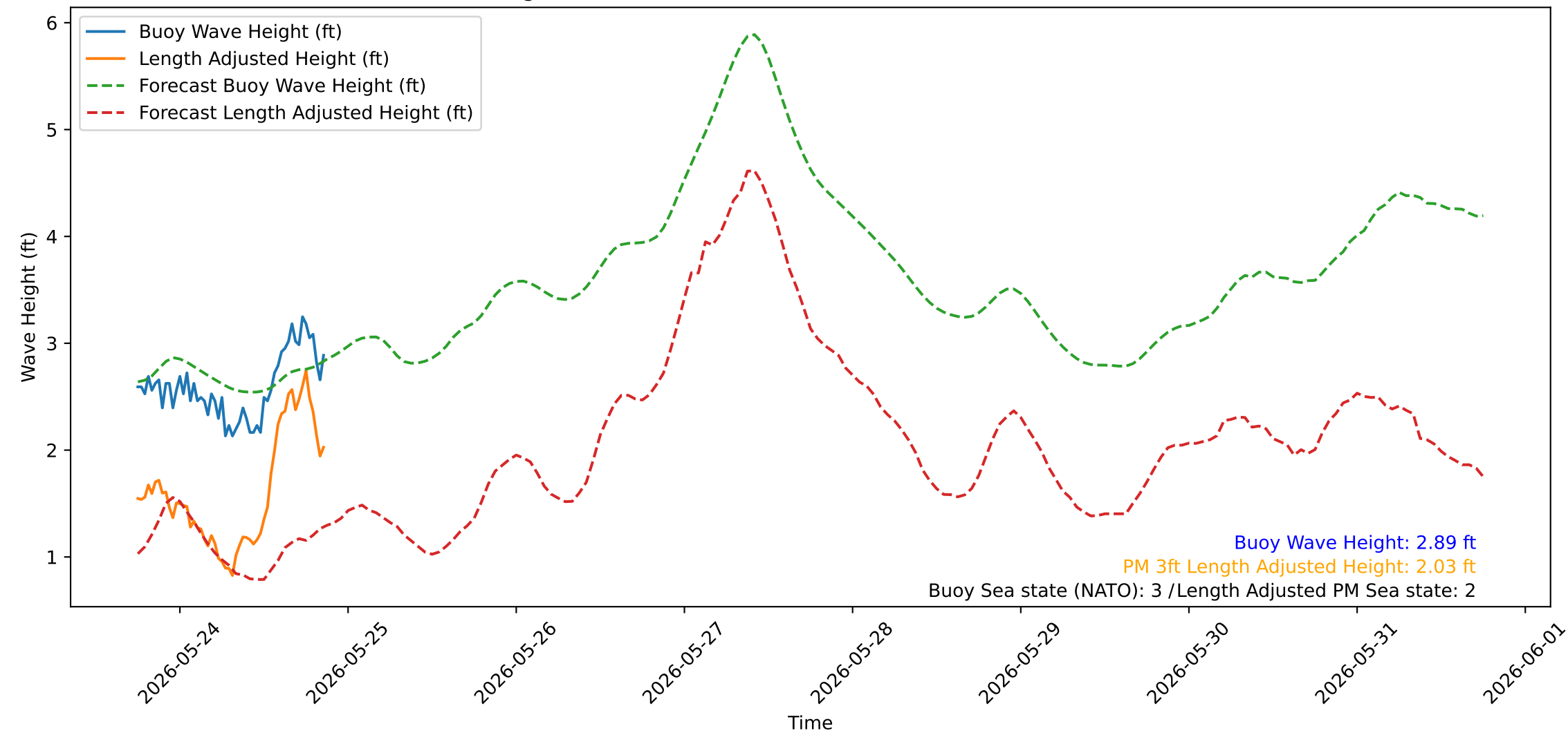
Wave Heights over Time for Oceanside Harbor at 2026-05-26 17:50:26
