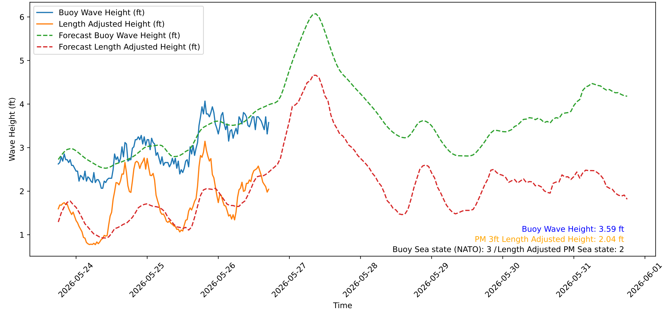
Wave Heights over Time for Green Beach at 2026-05-26 17:51:10
