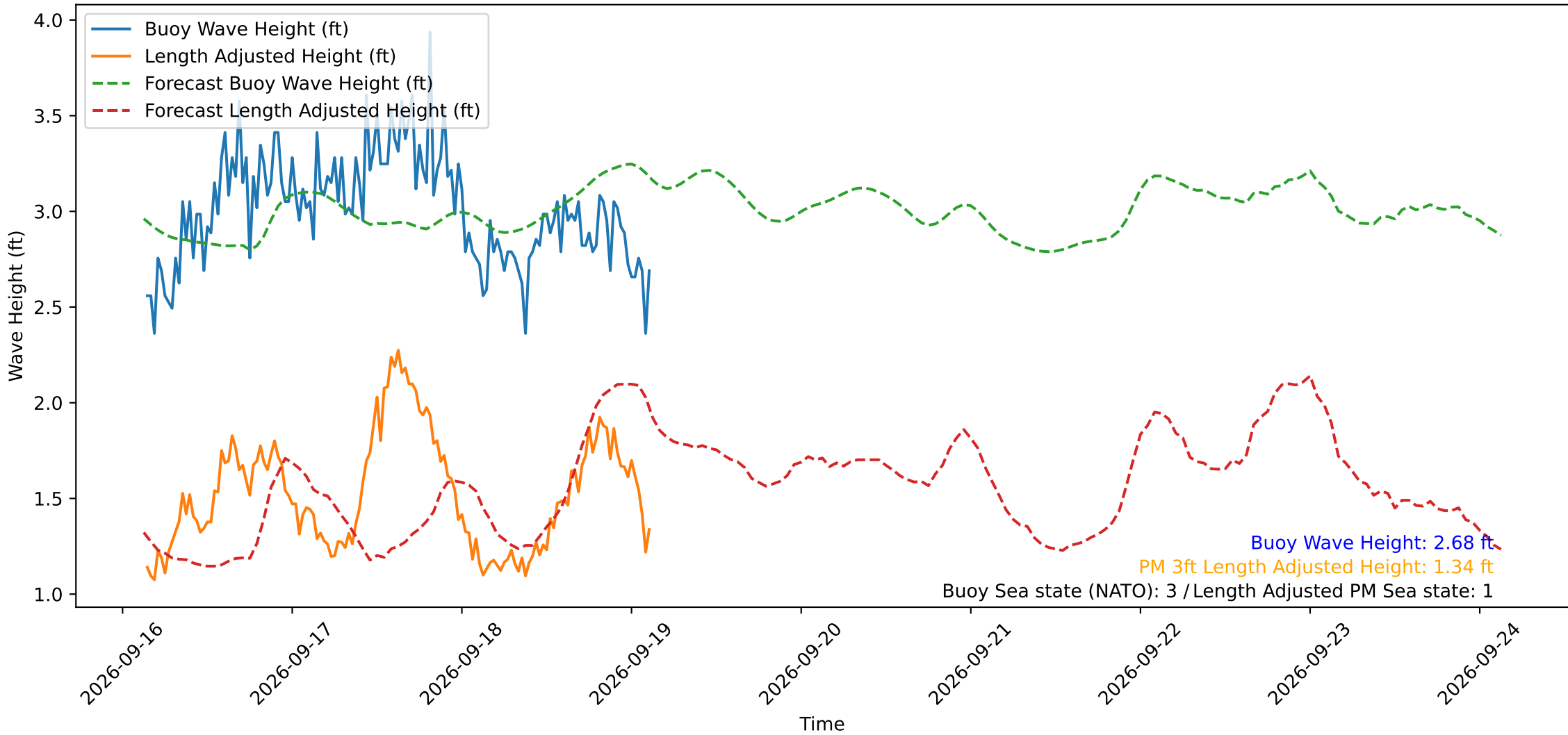
Wave Heights over Time for Oceanside Harbor at 2026-09-19 03:20:30
