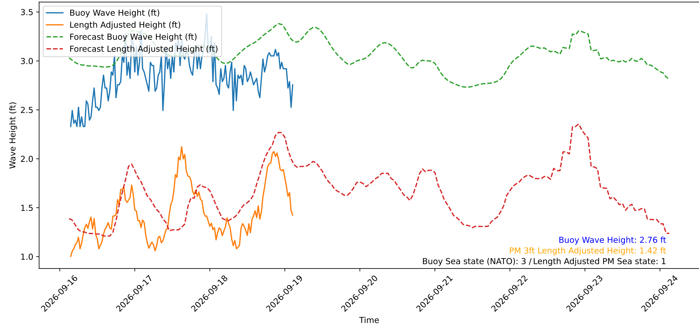
Wave Heights over Time for Green Beach at 2026-09-19 03:21:14
