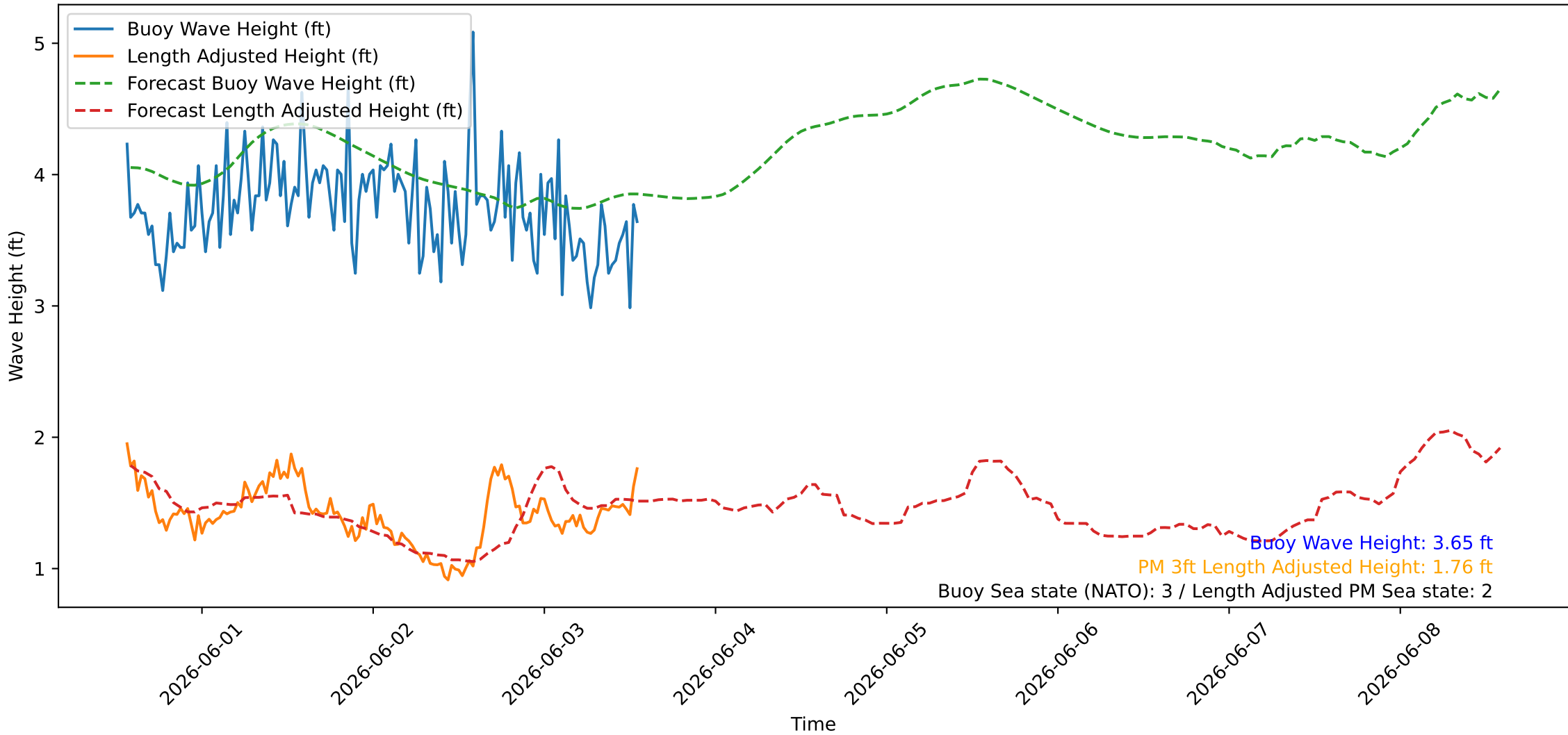
Wave Heights over Time for Oceanside Harbor at 2026-06-03 13:40:26
