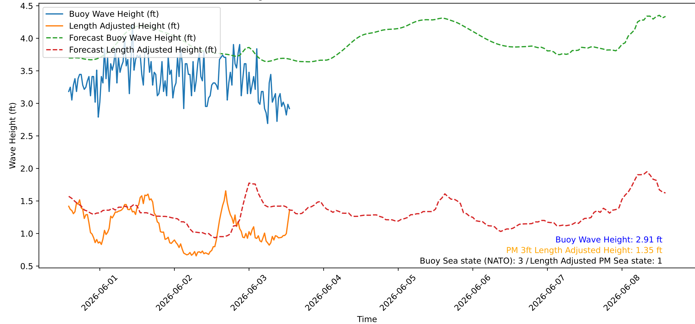
Wave Heights over Time for Red Beach at 2026-06-03 13:40:46
