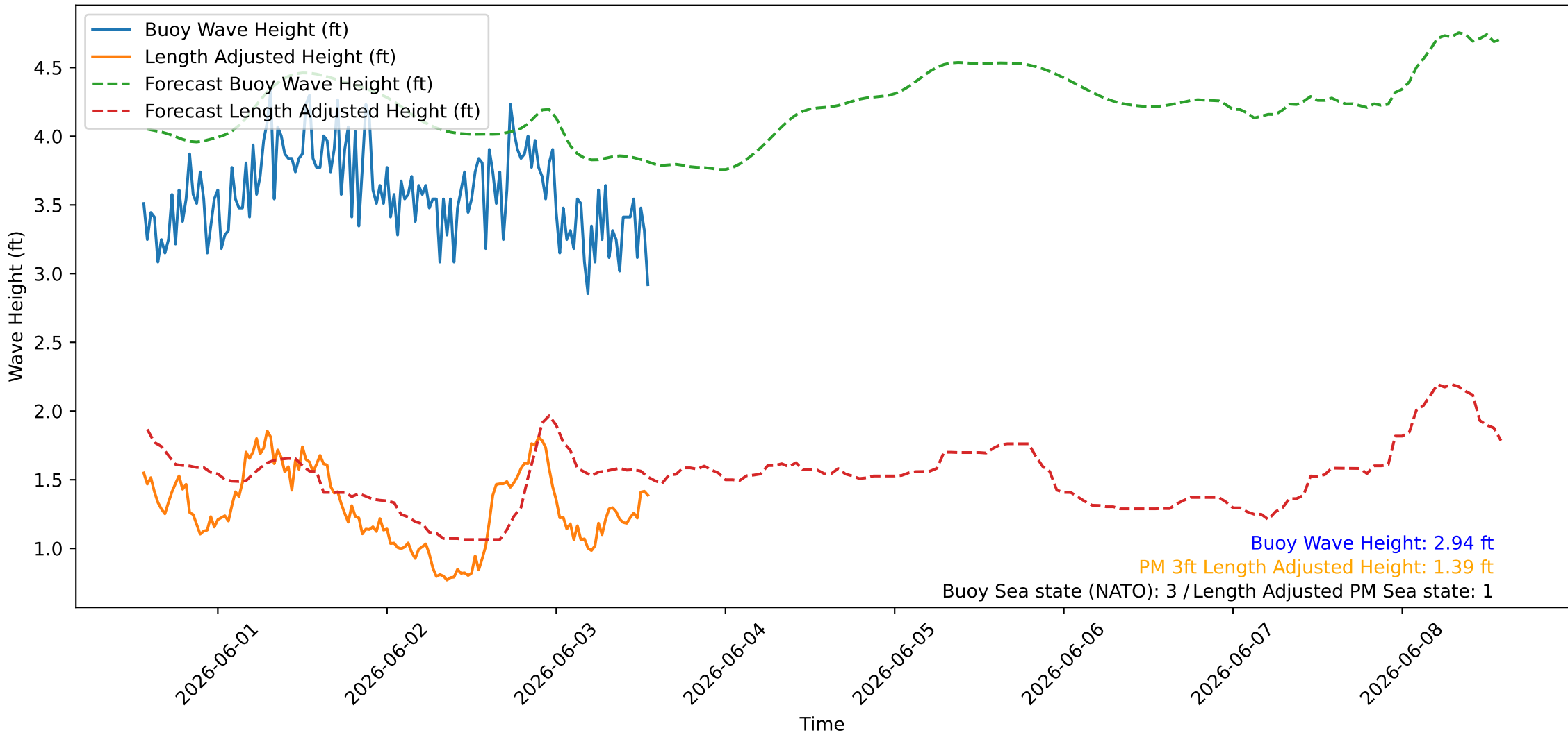
Wave Heights over Time for Green Beach at 2026-06-03 13:41:09
