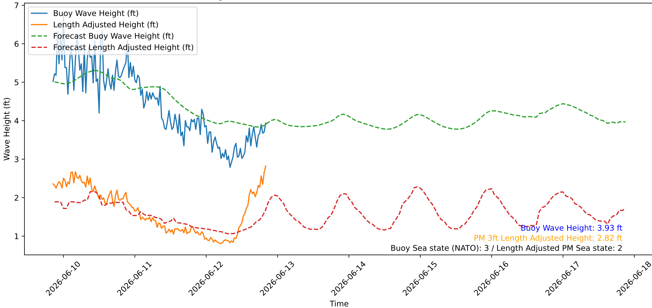
Wave Heights over Time for Oceanside Harbor at 2026-06-12 20:40:26
