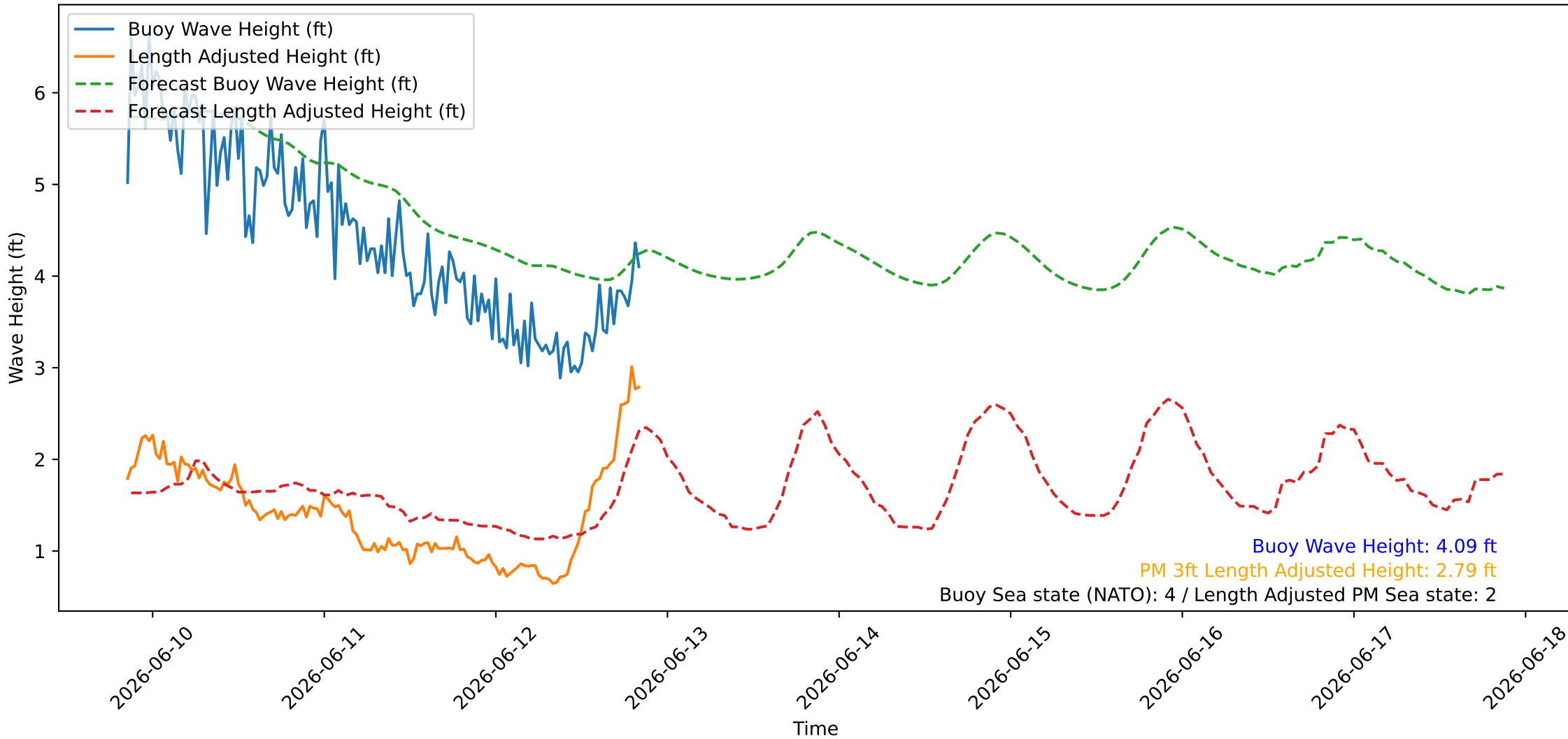
Wave Heights over Time for Green Beach at 2026-06-12 20:41:08
