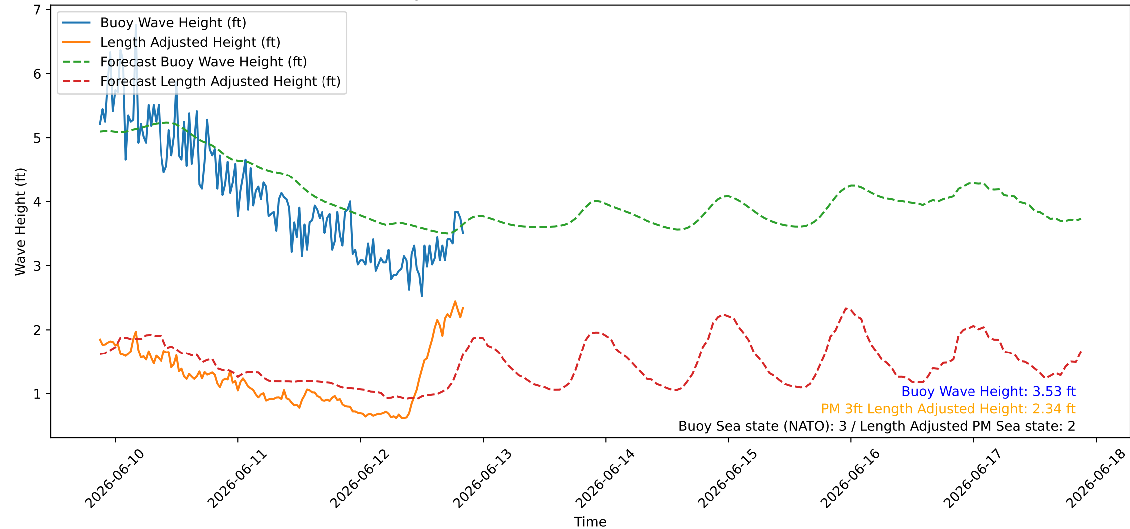
Wave Heights over Time for Red Beach at 2026-06-12 20:40:45
