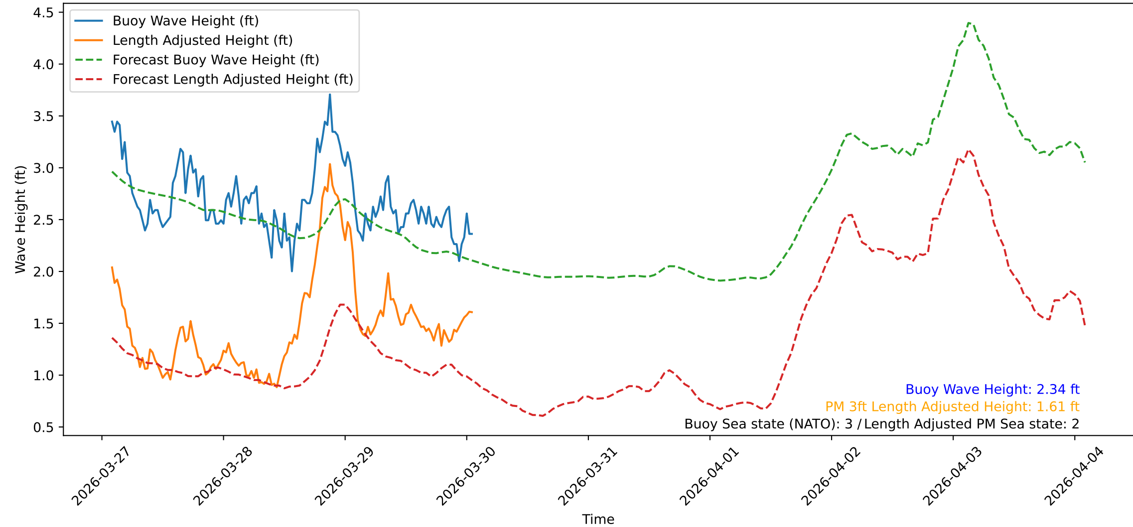
Wave Heights over Time for Green Beach at 2026-03-30 01:51:09
