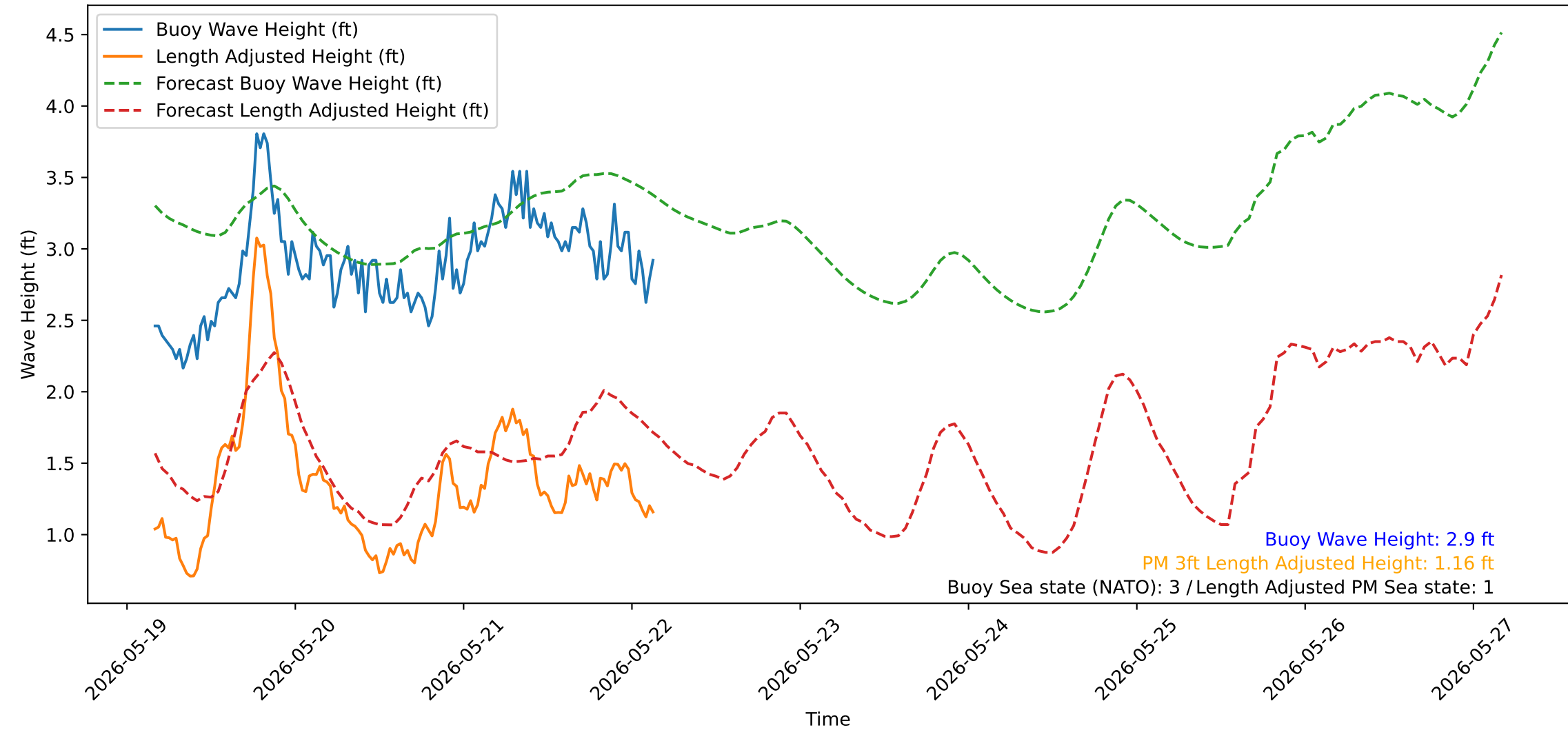
Wave Heights over Time for Green Beach at 2026-05-22 04:01:14
