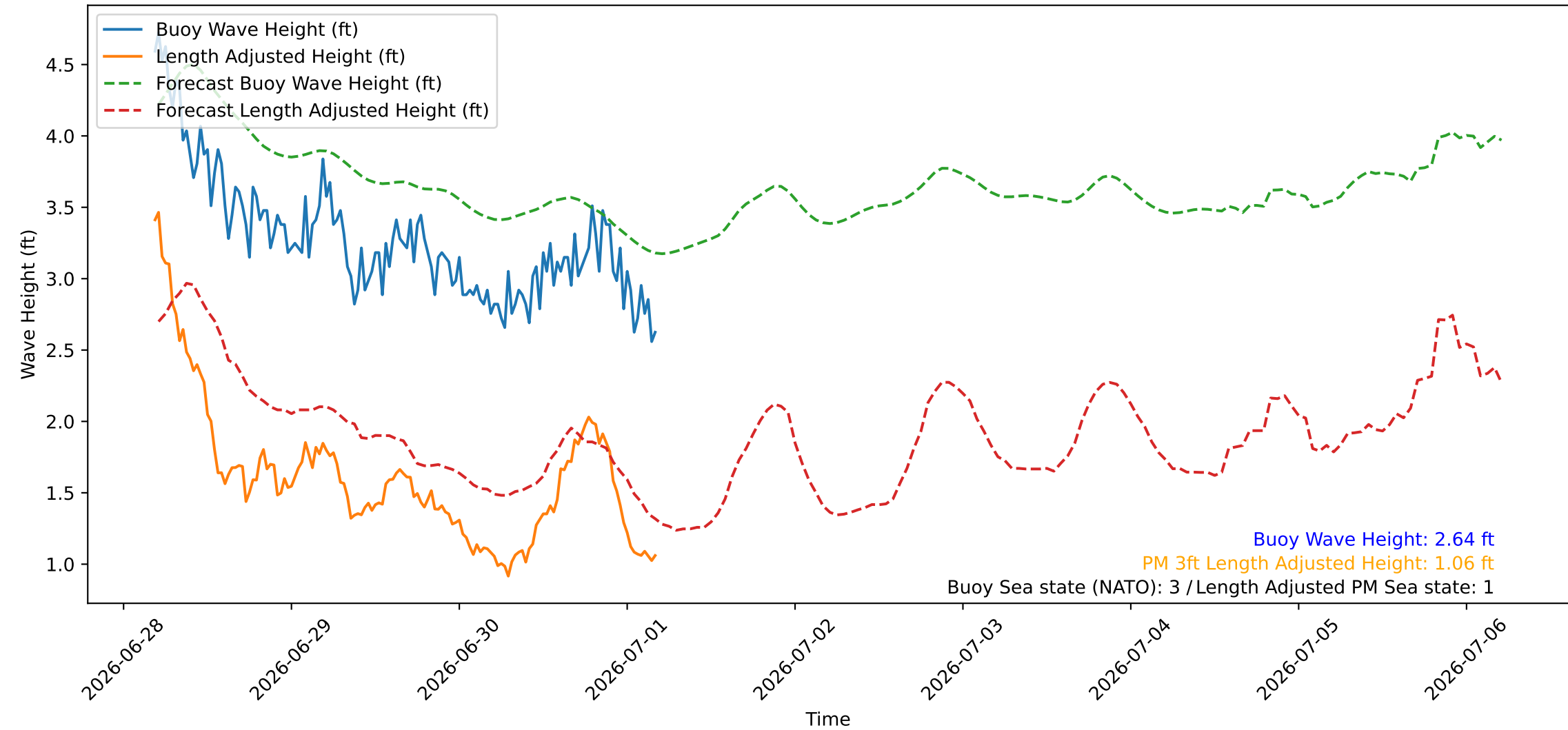
Wave Heights over Time for Green Beach at 2026-07-01 04:41:08
