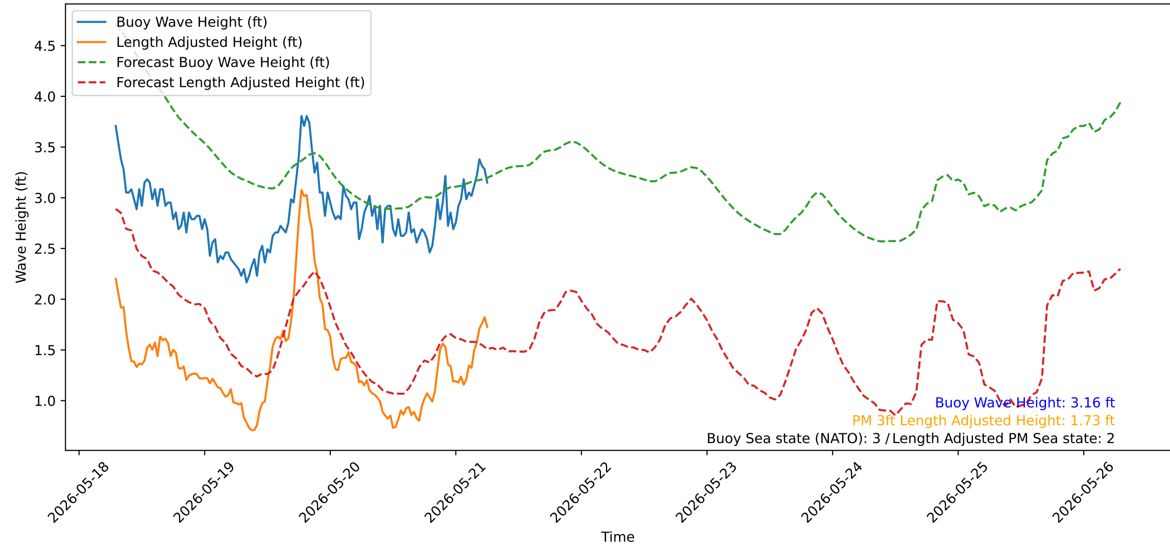
Wave Heights over Time for Green Beach at 2026-05-21 06:51:14
