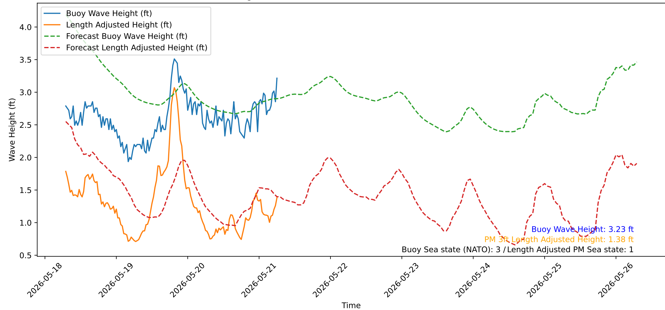
Wave Heights over Time for Red Beach at 2026-05-21 06:50:52
