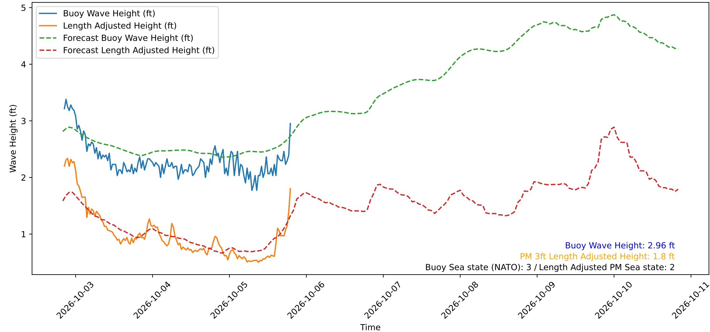
Wave Heights over Time for Green Beach at 2026-10-05 20:01:13
