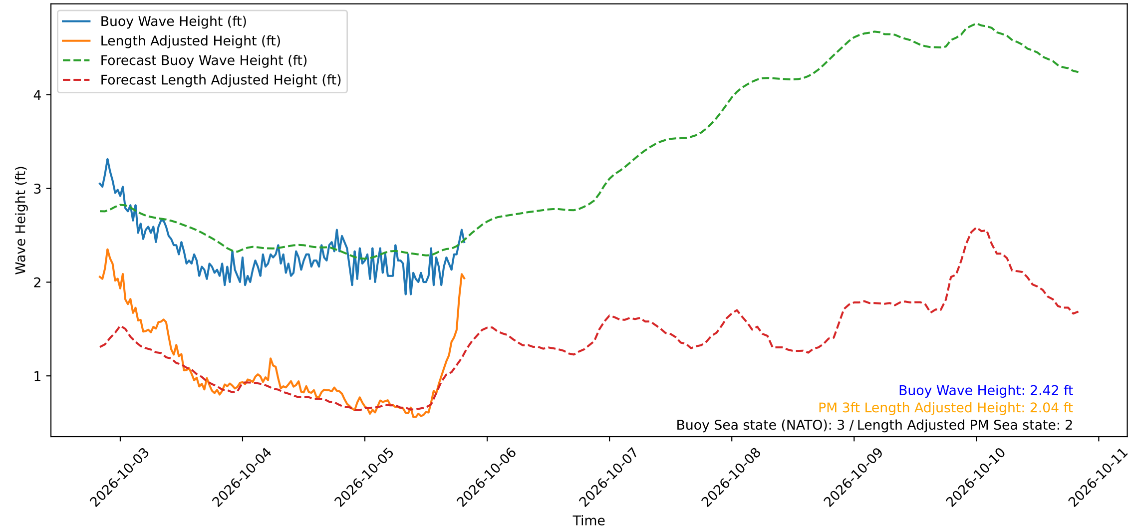
Wave Heights over Time for Oceanside Harbor at 2026-10-05 20:00:30
