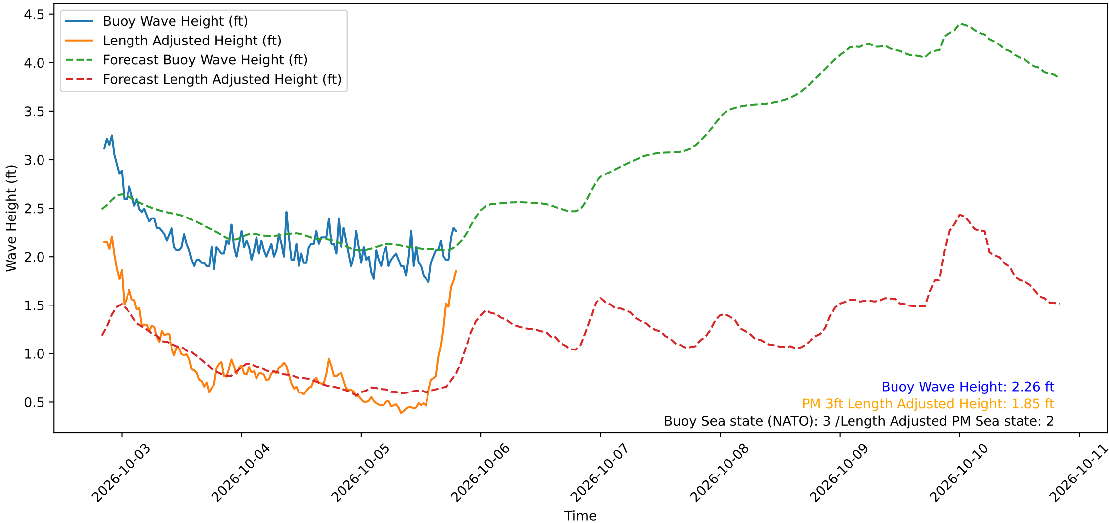
Wave Heights over Time for Red Beach at 2026-10-05 20:00:50
